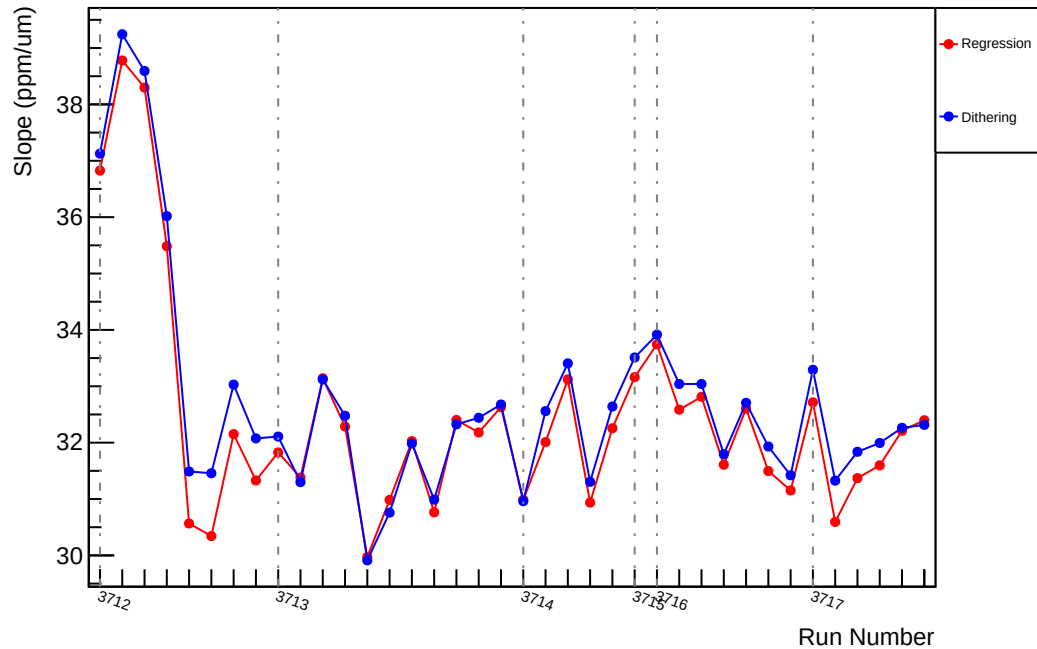
Slug19: Slope : usl_vs_evMon0 (ppm/um)
