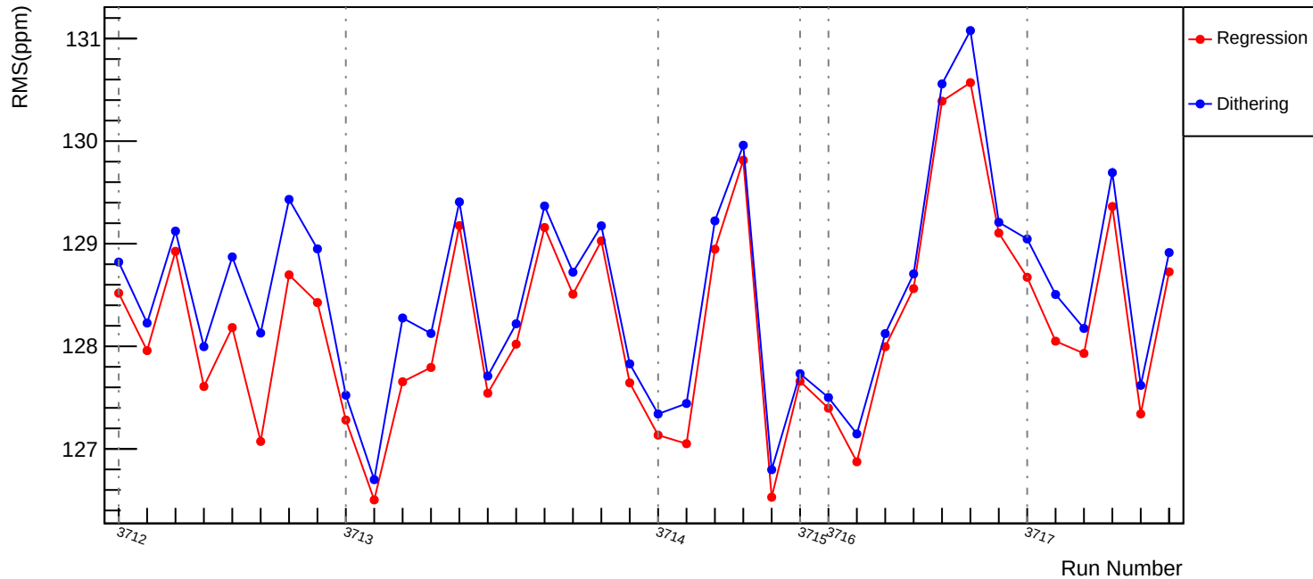
Slug19: Corrected RMS (ppm): asym_usl
