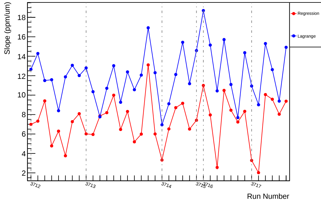
Slug19: Slope : usl_vs_evMon8 (ppm/um)
