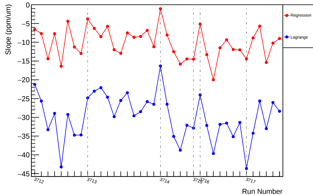
Slug19: Slope : usl_vs_evMon11 (ppm/um)
