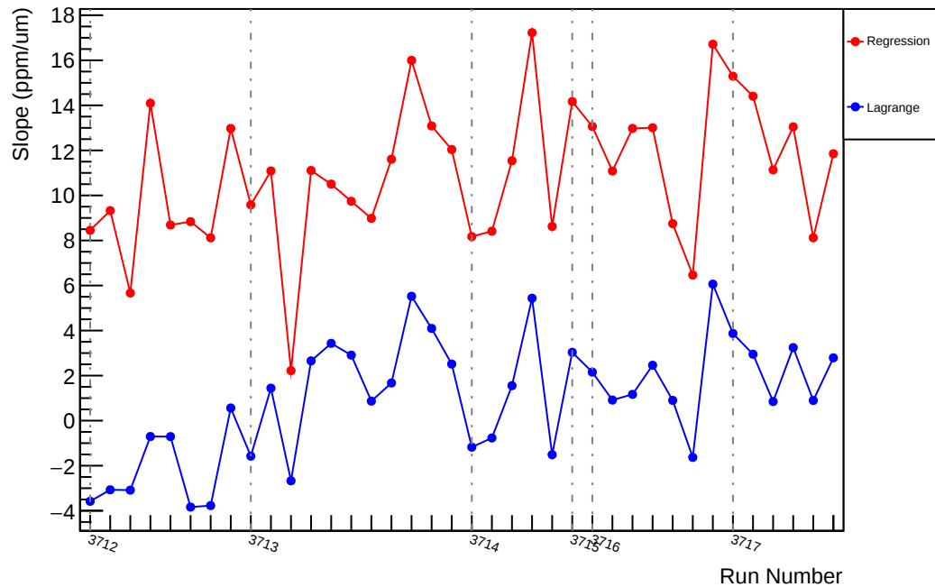
Slug19: Slope : usl_vs_evMon7 (ppm/um)
