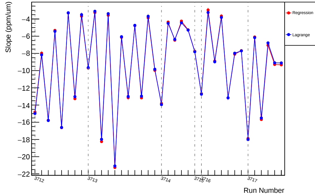
Slug19: Slope : usl_vs_evMon1 (ppm/um)
