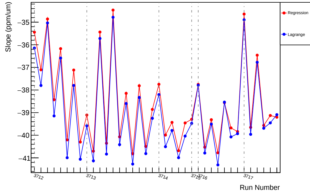
Slug19: Slope : usl_vs_evMon2 (ppm/um)
