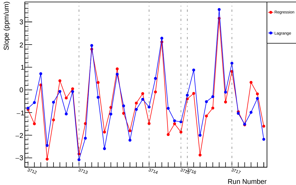
Slug19: Slope : usl_vs_evMon5 (ppm/um)
