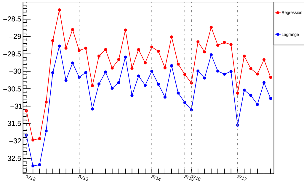
Slug19: Slope : usl_vs_evMon0 (ppm/um)
