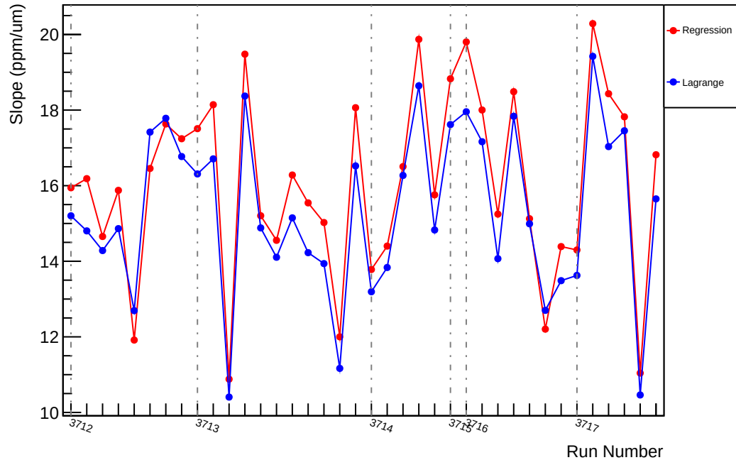
Slug19: Slope : usr_vs_evMon6 (ppm/um)
