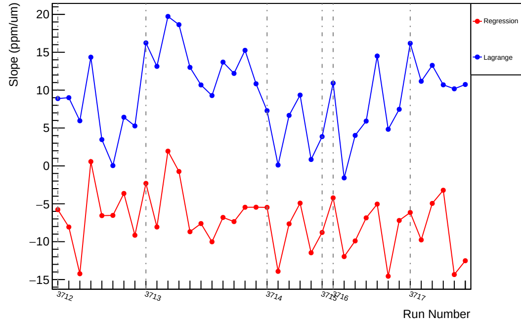
Slug19: Slope : usr_vs_evMon11 (ppm/um)
