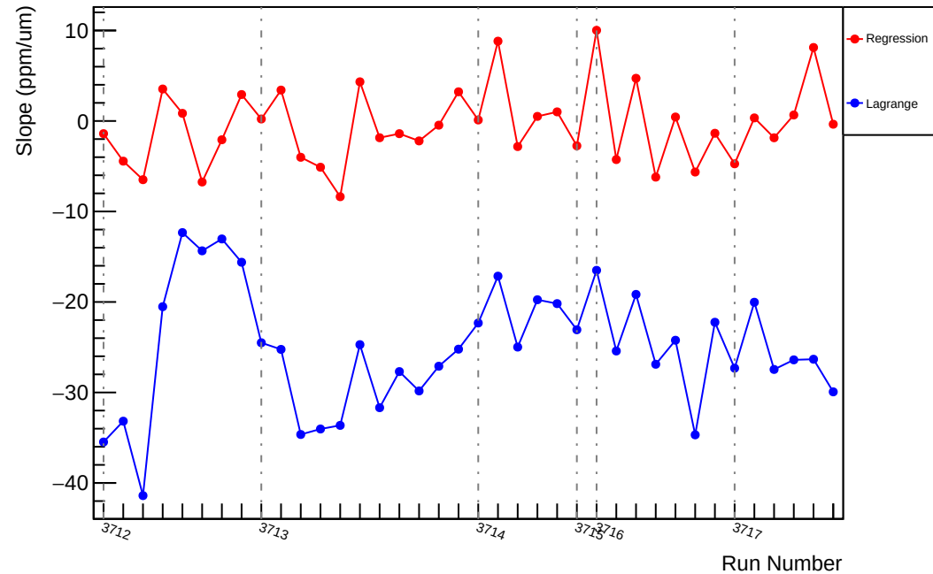
Slug19: Slope : usr_vs_evMon10 (ppm/um)
