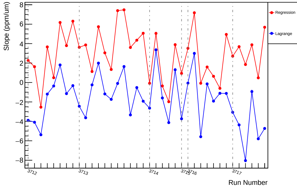
Slug19: Slope : usr_vs_evMon8 (ppm/um)
