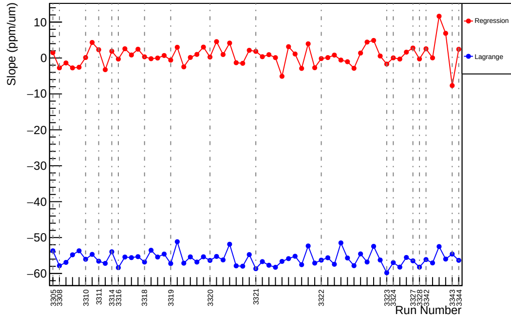
Slug1: Slope : us_avg_vs_evMon7 (ppm/um)
