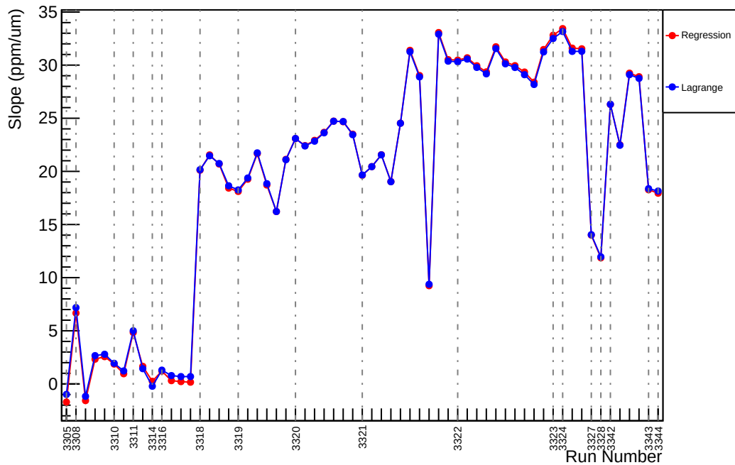
Slug1: Slope : us_avg_vs_evMon0 (ppm/um)
