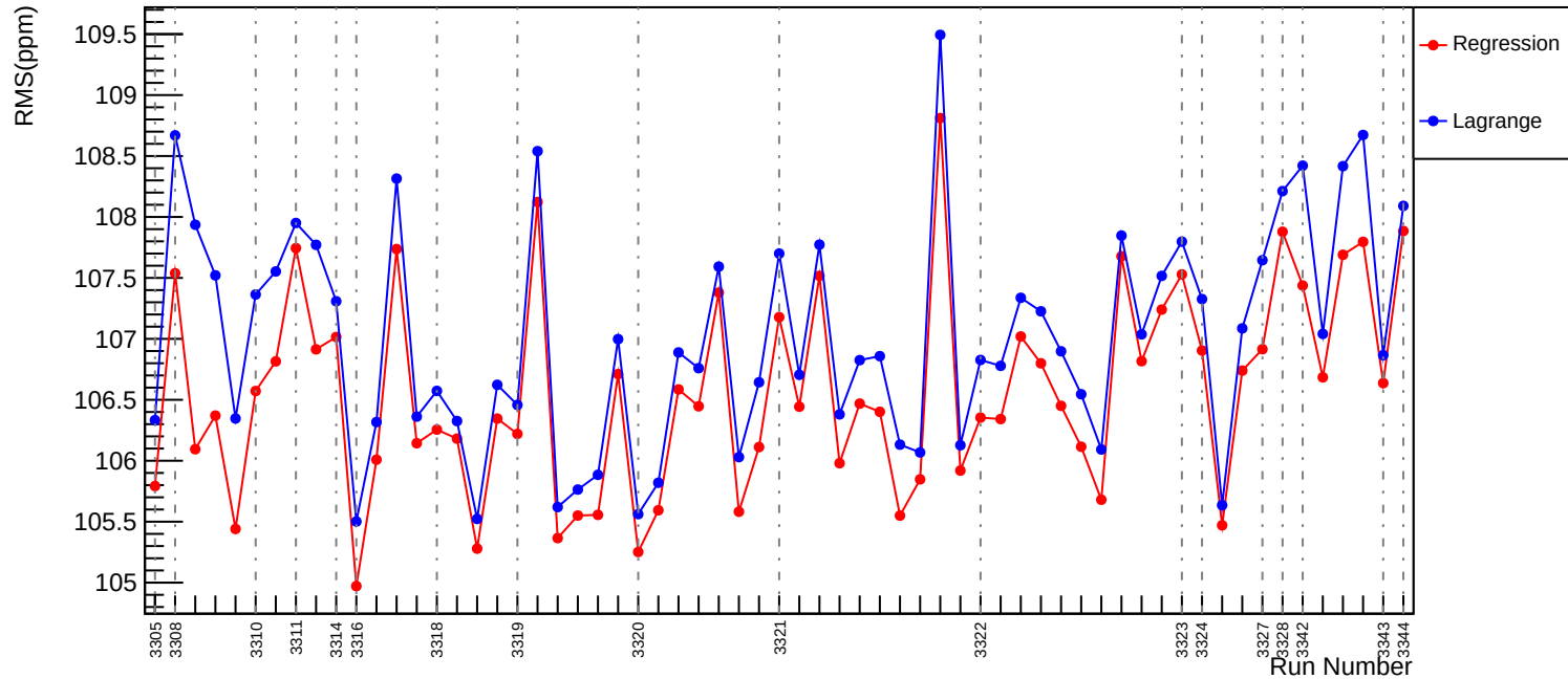
Slug1: Corrected RMS (ppm): asym_us_dd
