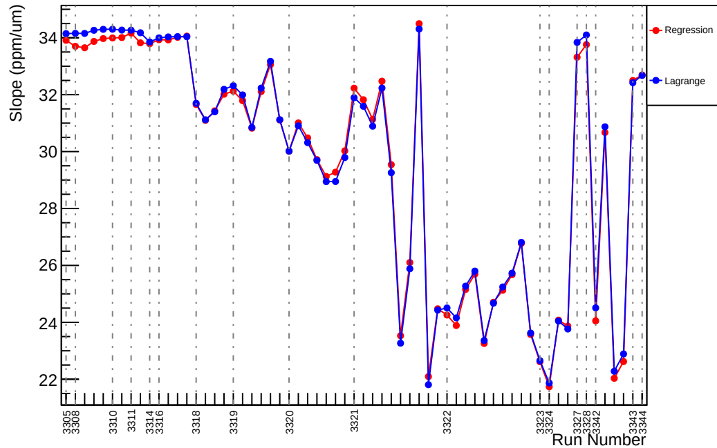
Slug1: Slope : us_dd_vs_evMon0 (ppm/um)
