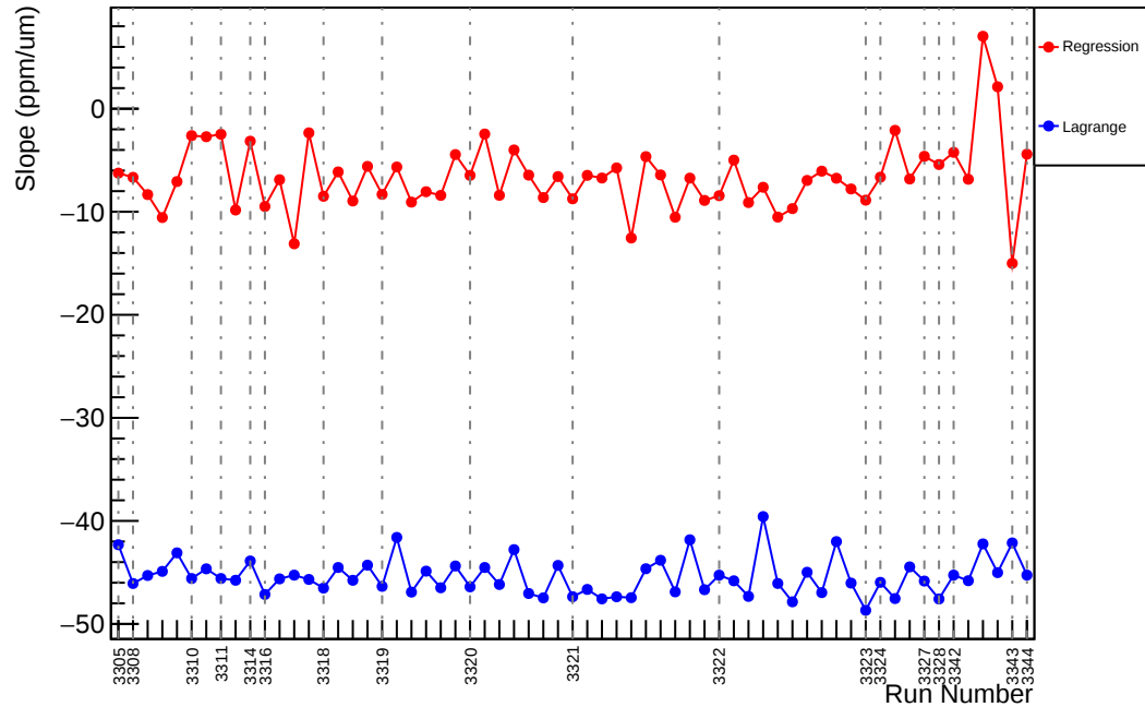
Slug1: Slope : usl_vs_evMon7 (ppm/um)
