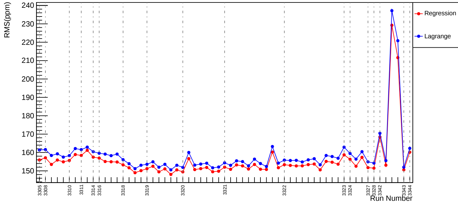
Slug1: Corrected RMS (ppm): asym_usl
