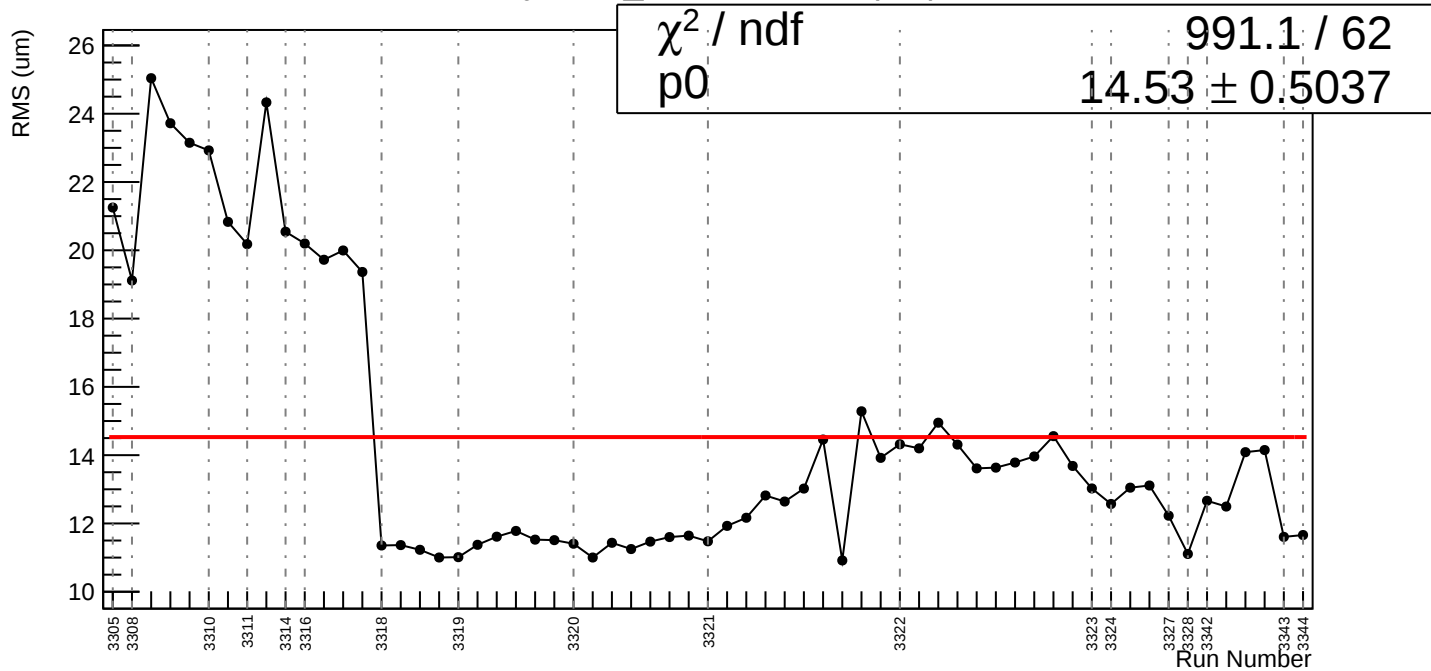
Slug1: diff_evMon1 RMS (um)
