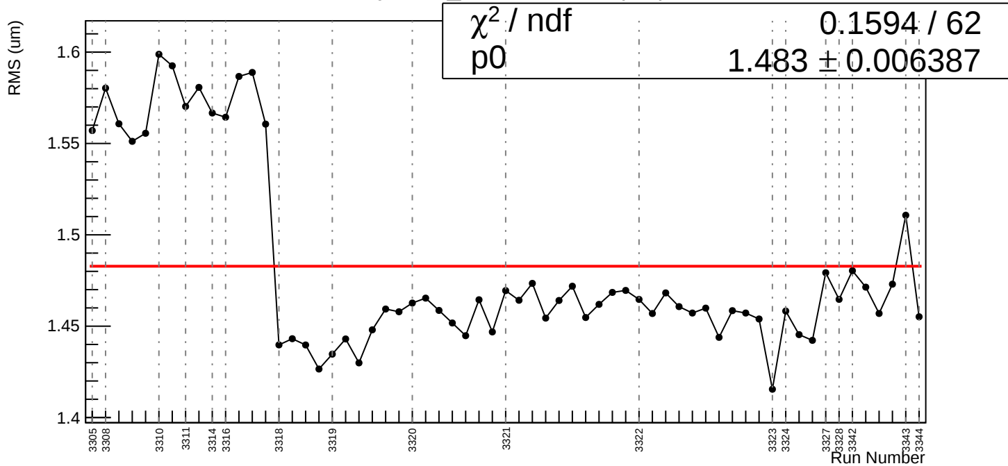
Slug1: diff_evMon5 RMS (um)
