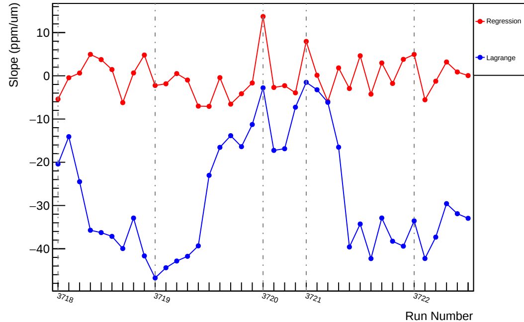
Slug20: Slope : usr_vs_evMon10 (ppm/um)
