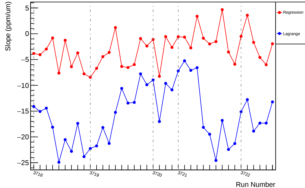
Slug20: Slope : usr_vs_evMon9 (ppm/um)
