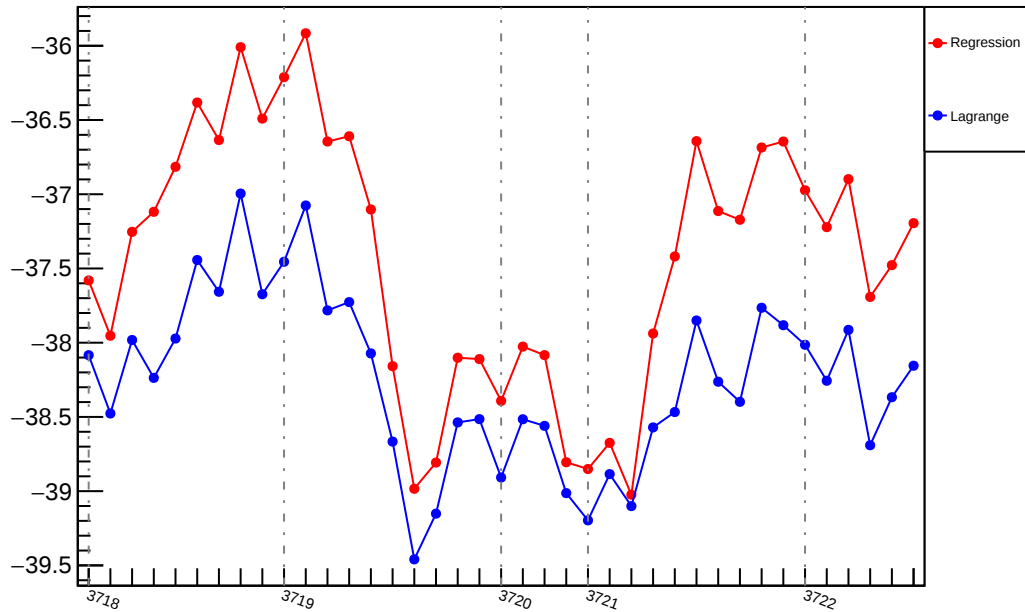
Slug20: Slope : usr_vs_evMon0 (ppm/um)
