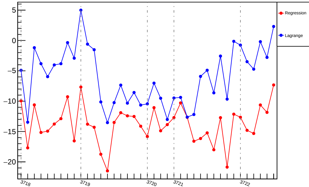
Slug20: Slope : usr_vs_evMon7 (ppm/um)
