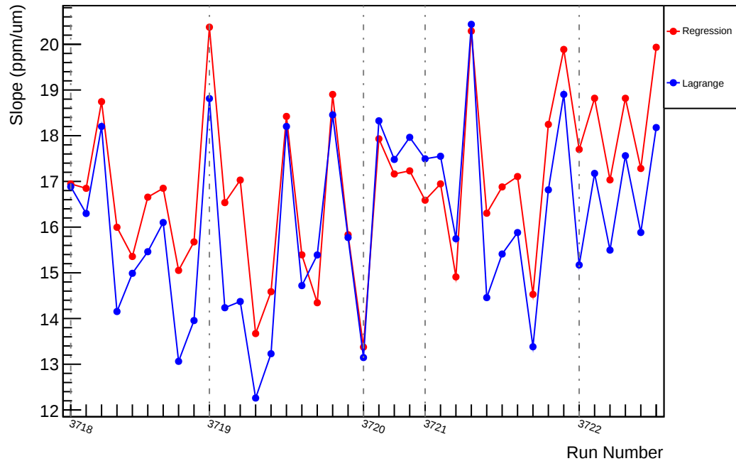
Slug20: Slope : usr_vs_evMon6 (ppm/um)
