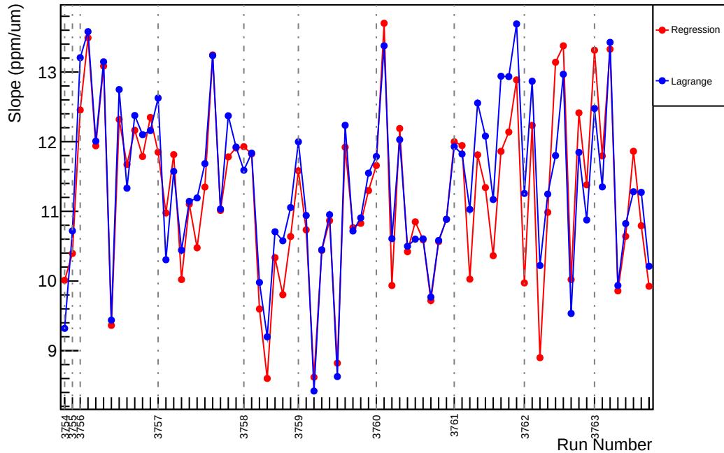
Slug21: Slope : us_avg_vs_evMon6 (ppm/um)
