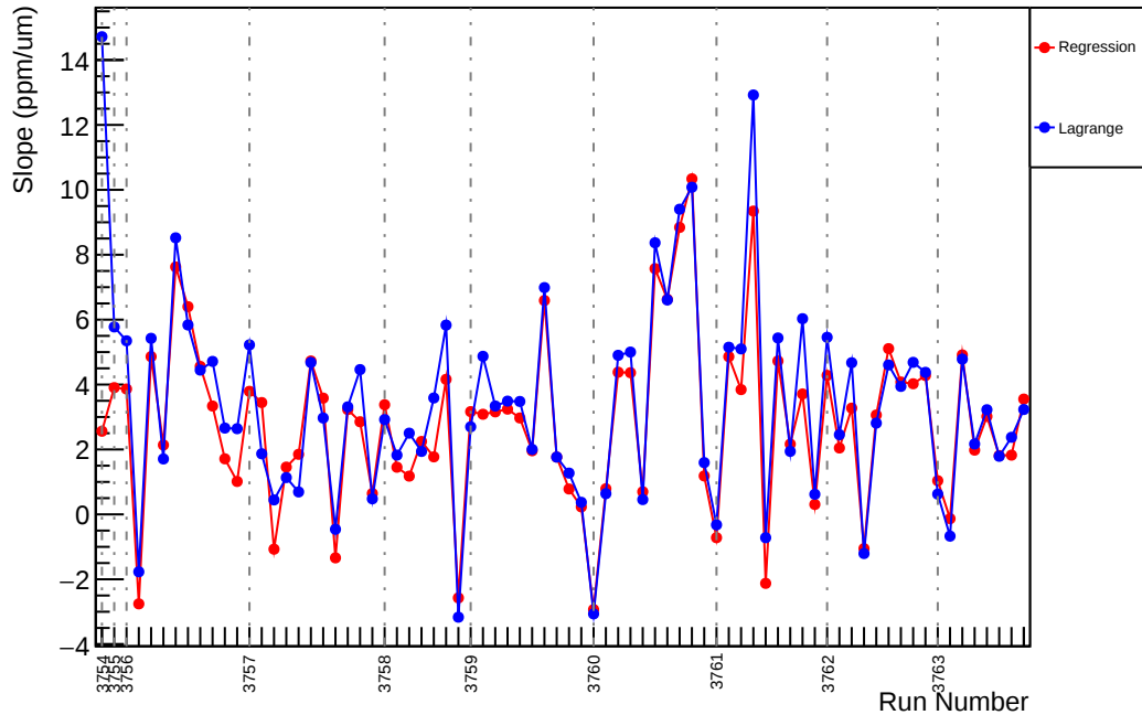
Slug21: Slope : us_avg_vs_evMon10 (ppm/um)
