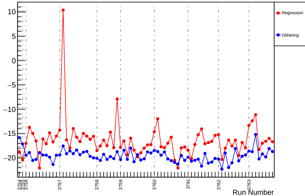
Slug21: Slope : usl_vs_evMon4 (ppm/um)
