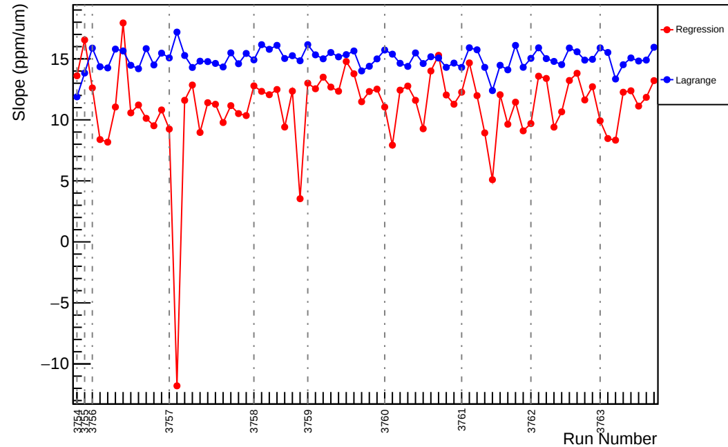
Slug21: Slope : usl_vs_evMon4 (ppm/um)
