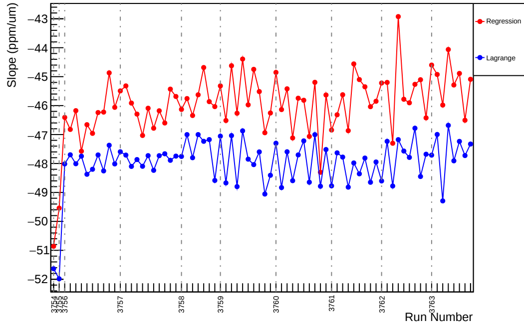
Slug21: Slope : usl_vs_evMon3 (ppm/um)
