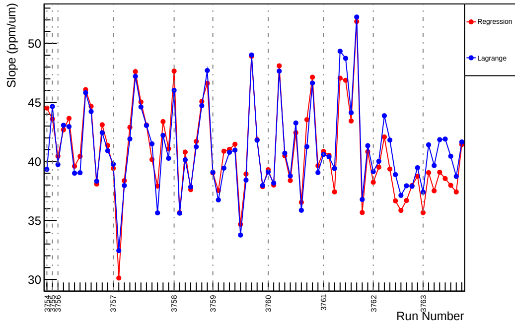
Slug21: Slope : usl_vs_evMon5 (ppm/um)
