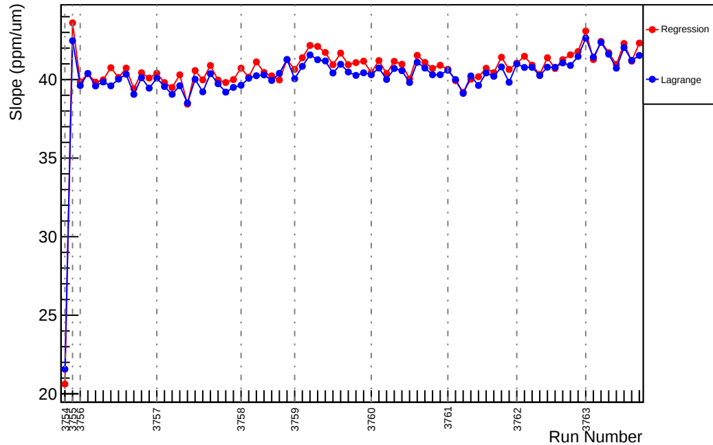
Slug21: Slope : usl_vs_evMon2 (ppm/um)
