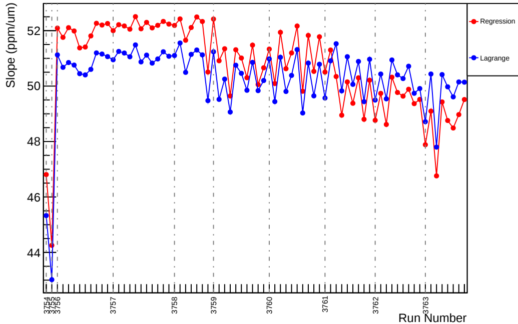
Slug21: Slope : usl_vs_evMon0 (ppm/um)
