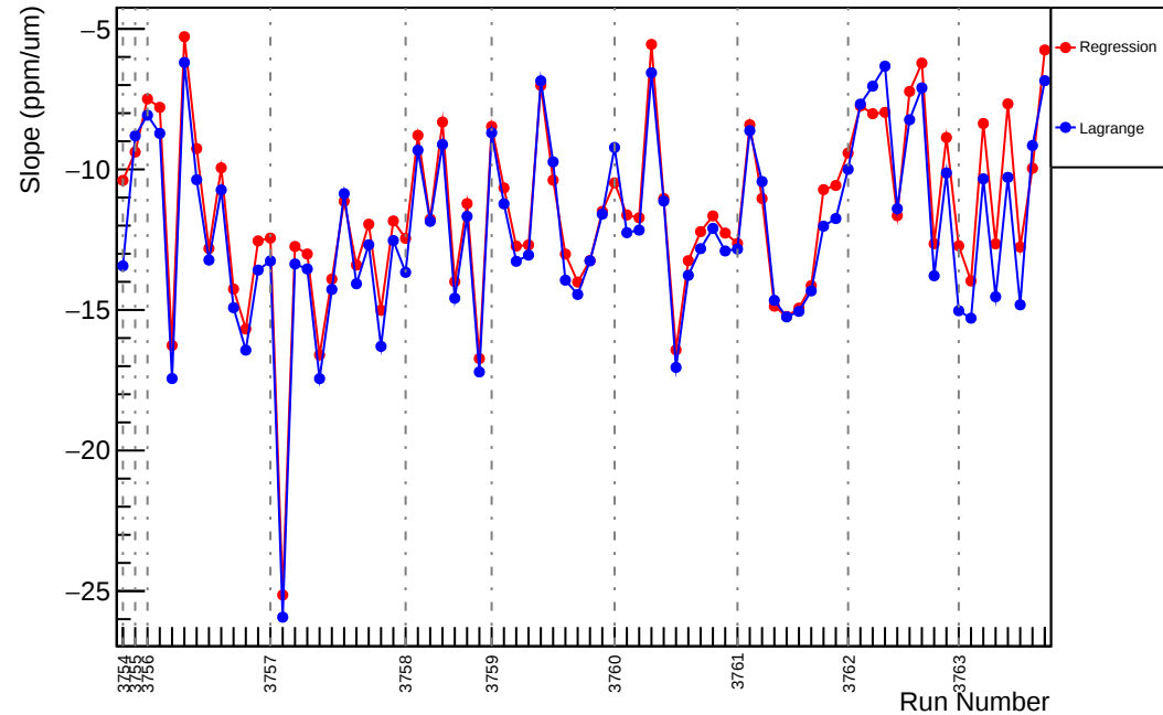
Slug21: Slope : usr_vs_evMon7 (ppm/um)
