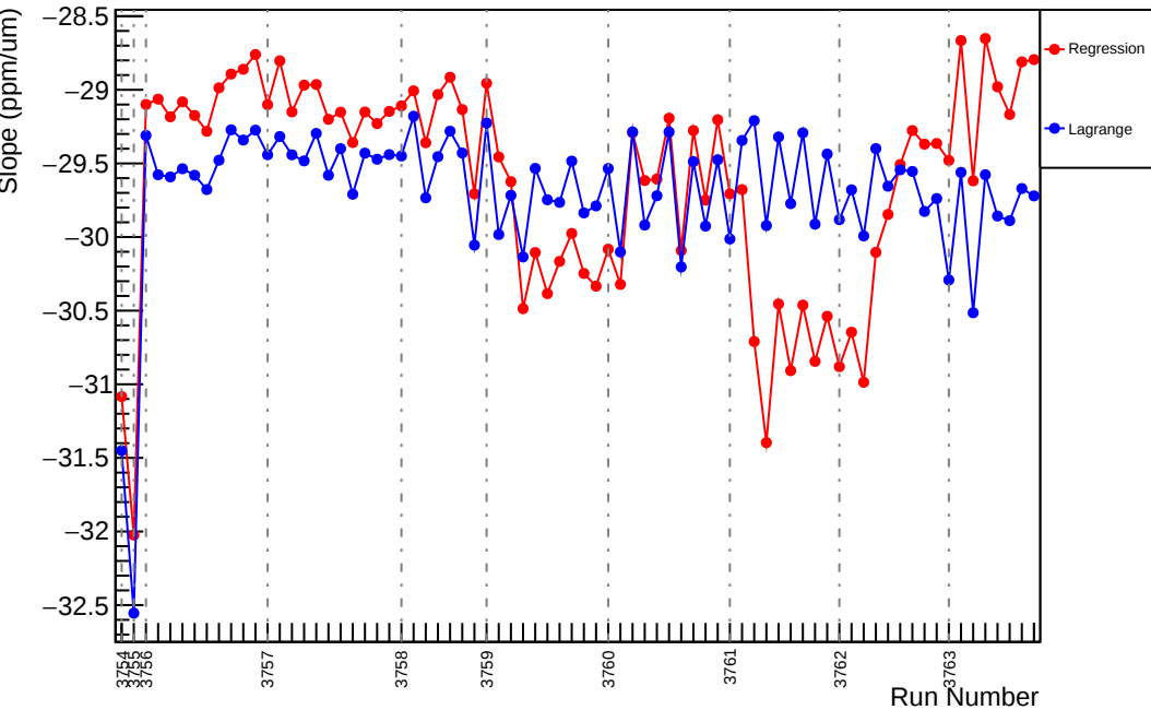
Slug21: Slope : usr_vs_evMon0 (ppm/um)
