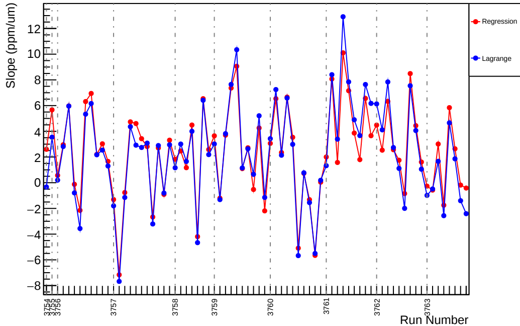
Slug21: Slope : usr_vs_evMon9 (ppm/um)
