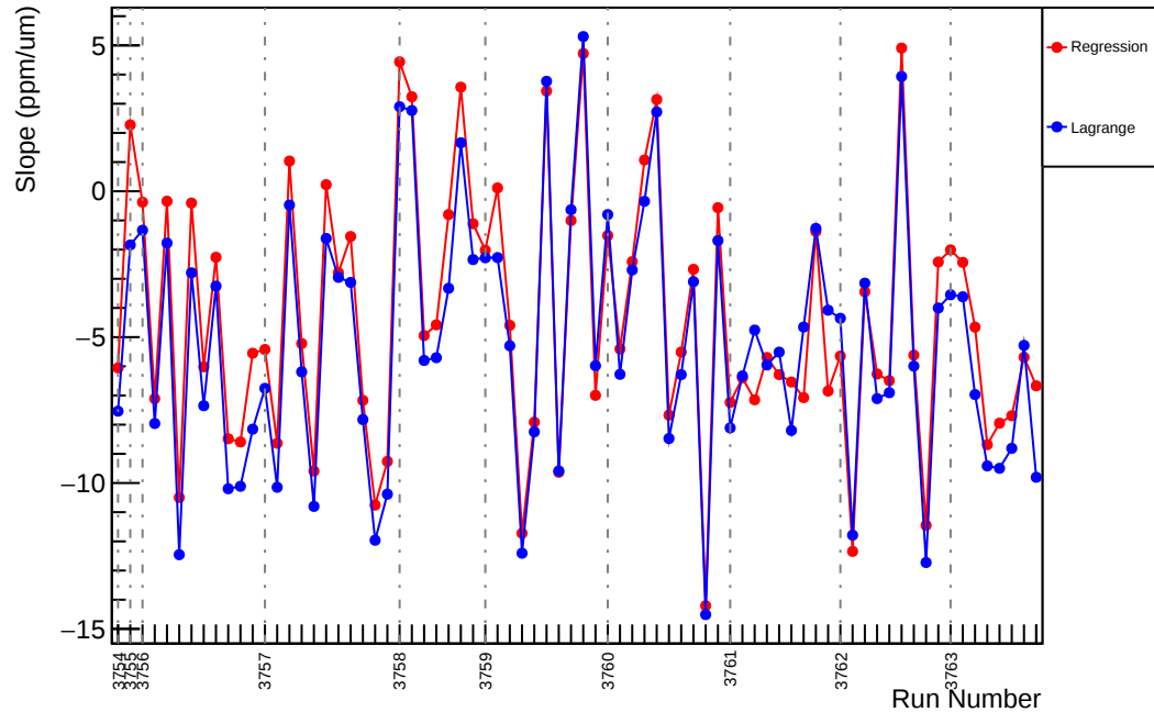
Slug21: Slope : usr_vs_evMon11 (ppm/um)
