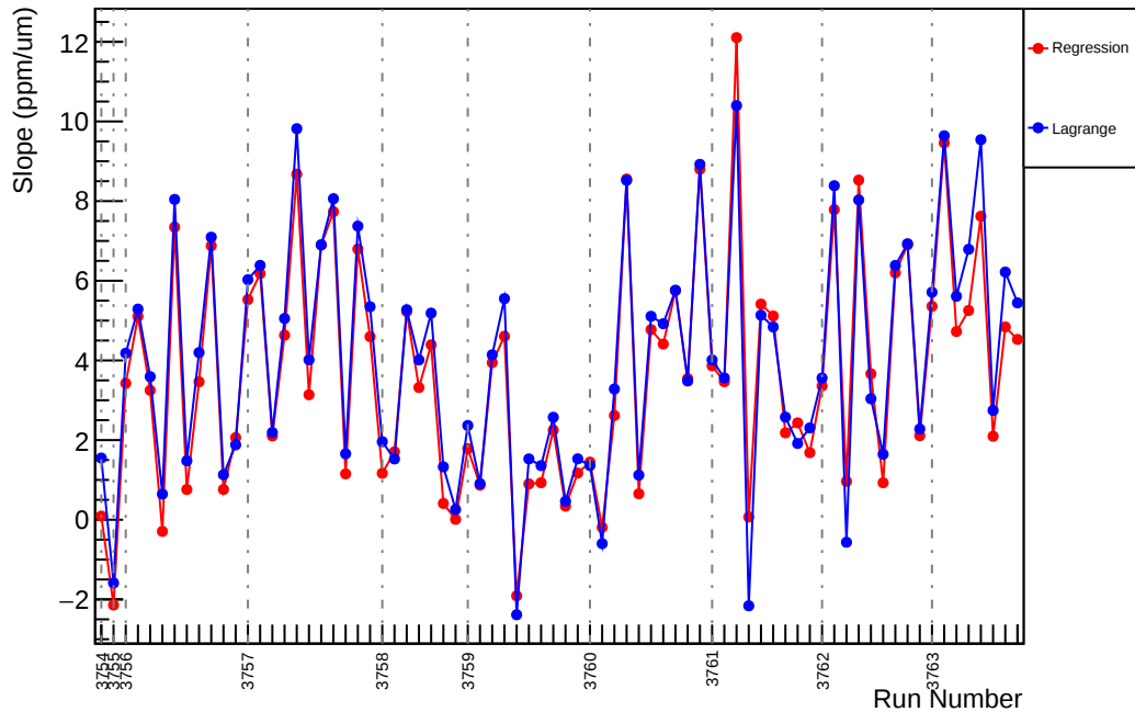
Slug21: Slope : usr_vs_evMon8 (ppm/um)
