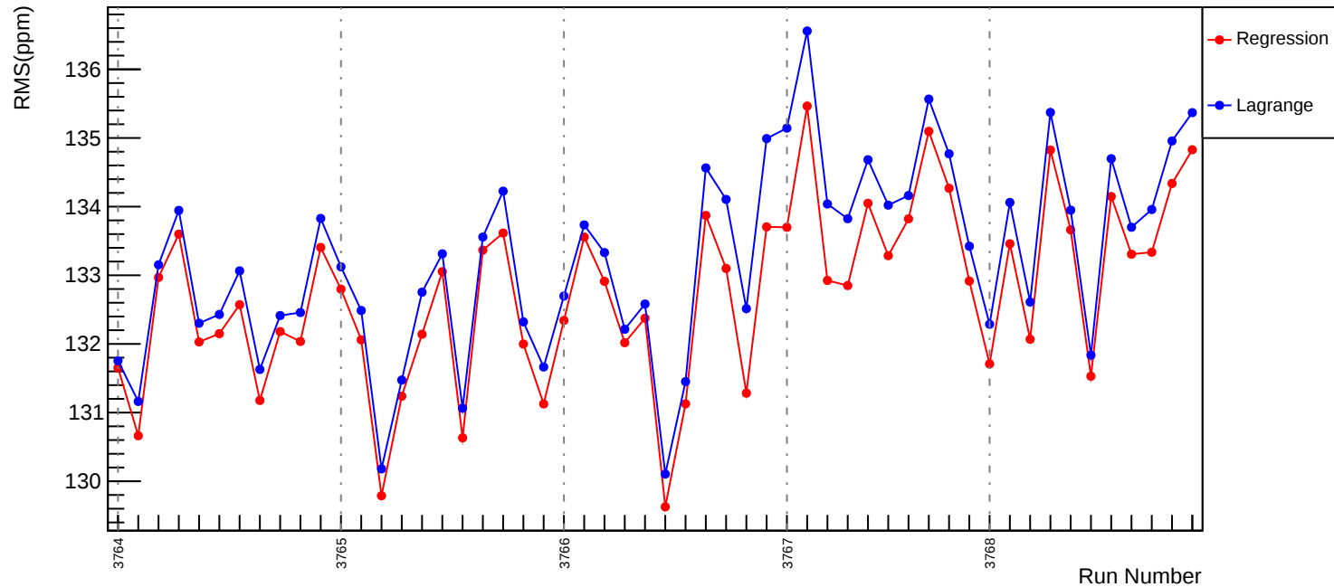
Slug22: Corrected RMS (ppm): asym_usl
