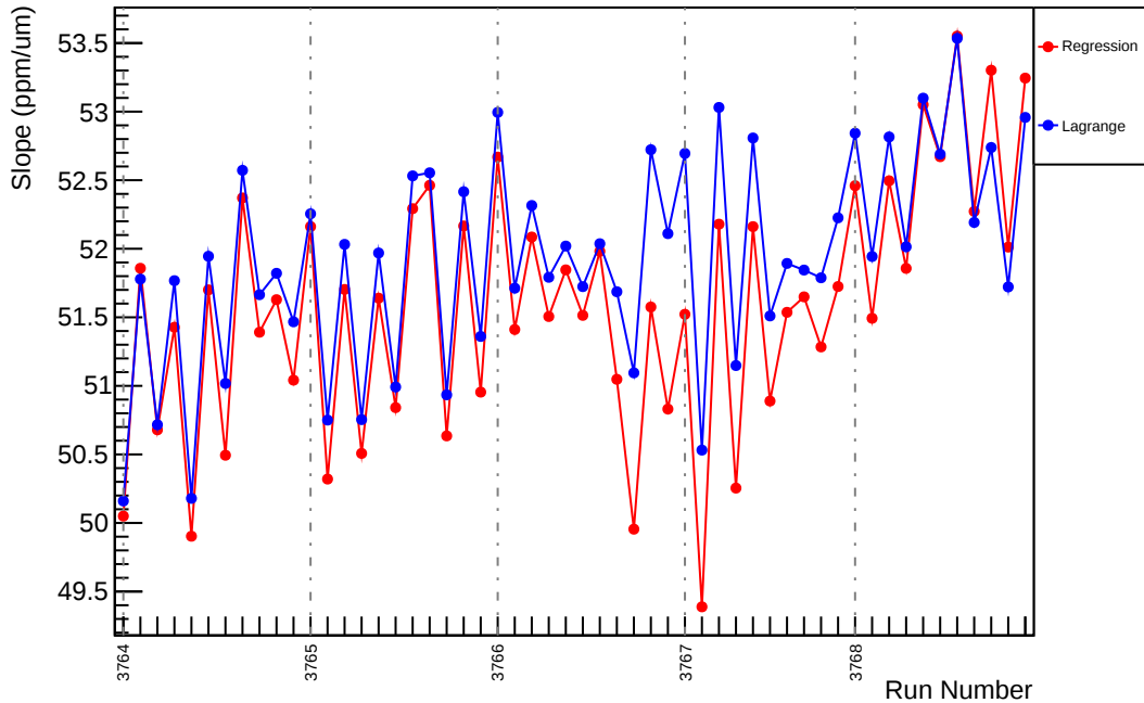
Slug22: Slope : usl_vs_evMon0 (ppm/um)
