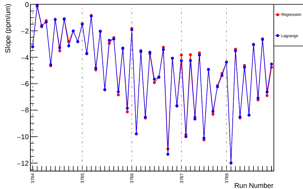
Slug22: Slope : usl_vs_evMon1 (ppm/um)
