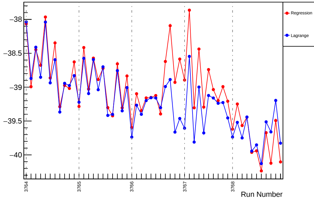
Slug22: Slope : usl_vs_evMon0 (ppm/um)
