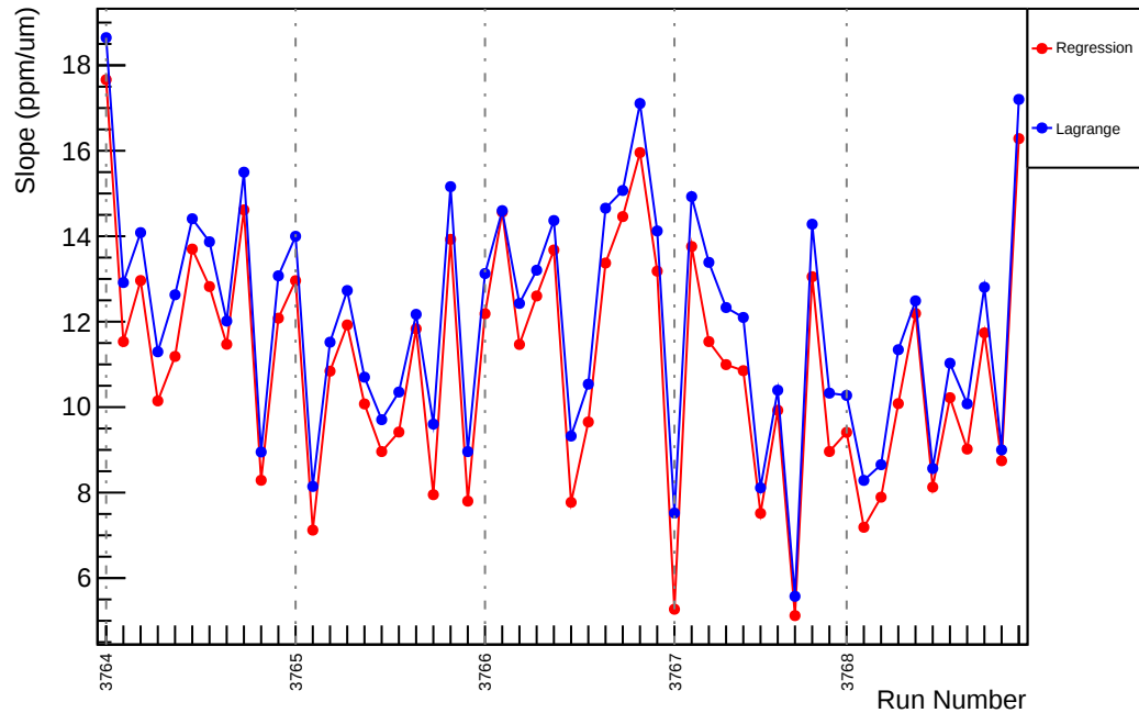
Slug22: Slope : usl_vs_evMon7 (ppm/um)
