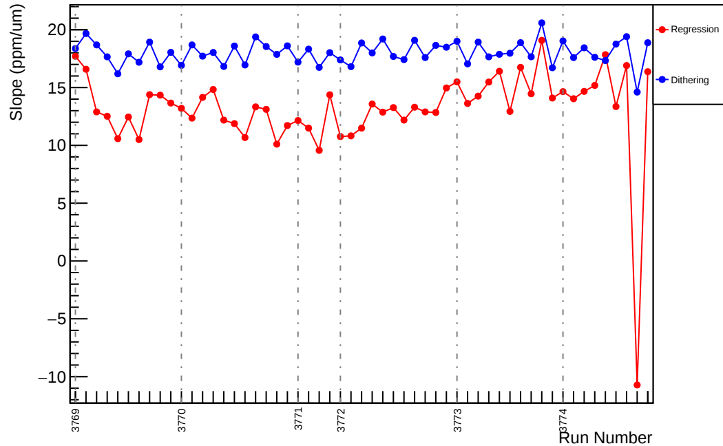
Slug23: Slope : usl_vs_evMon4 (ppm/um)
