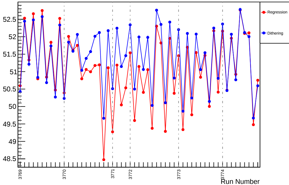
Slug23: Slope : usl_vs_evMon0 (ppm/um)
