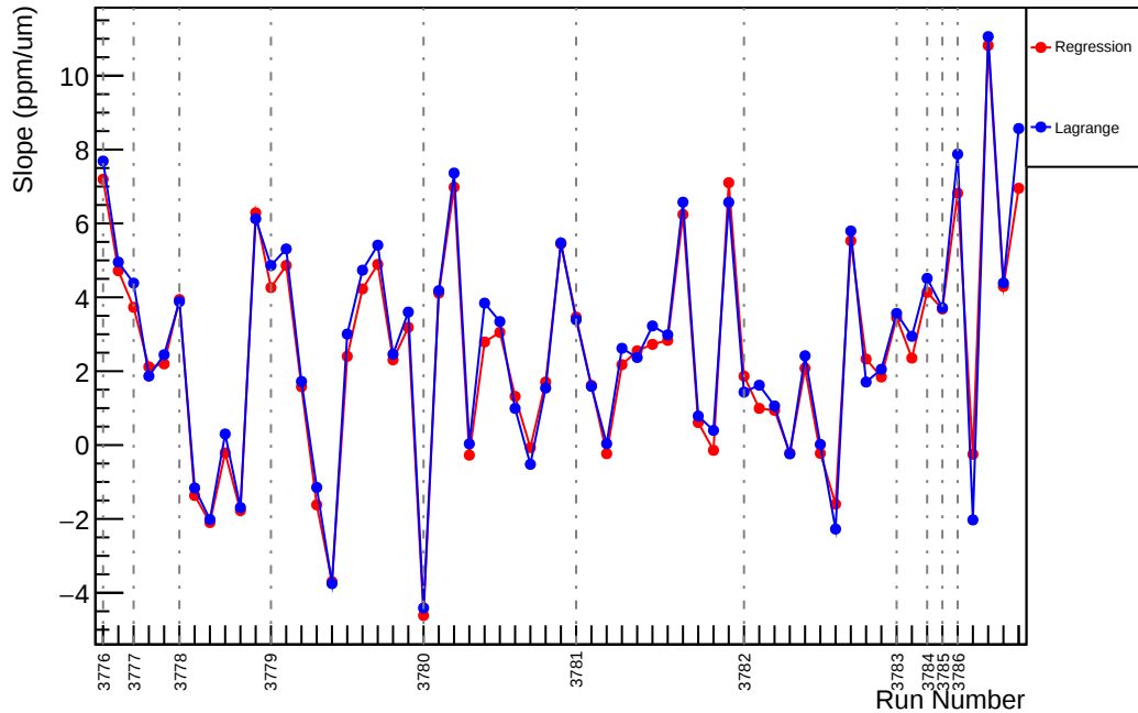
Slug24: Slope : usr_vs_evMon8 (ppm/um)
