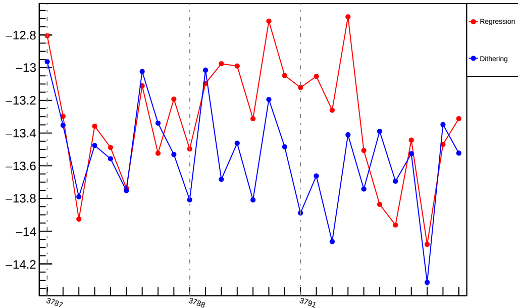
Slug25: Slope : us_dd_vs_evMon2 (ppm/um)
