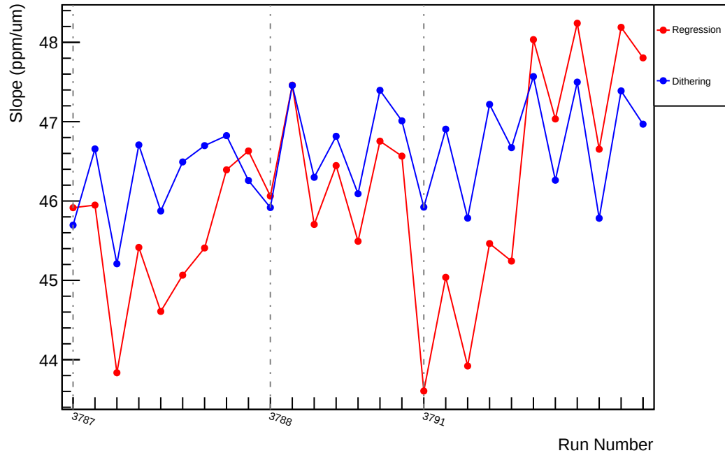
Slug25: Slope : usl_vs_evMon0 (ppm/um)
