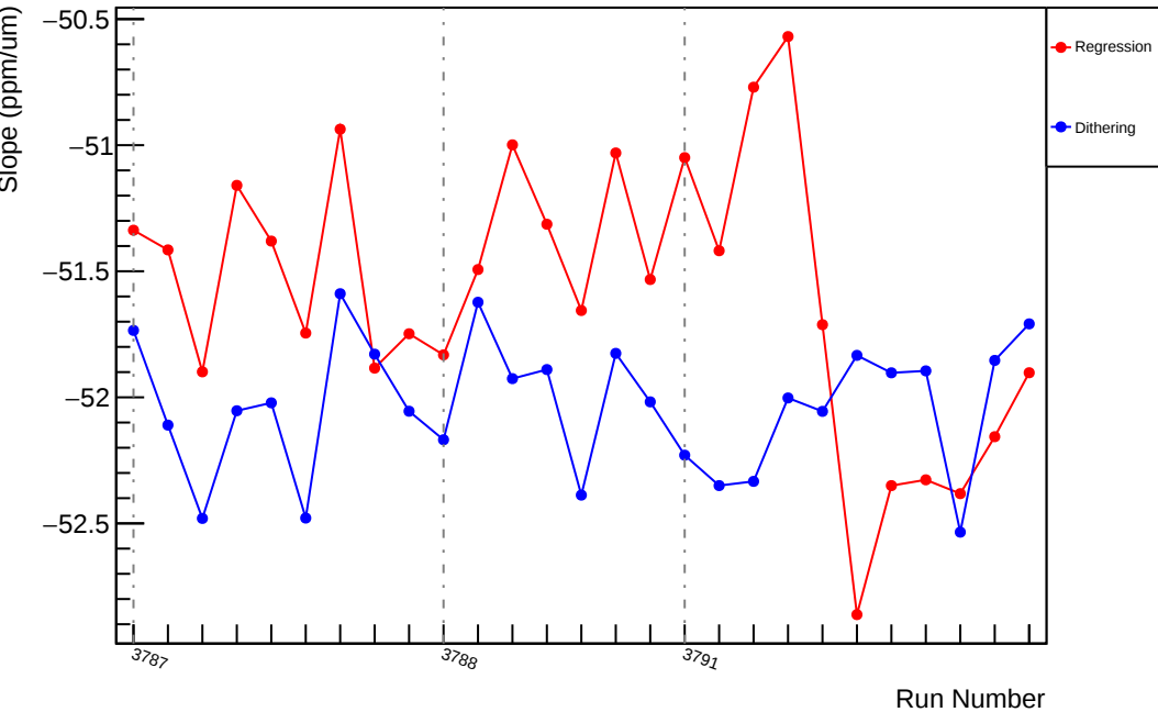
Slug25: Slope : usl_vs_evMon2 (ppm/um)
