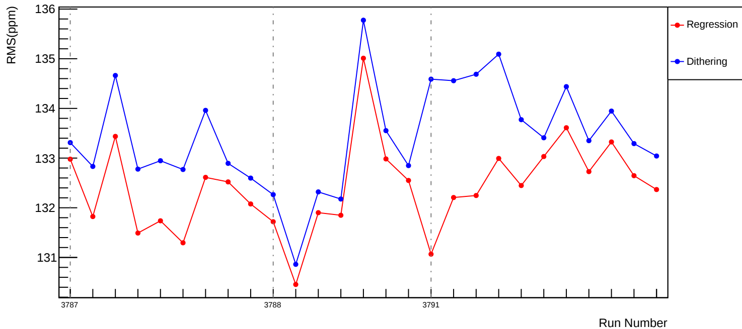
Slug25: Corrected RMS (ppm): asym_usl
