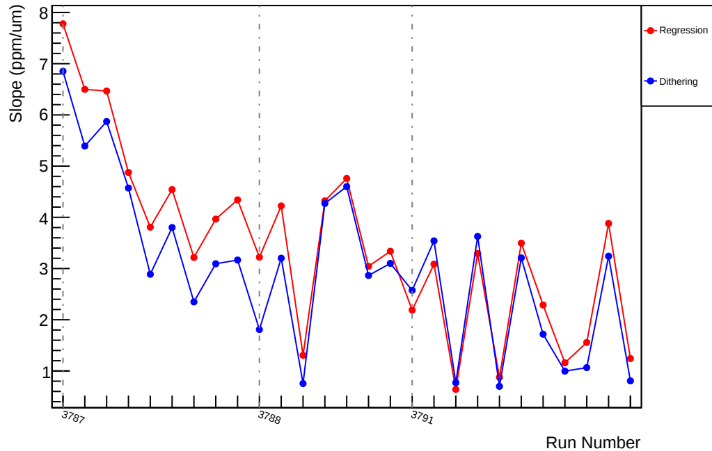
Slug25: Slope : usl_vs_evMon1 (ppm/um)
