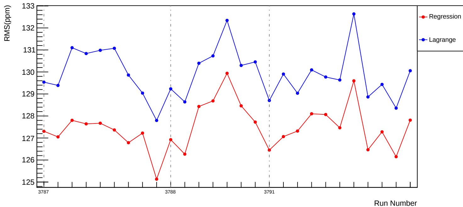
Slug25: Corrected RMS (ppm): asym_usr
