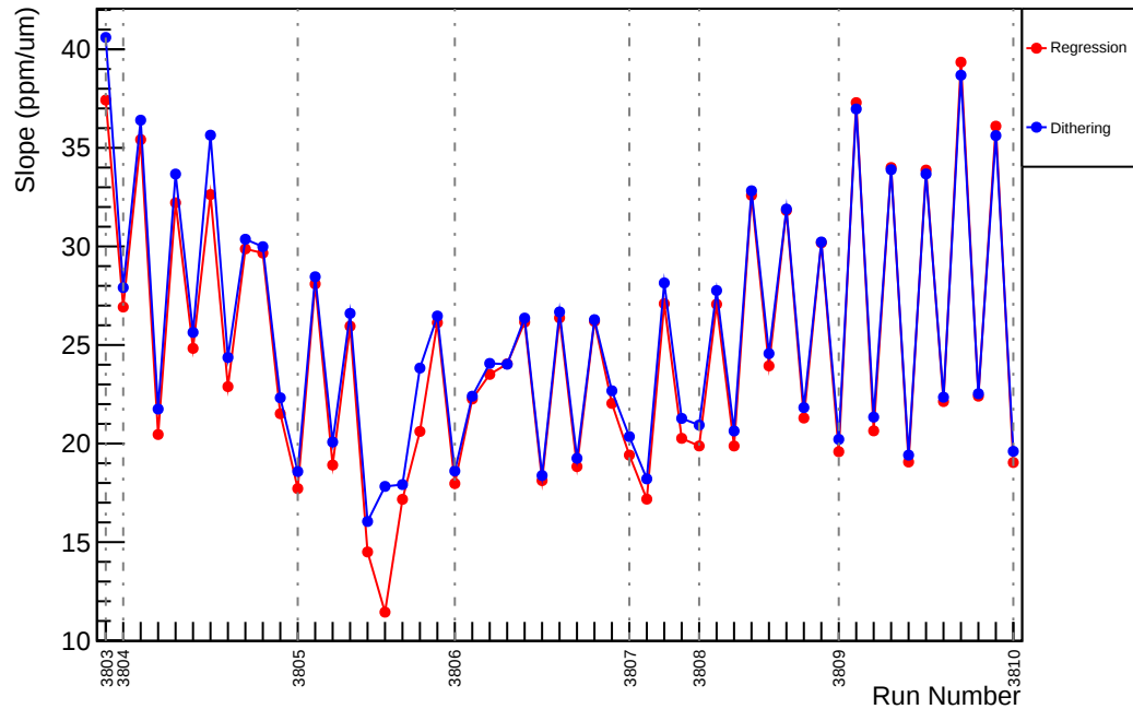
Slug26: Slope : us_avg_vs_evMon2 (ppm/um)
