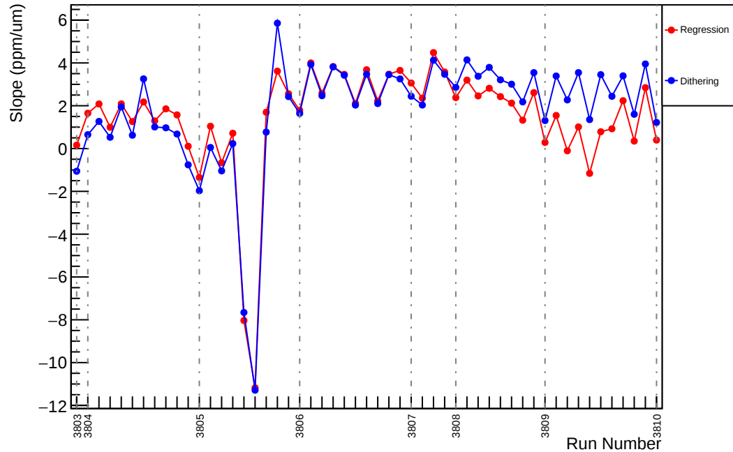
Slug26: Slope : us_avg_vs_evMon0 (ppm/um)
