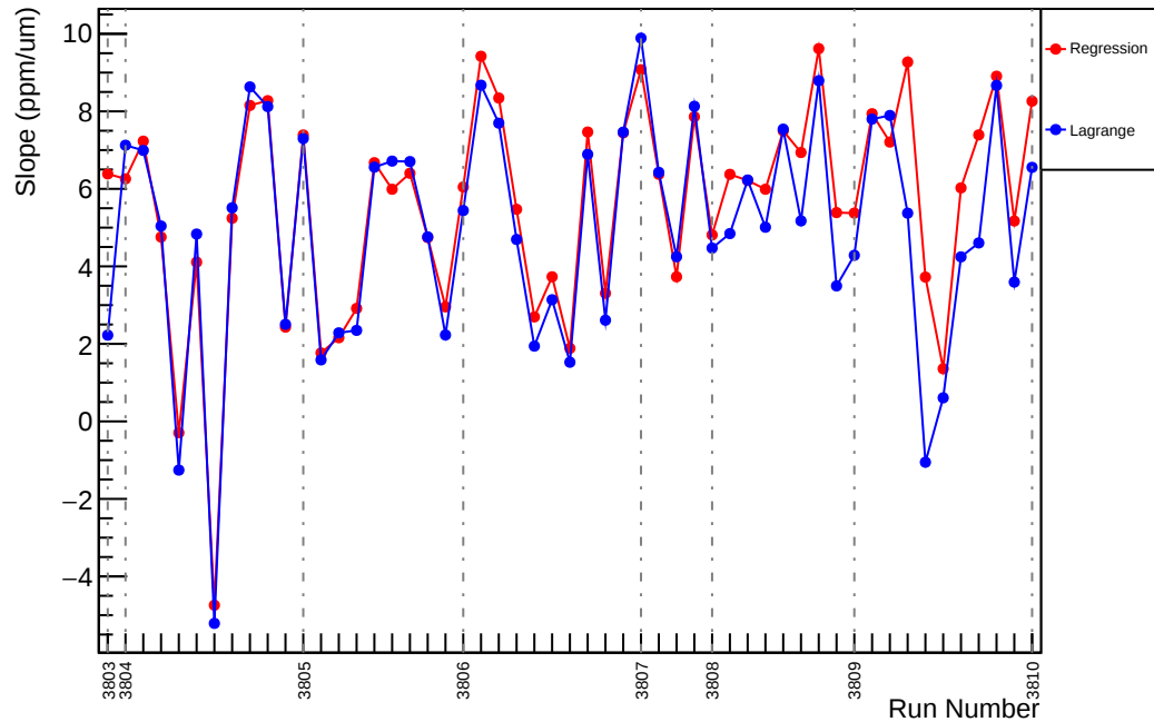
Slug26: Slope : us_avg_vs_evMon9 (ppm/um)
