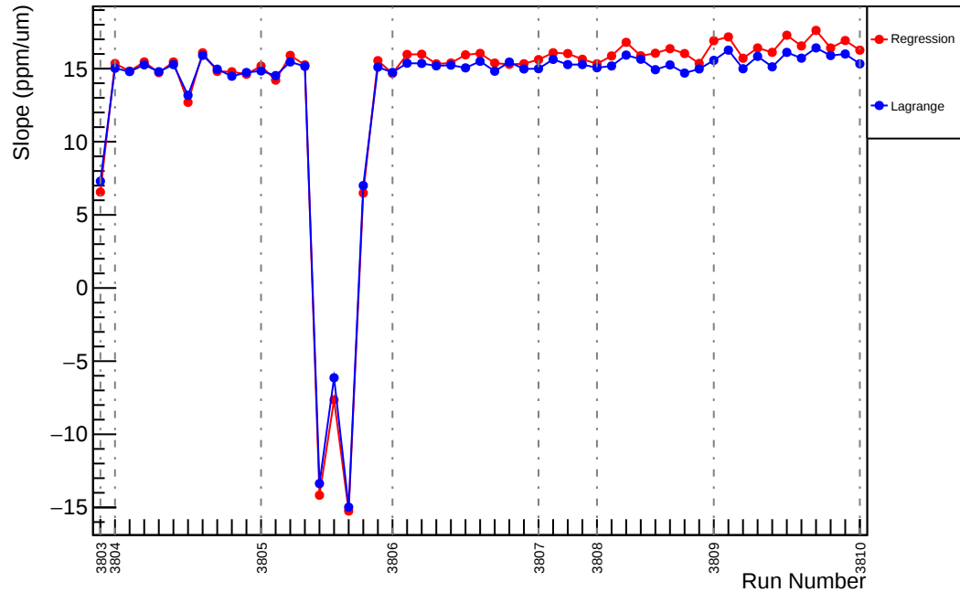
Slug26: Slope : us_avg_vs_evMon4 (ppm/um)
