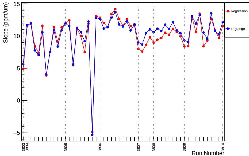
Slug26: Slope : us_avg_vs_evMon6 (ppm/um)
