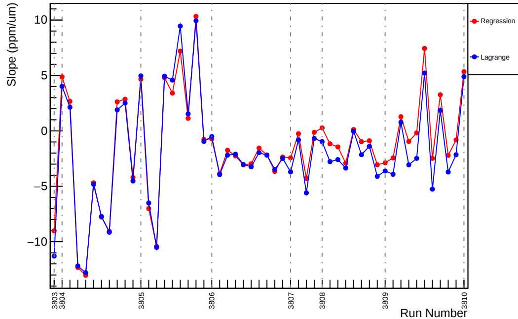
Slug26: Slope : us_avg_vs_evMon7 (ppm/um)
