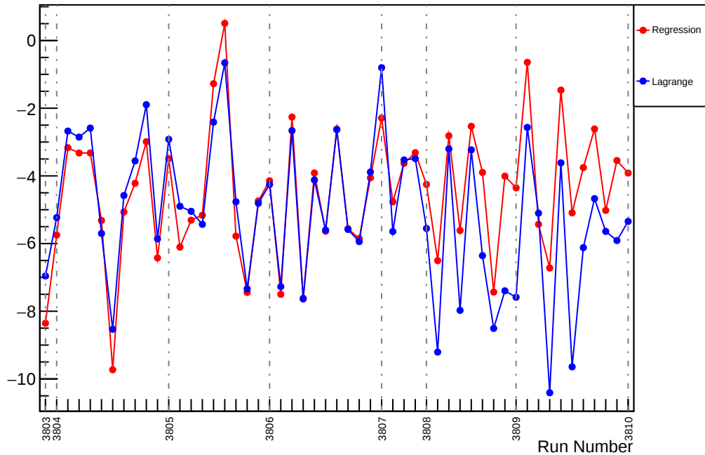
Slug26: Slope : us_avg_vs_evMon8 (ppm/um)
