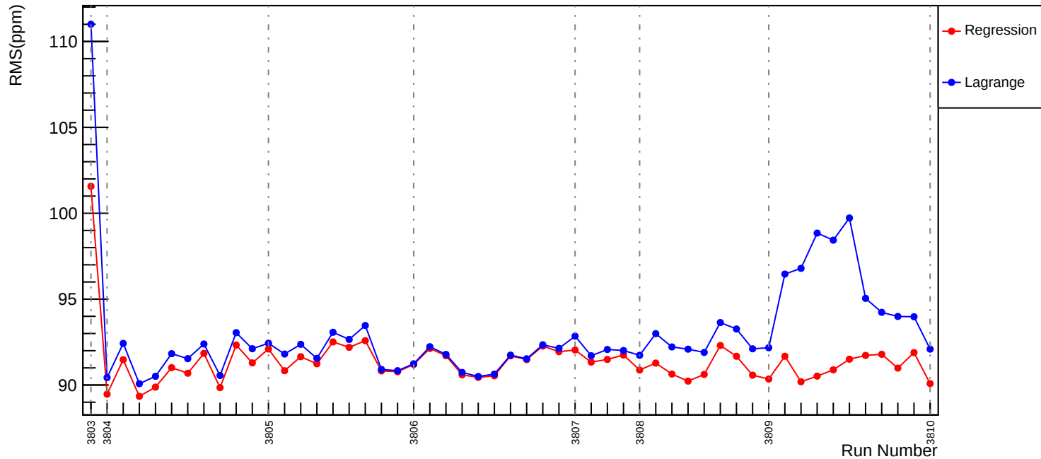
Slug26: Corrected RMS (ppm): asym_us_avg
