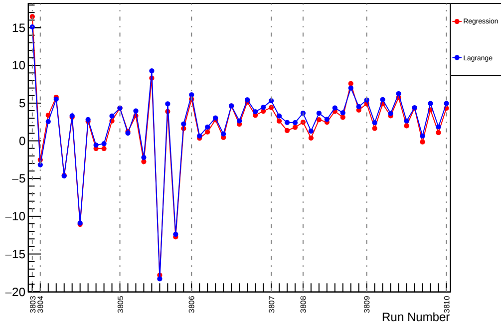
Slug26: Slope : us_avg_vs_evMon3 (ppm/um)
