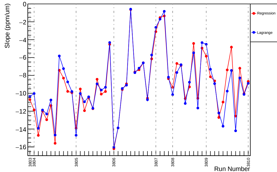
Slug26: Slope : us_avg_vs_evMon11 (ppm/um)
