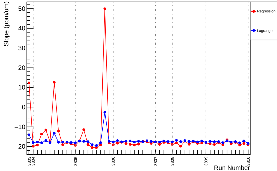
Slug26: Slope : us_dd_vs_evMon3 (ppm/um)
