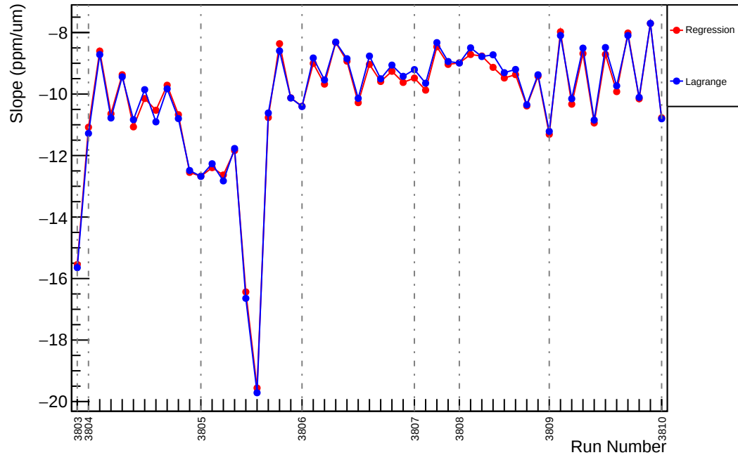
Slug26: Slope : us_dd_vs_evMon1 (ppm/um)
