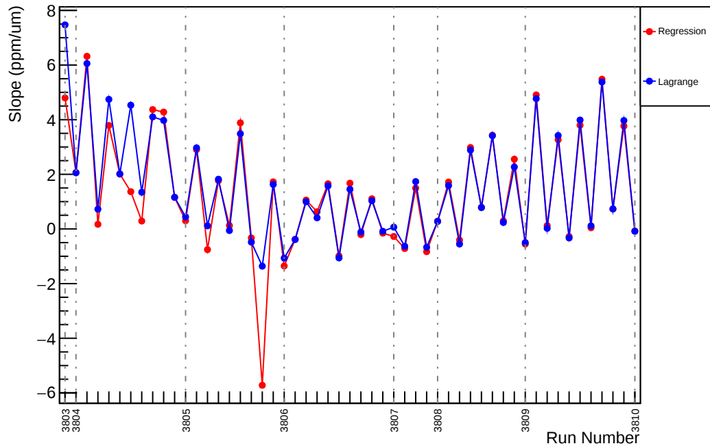
Slug26: Slope : us_dd_vs_evMon2 (ppm/um)
