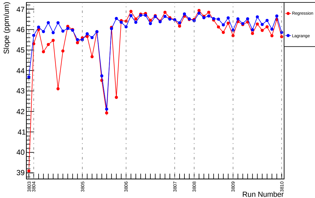
Slug26: Slope : us_dd_vs_evMon0 (ppm/um)
