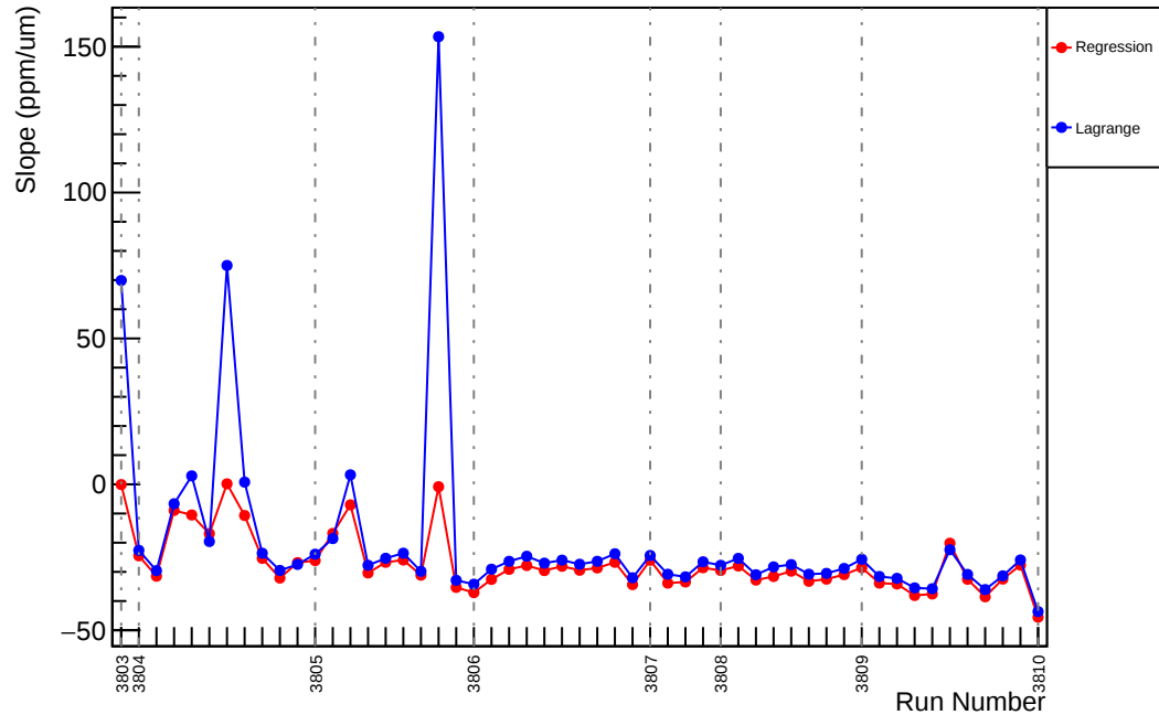
Slug26: Slope : us_dd_vs_evMon5 (ppm/um)
