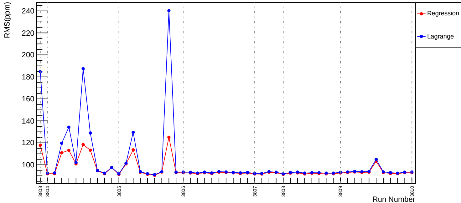
Slug26: Corrected RMS (ppm): asym_us_dd
