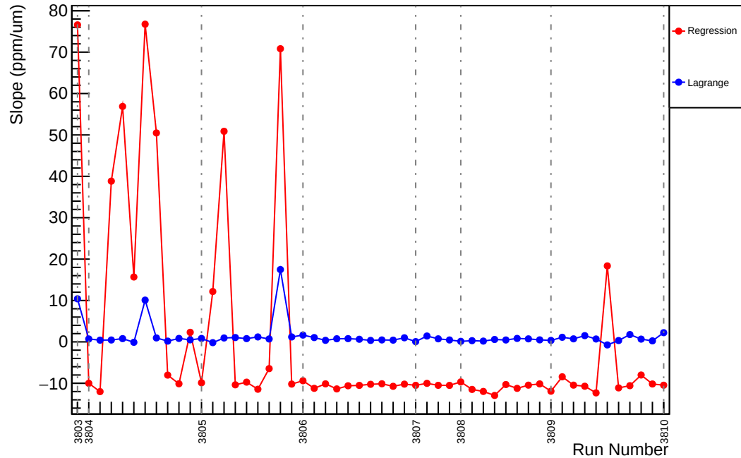
Slug26: Slope : us_dd_vs_evMon4 (ppm/um)
