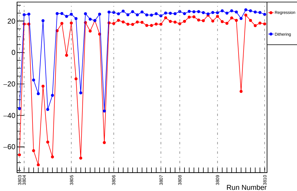
Slug26: Slope : usl_vs_evMon4 (ppm/um)
