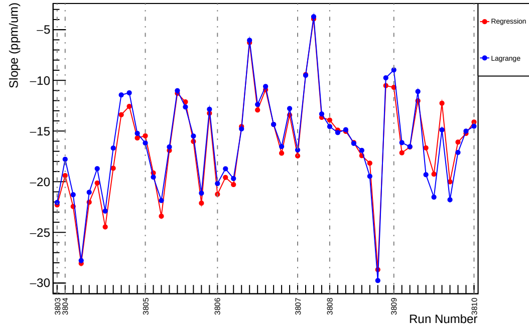
Slug26: Slope : usl_vs_evMon11 (ppm/um)
