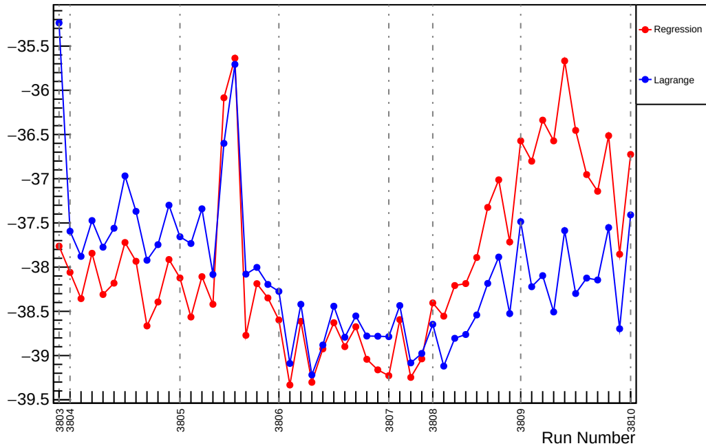
Slug26: Slope : usl_vs_evMon0 (ppm/um)
