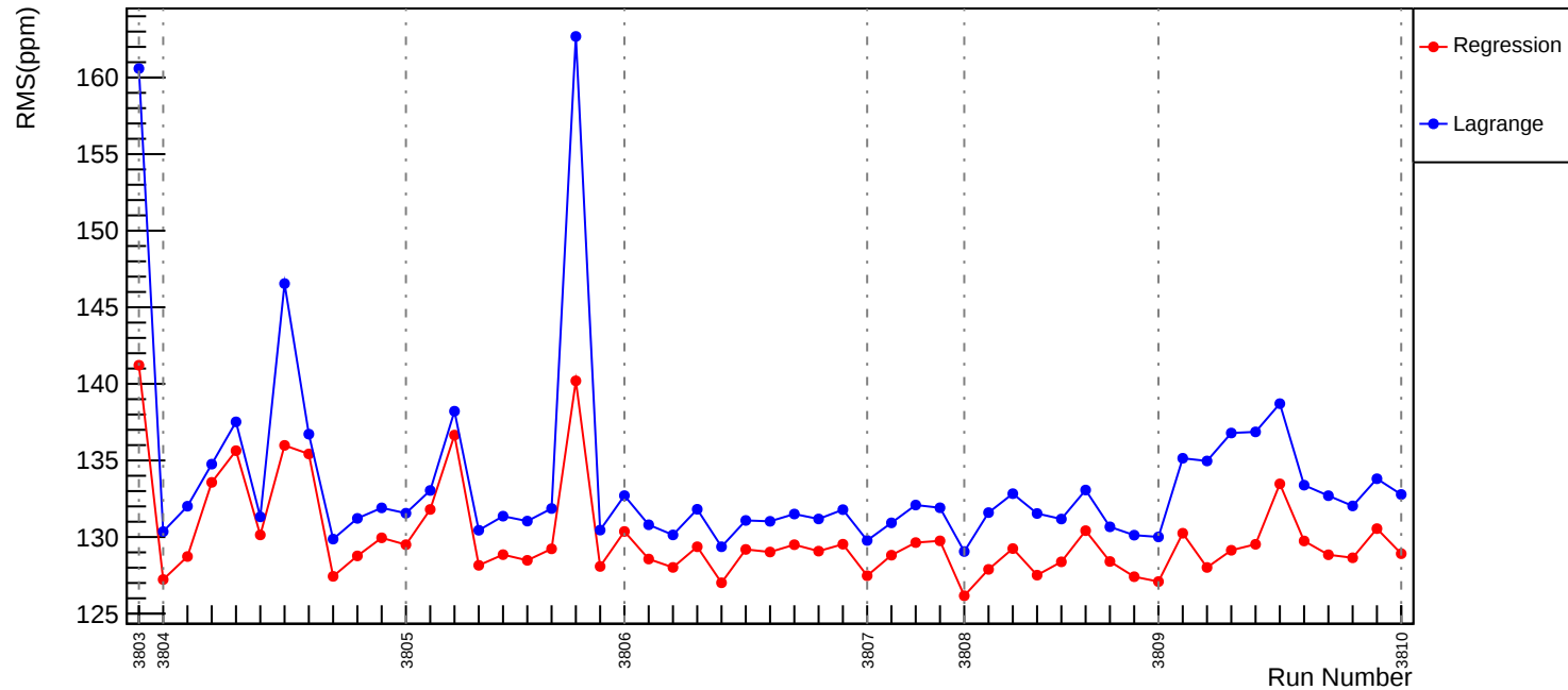
Slug26: Corrected RMS (ppm): asym_usr
