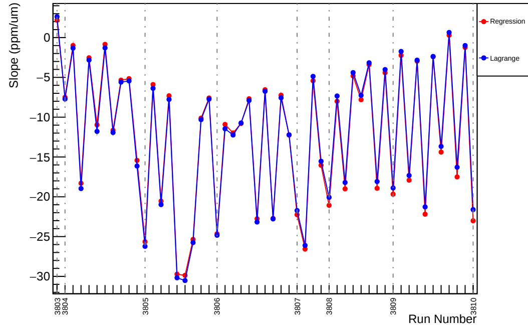
Slug26: Slope : usr_vs_evMon1 (ppm/um)
