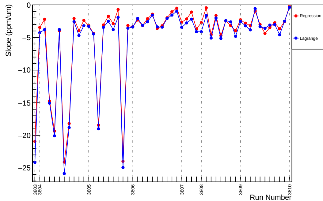
Slug26: Slope : usr_vs_evMon5 (ppm/um)
