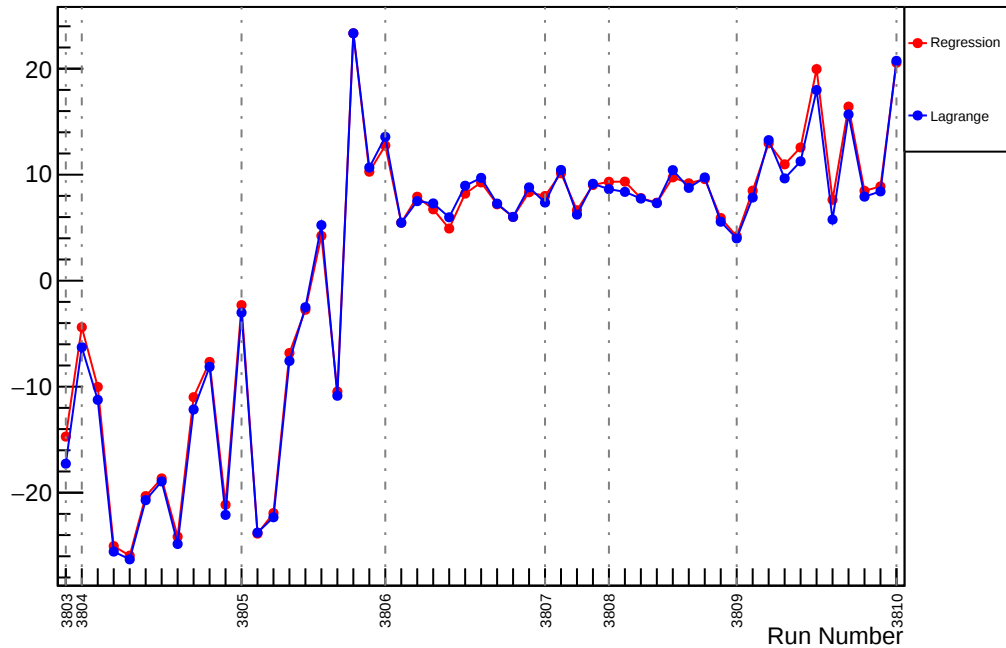
Slug26: Slope : usr_vs_evMon7 (ppm/um)
