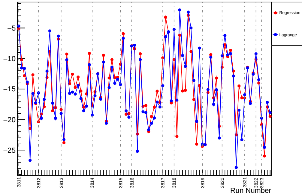
Slug27: Slope : usl_vs_evMon11 (ppm/um)
