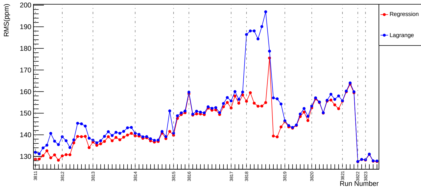
Slug27: Corrected RMS (ppm): asym_usl
