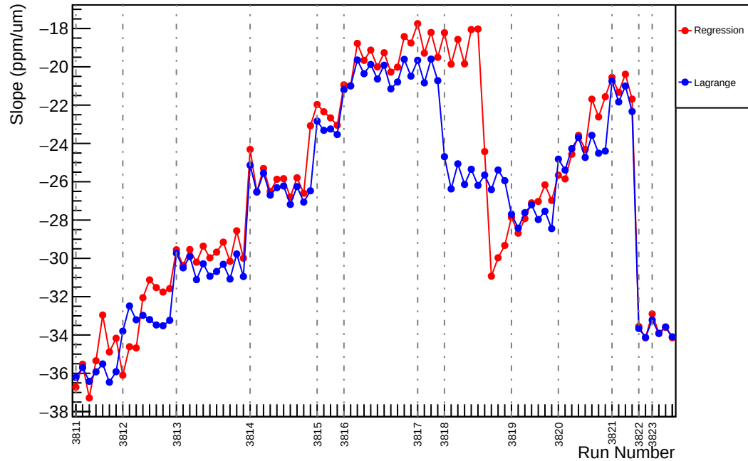
Slug27: Slope : usl_vs_evMon0 (ppm/um)
