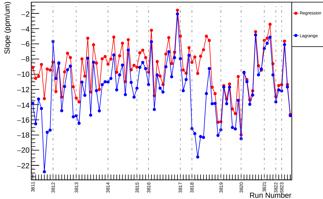
Slug27: Slope : usl_vs_evMon7 (ppm/um)
