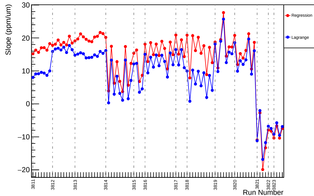
Slug27: Slope : usl_vs_evMon4 (ppm/um)
