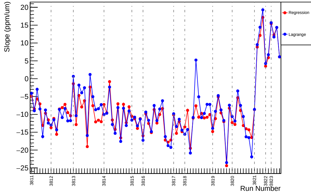
Slug27: Slope : usl_vs_evMon9 (ppm/um)
