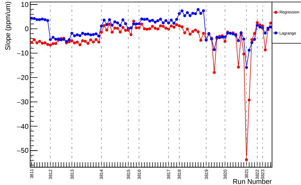
Slug27: Slope : usr_vs_evMon3 (ppm/um)
