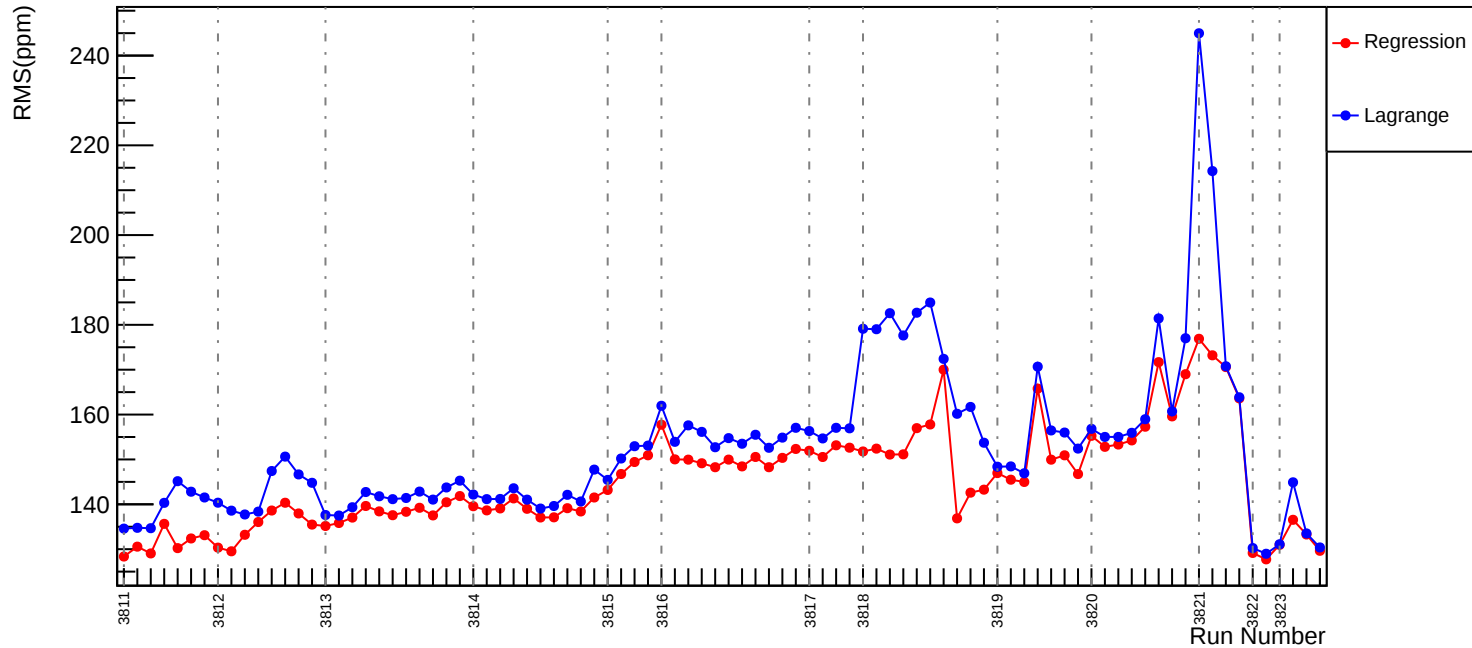
Slug27: Corrected RMS (ppm): asym_usr
