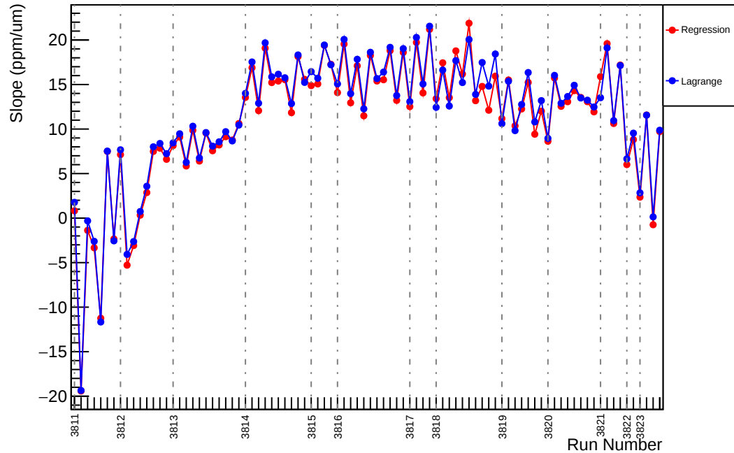
Slug27: Slope : usr_vs_evMon1 (ppm/um)
