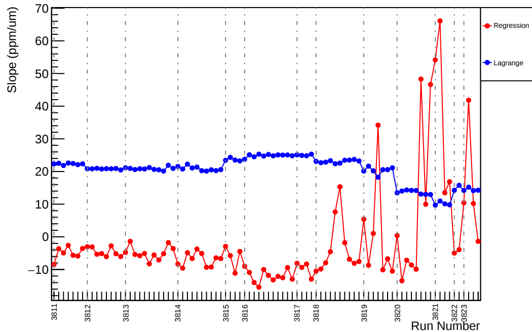
Slug27: Slope : usr_vs_evMon4 (ppm/um)
