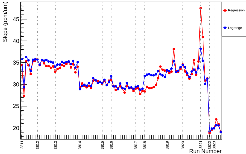
Slug27: Slope : usr_vs_evMon2 (ppm/um)
