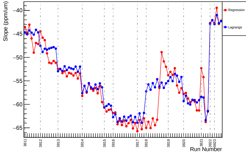
Slug27: Slope : usr_vs_evMon0 (ppm/um)
