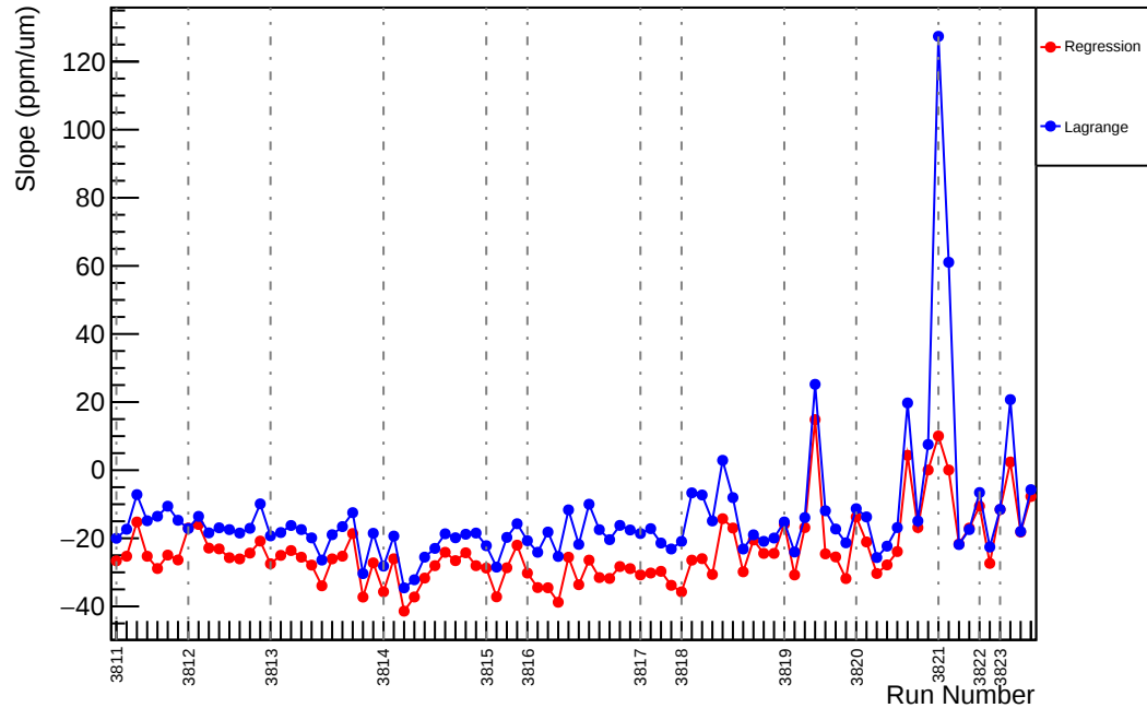
Slug27: Slope : usr_vs_evMon5 (ppm/um)
