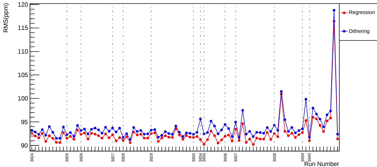
Slug28: Corrected RMS (ppm): asym_us_avg
