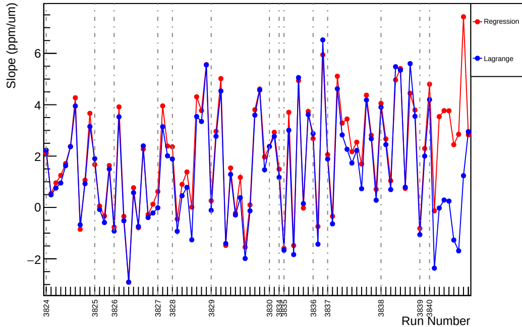
Slug28: Slope : us_dd_vs_evMon8 (ppm/um)
