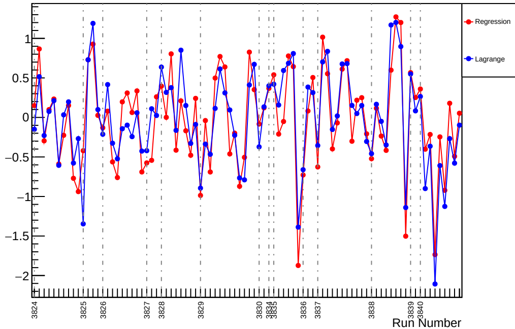
Slug28: Slope : us_dd_vs_evMon5 (ppm/um)
