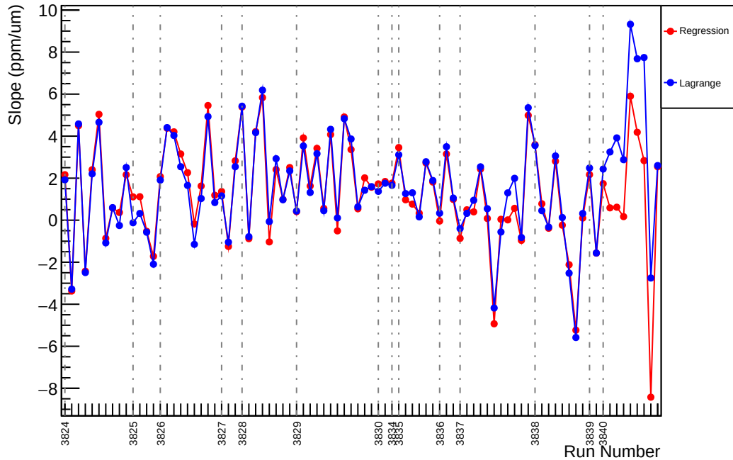
Slug28: Slope : us_dd_vs_evMon9 (ppm/um)
