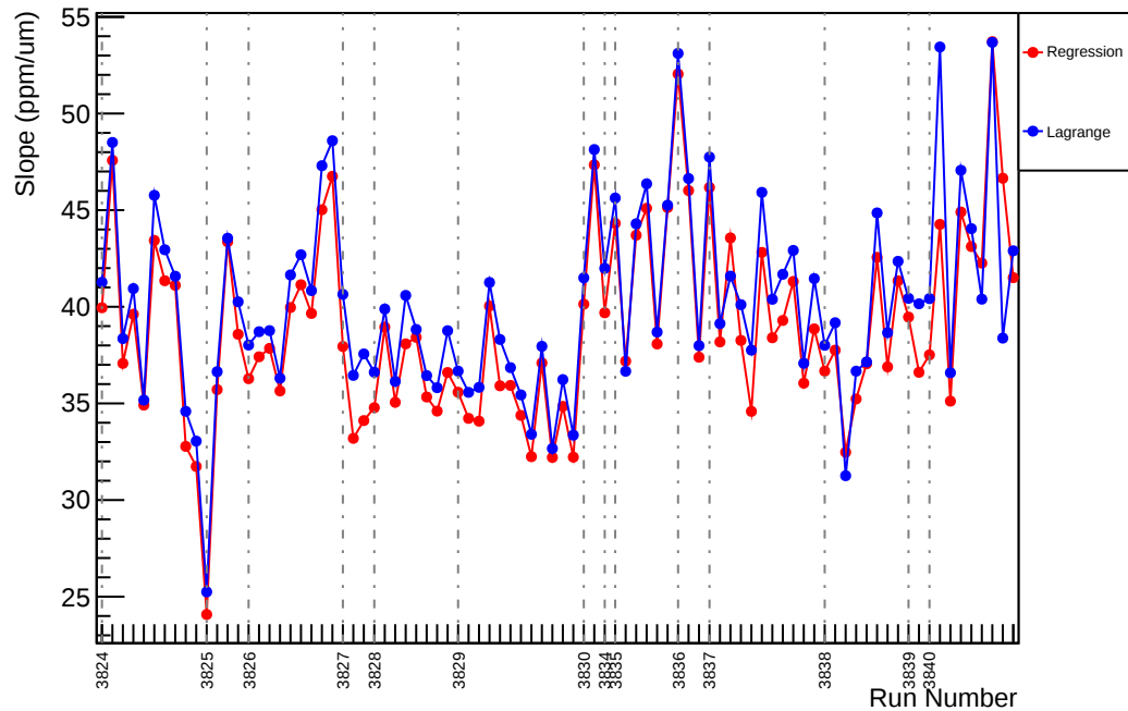
Slug28: Slope : usl_vs_evMon5 (ppm/um)
