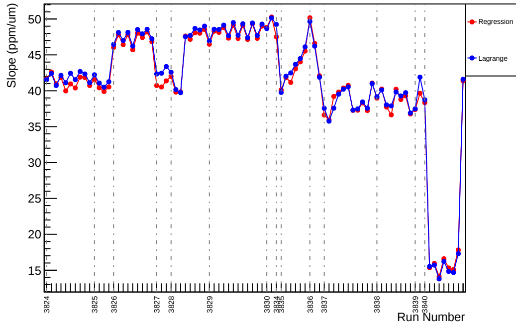
Slug28: Slope : usl_vs_evMon0 (ppm/um)
