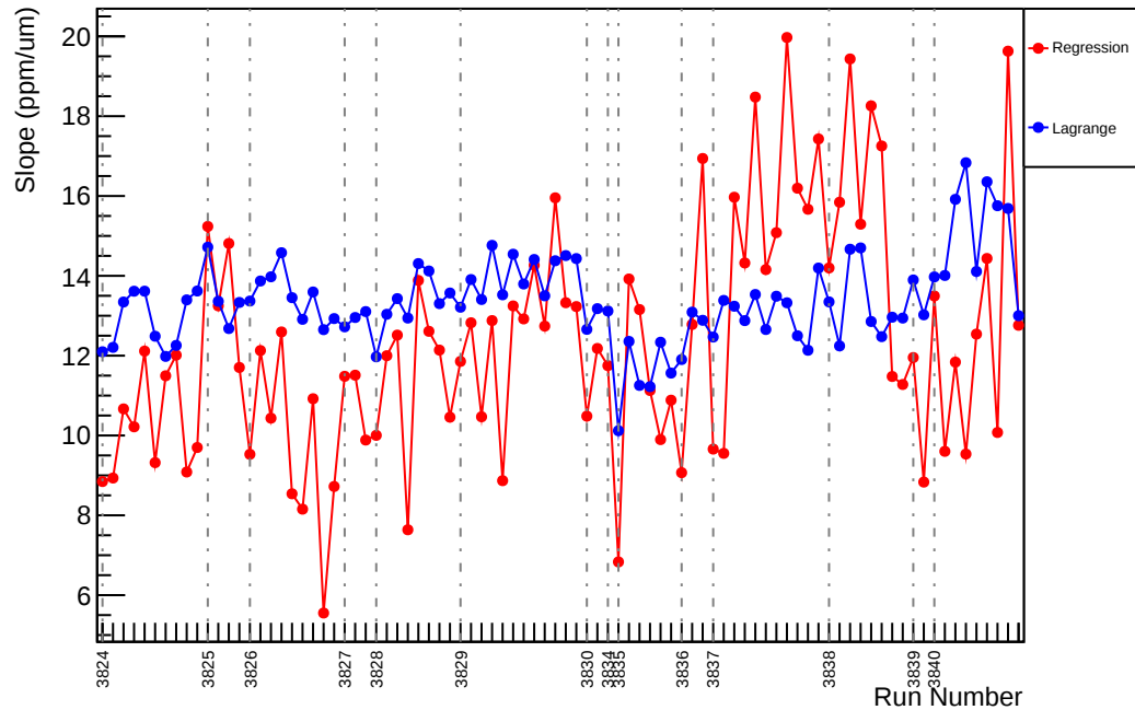
Slug28: Slope : usl_vs_evMon4 (ppm/um)
