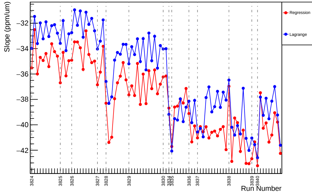
Slug28: Slope : usl_vs_evMon3 (ppm/um)
