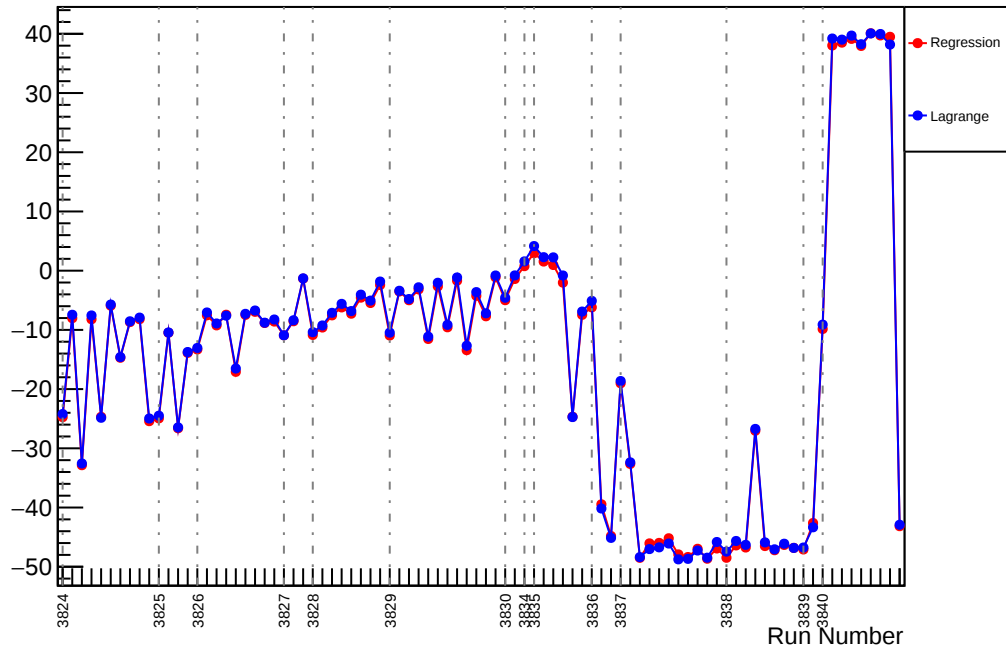
Slug28: Slope : usl_vs_evMon1 (ppm/um)
