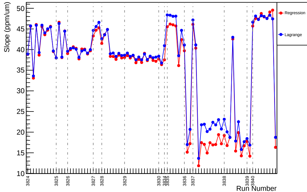
Slug28: Slope : usl_vs_evMon2 (ppm/um)
