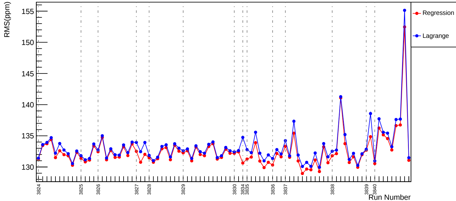
Slug28: Corrected RMS (ppm): asym_usl
