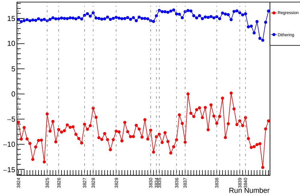
Slug28: Slope : usr_vs_evMon4 (ppm/um)
