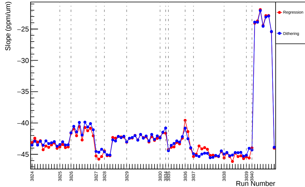
Slug28: Slope : usr_vs_evMon0 (ppm/um)
