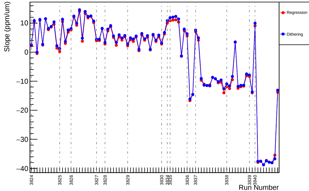
Slug28: Slope : usr_vs_evMon1 (ppm/um)
