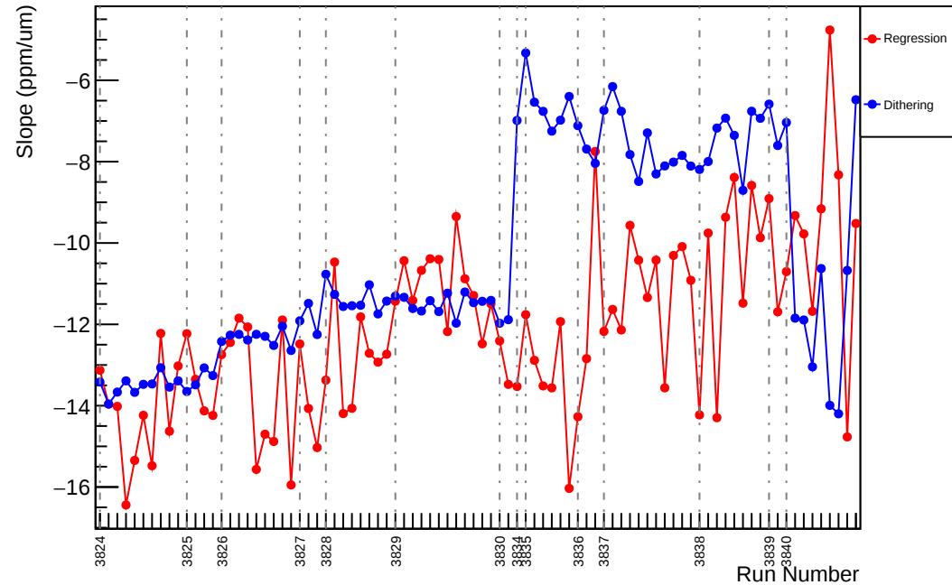
Slug28: Slope : usr_vs_evMon3 (ppm/um)
