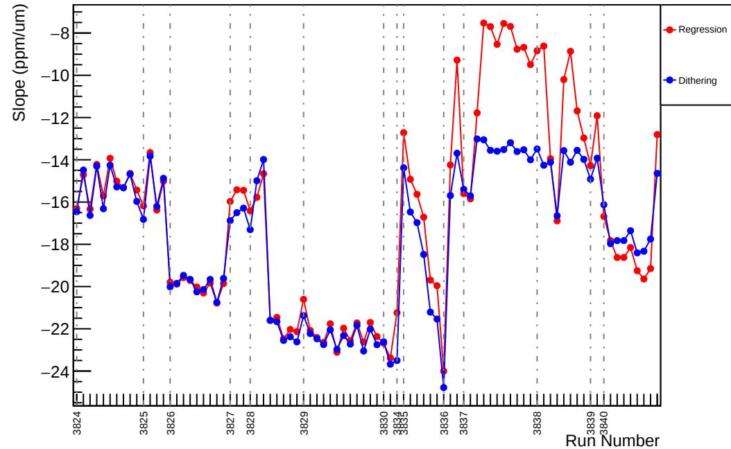
Slug28: Slope : usr_vs_evMon2 (ppm/um)
