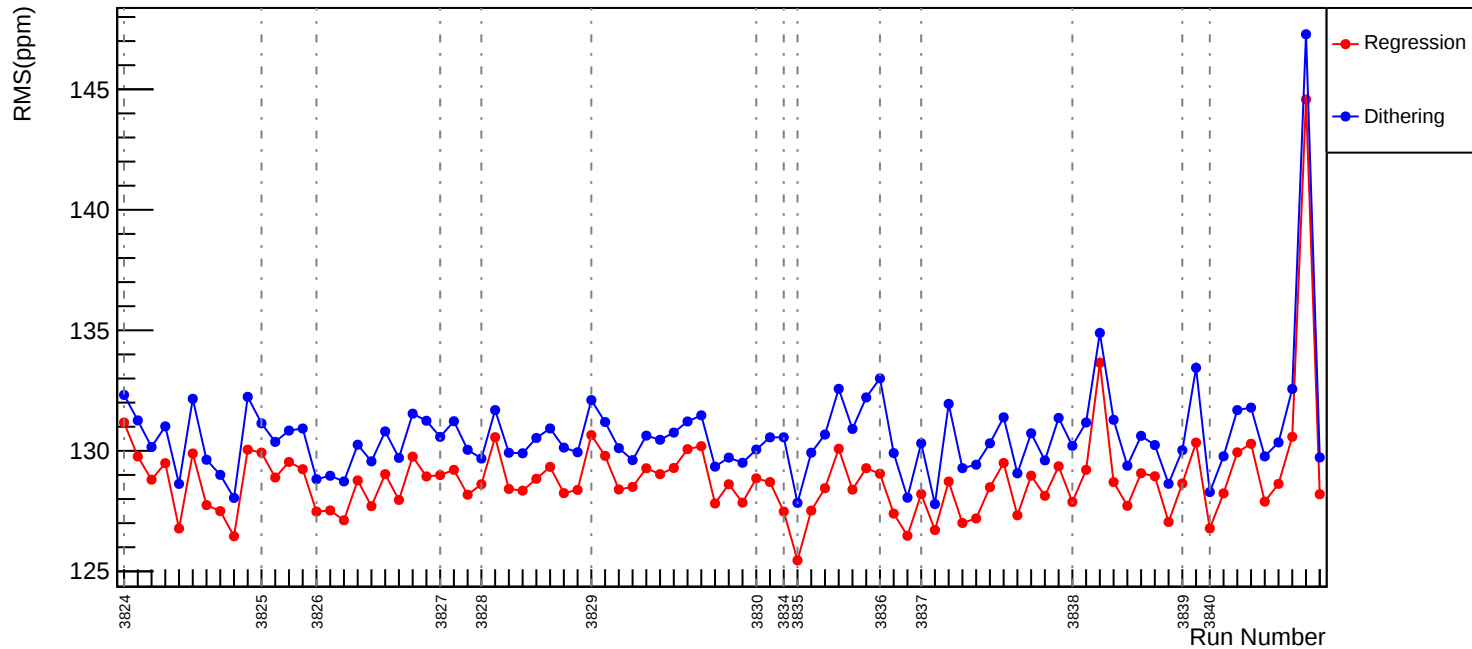
Slug28: Corrected RMS (ppm): asym_usr
