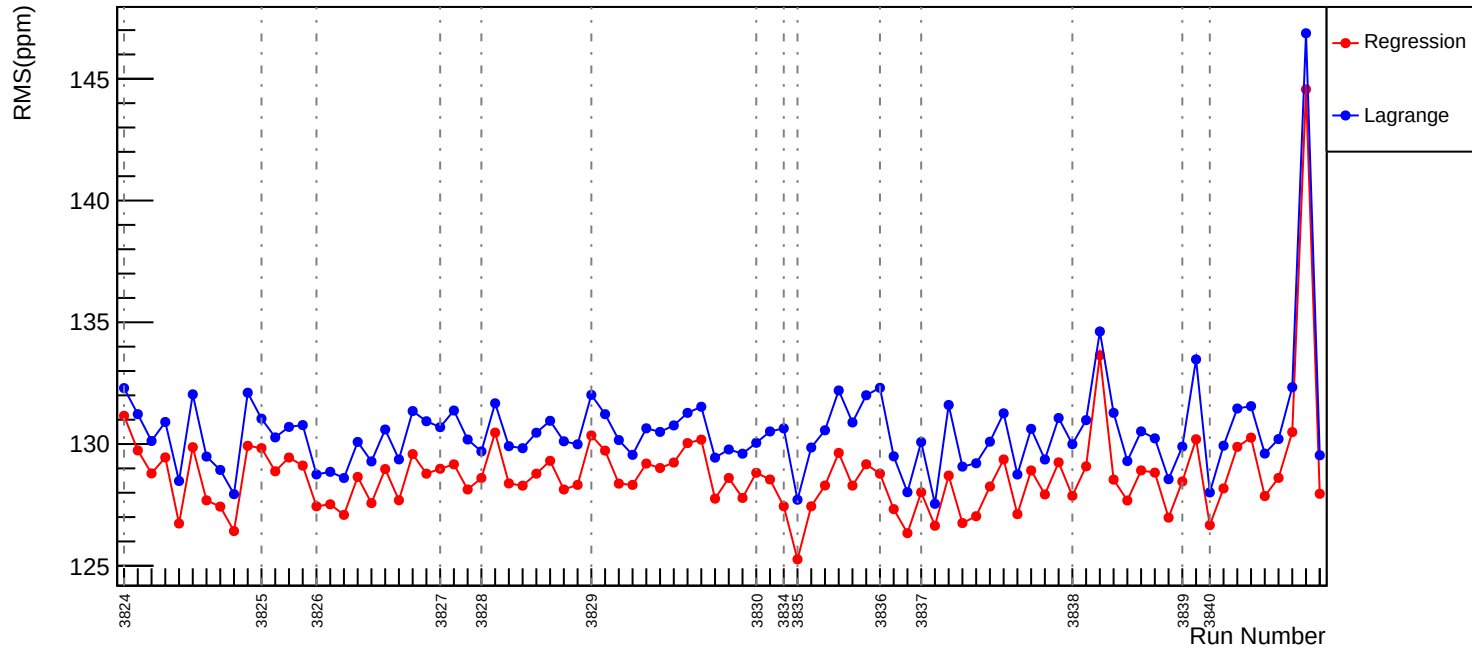
Slug28: Corrected RMS (ppm): asym_usr
