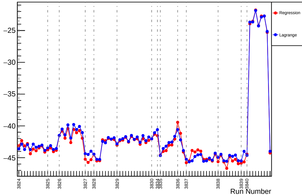
Slug28: Slope : usr_vs_evMon0 (ppm/um)
