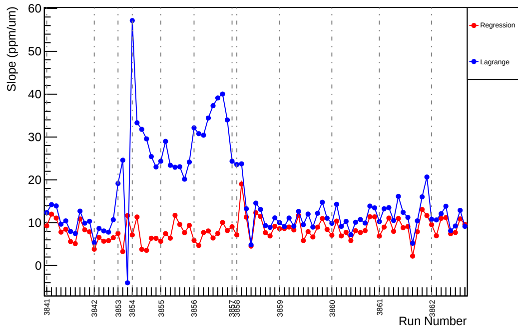
Slug29: Slope : us_avg_vs_evMon5 (ppm/um)
