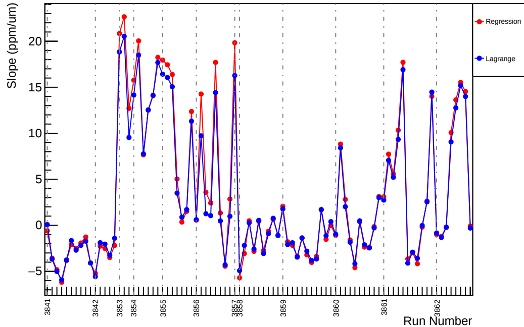
Slug29: Slope : us_dd_vs_evMon6 (ppm/um)
