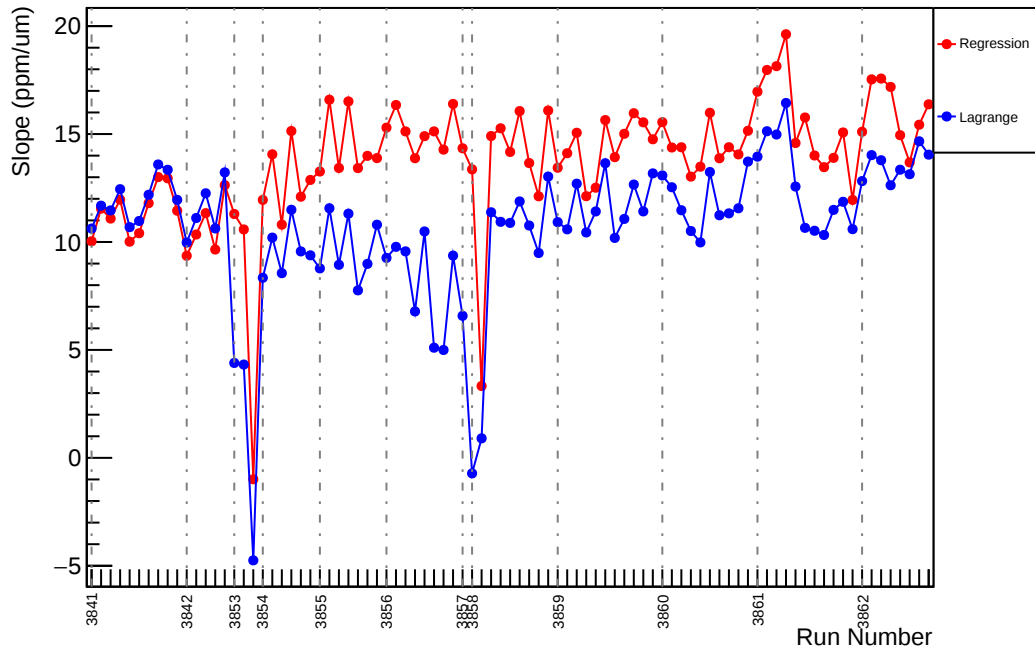
Slug29: Slope : us_dd_vs_evMon7 (ppm/um)
