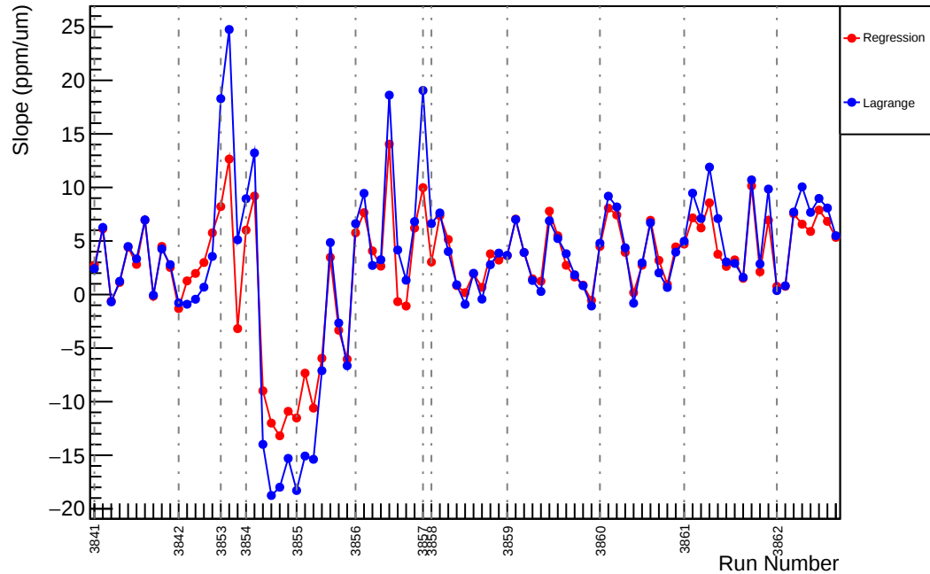
Slug29: Slope : us_dd_vs_evMon9 (ppm/um)
