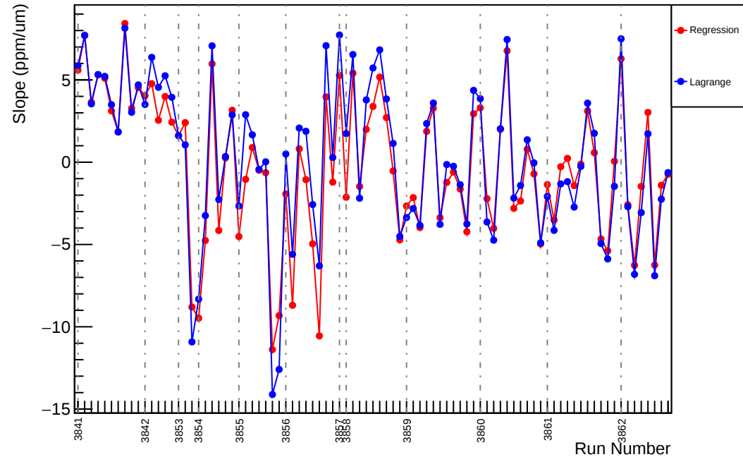
Slug29: Slope : us_dd_vs_evMon10 (ppm/um)
