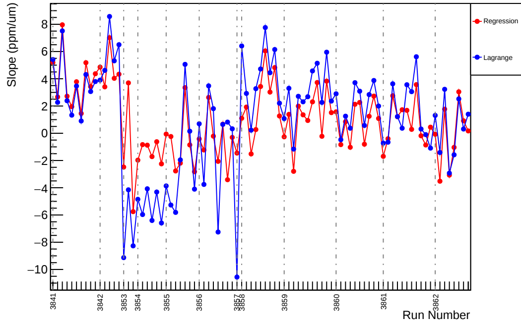
Slug29: Slope : us_dd_vs_evMon8 (ppm/um)
