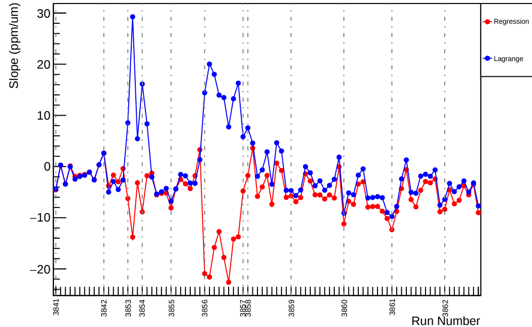
Slug29: Slope : us_dd_vs_evMon11 (ppm/um)
