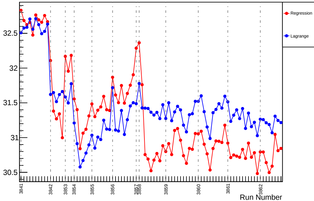
Slug29: Slope : us_dd_vs_evMon0 (ppm/um)
