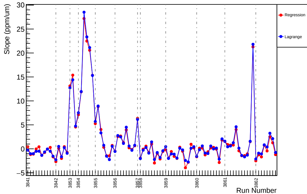
Slug29: Slope : usl_vs_evMon5 (ppm/um)
