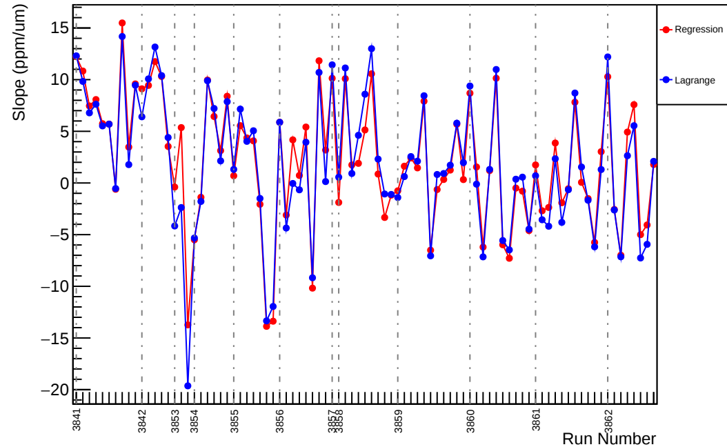
Slug29: Slope : usl_vs_evMon10 (ppm/um)
