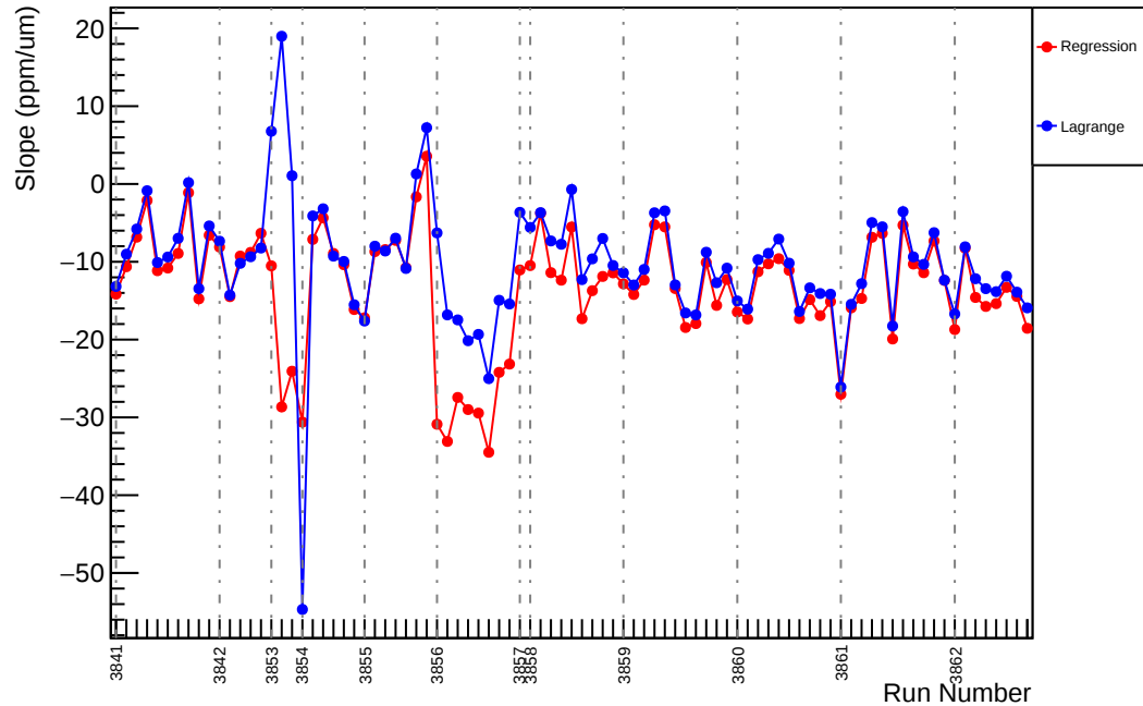
Slug29: Slope : usl_vs_evMon11 (ppm/um)
