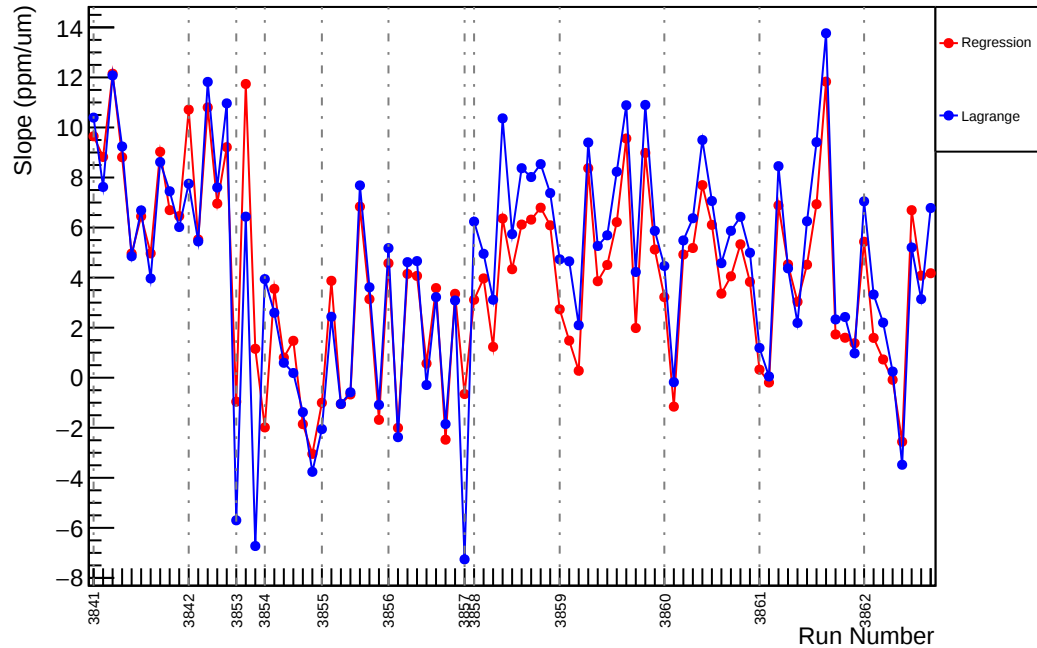
Slug29: Slope : usl_vs_evMon8 (ppm/um)
