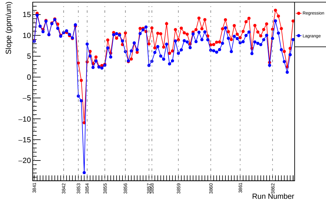
Slug29: Slope : usl_vs_evMon7 (ppm/um)
