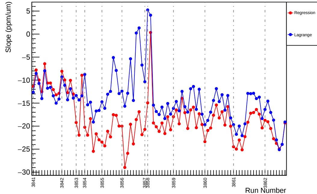
Slug29: Slope : usr_vs_evMon7 (ppm/um)
