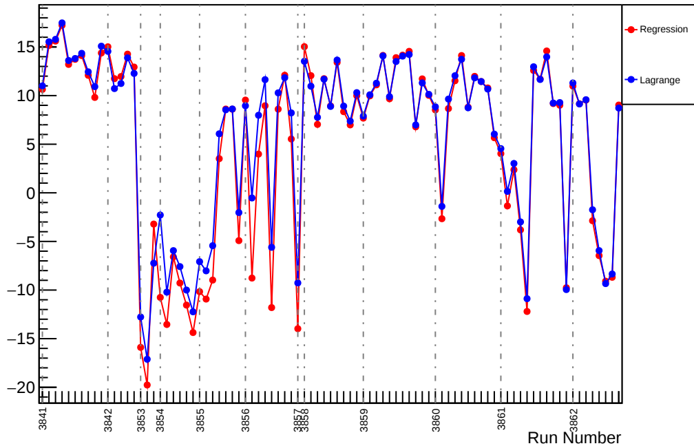
Slug29: Slope : usr_vs_evMon6 (ppm/um)
