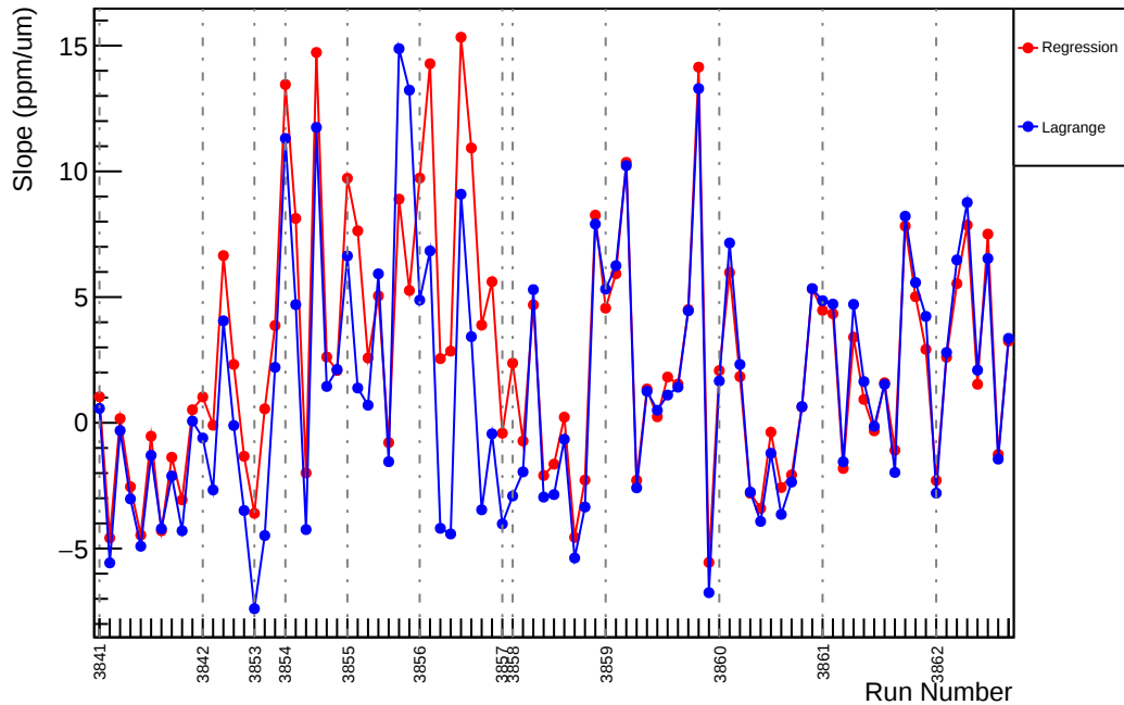
Slug29: Slope : usr_vs_evMon10 (ppm/um)
