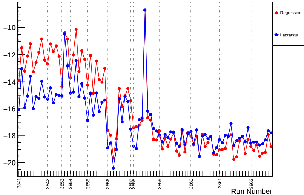
Slug29: Slope : usr_vs_evMon4 (ppm/um)
