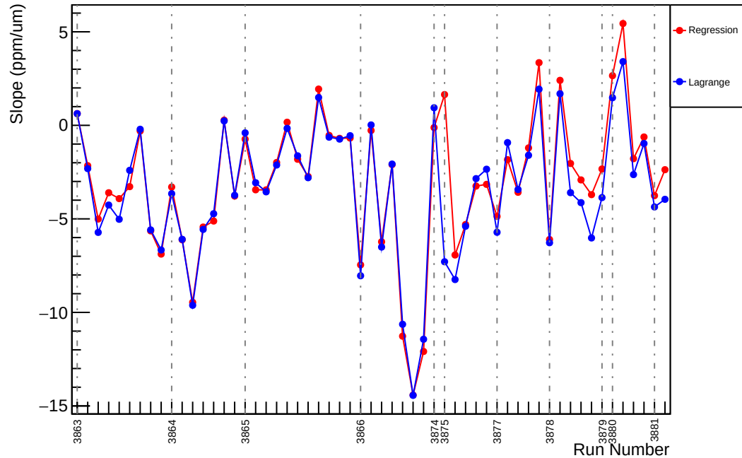
Slug30: Slope : us_avg_vs_evMon10 (ppm/um)
