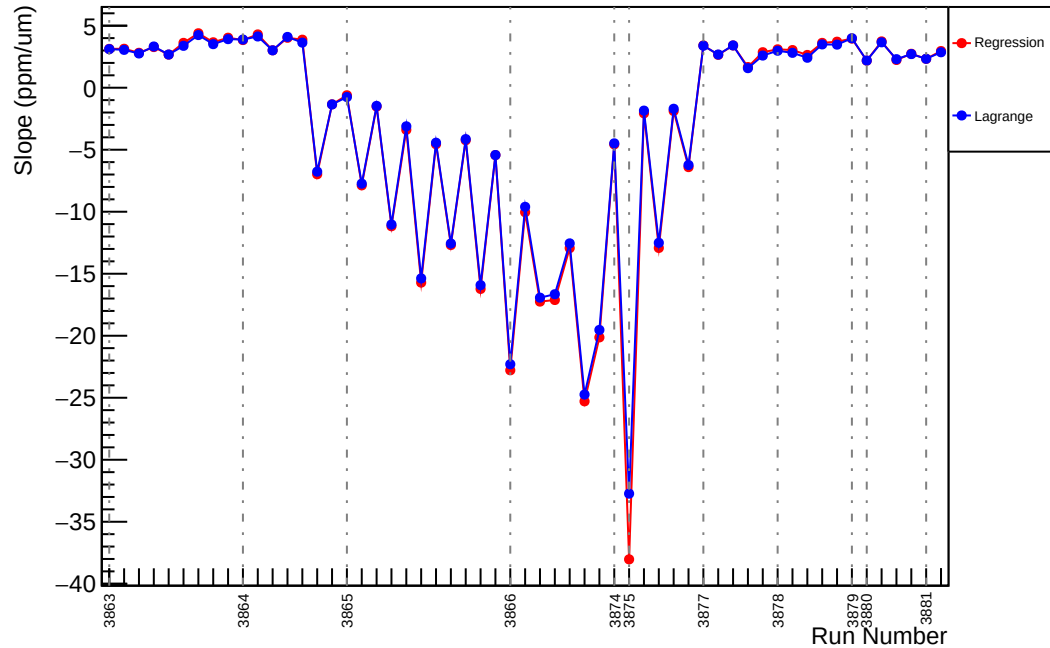
Slug30: Slope : us_avg_vs_evMon1 (ppm/um)
