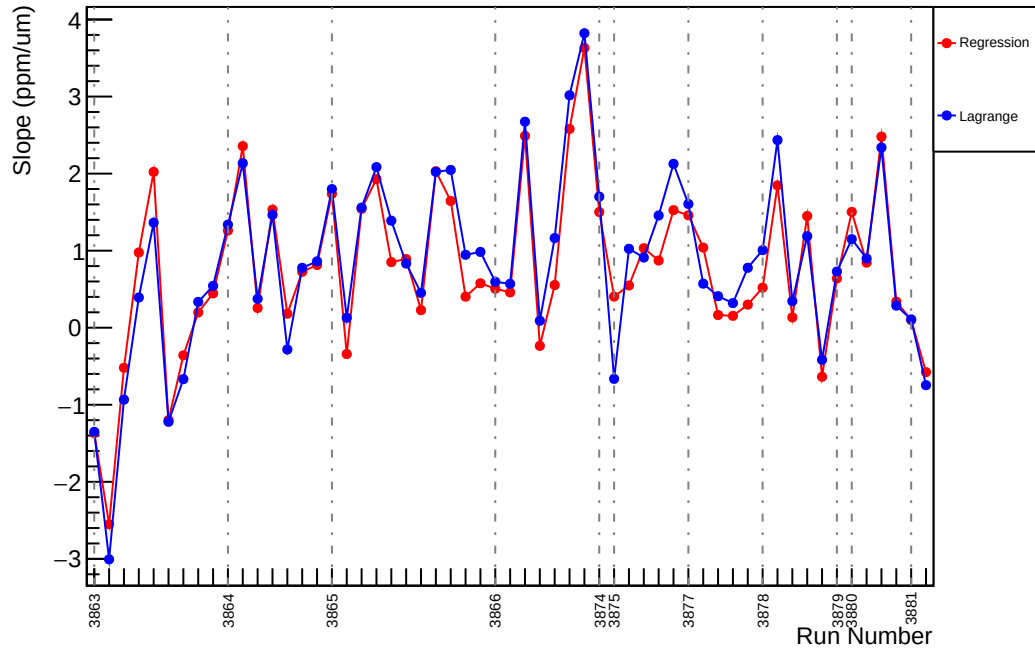
Slug30: Slope : us_avg_vs_evMon5 (ppm/um)
