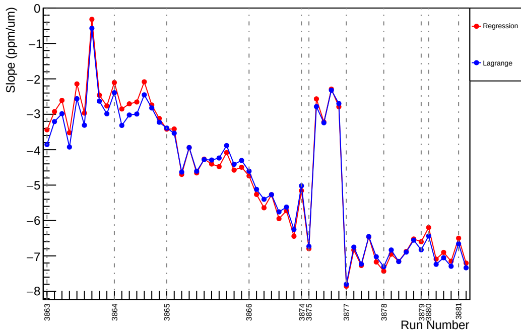
Slug30: Slope : us_avg_vs_evMon0 (ppm/um)
