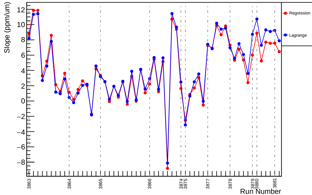
Slug30: Slope : us_avg_vs_evMon7 (ppm/um)
