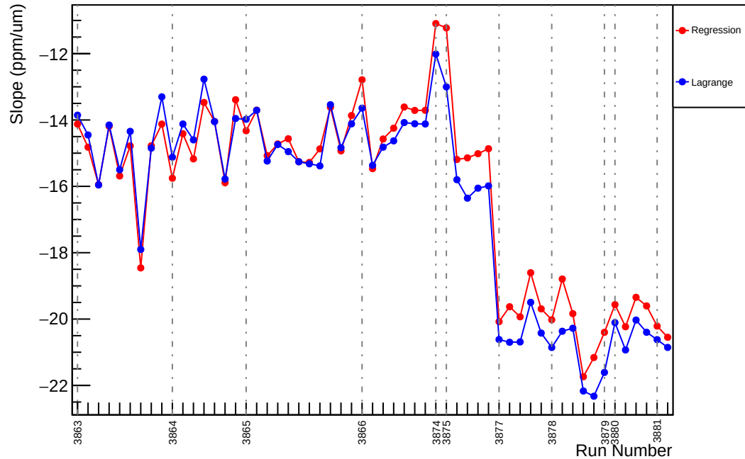
Slug30: Slope : us_avg_vs_evMon4 (ppm/um)
