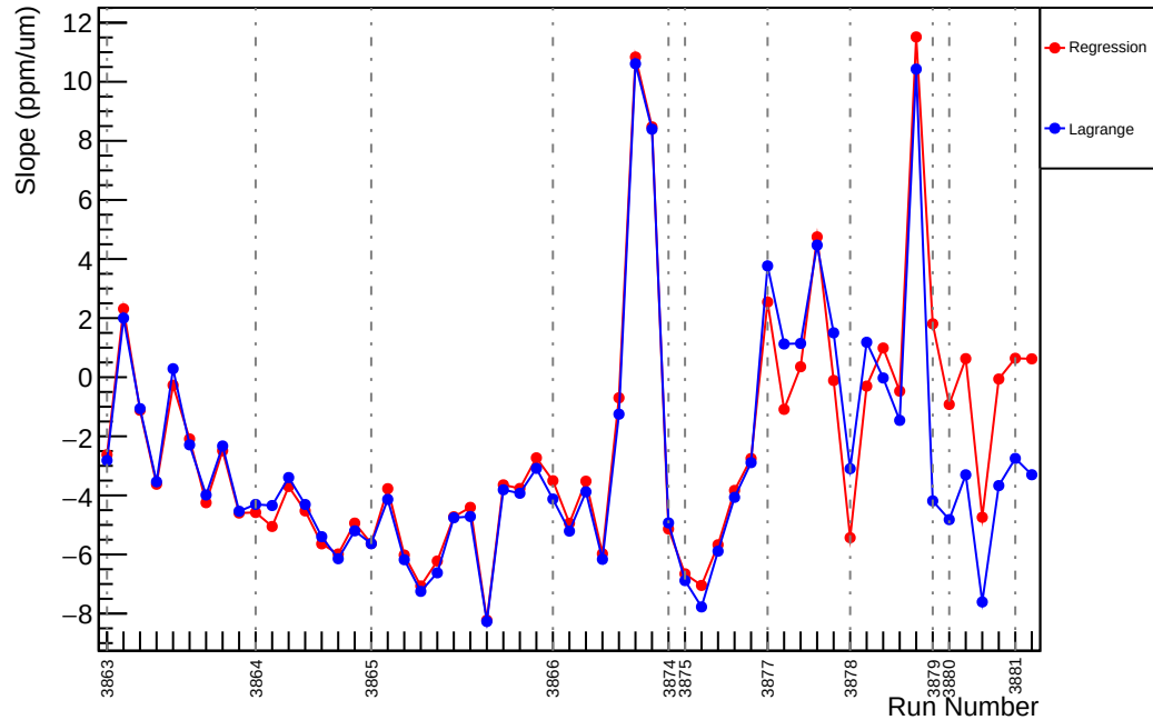
Slug30: Slope : us_avg_vs_evMon8 (ppm/um)
