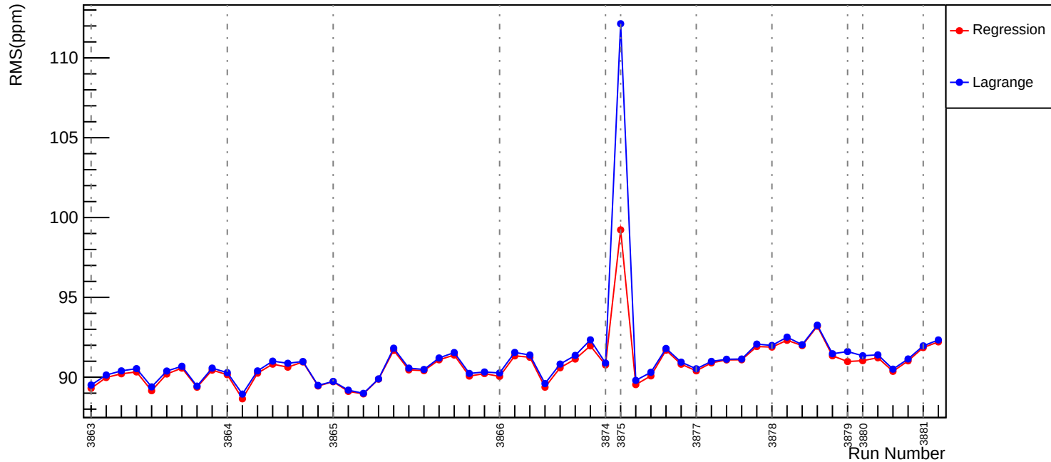
Slug30: Corrected RMS (ppm): asym_us_avg
