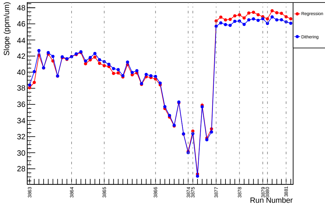
Slug30: Slope : us_dd_vs_evMon0 (ppm/um)
