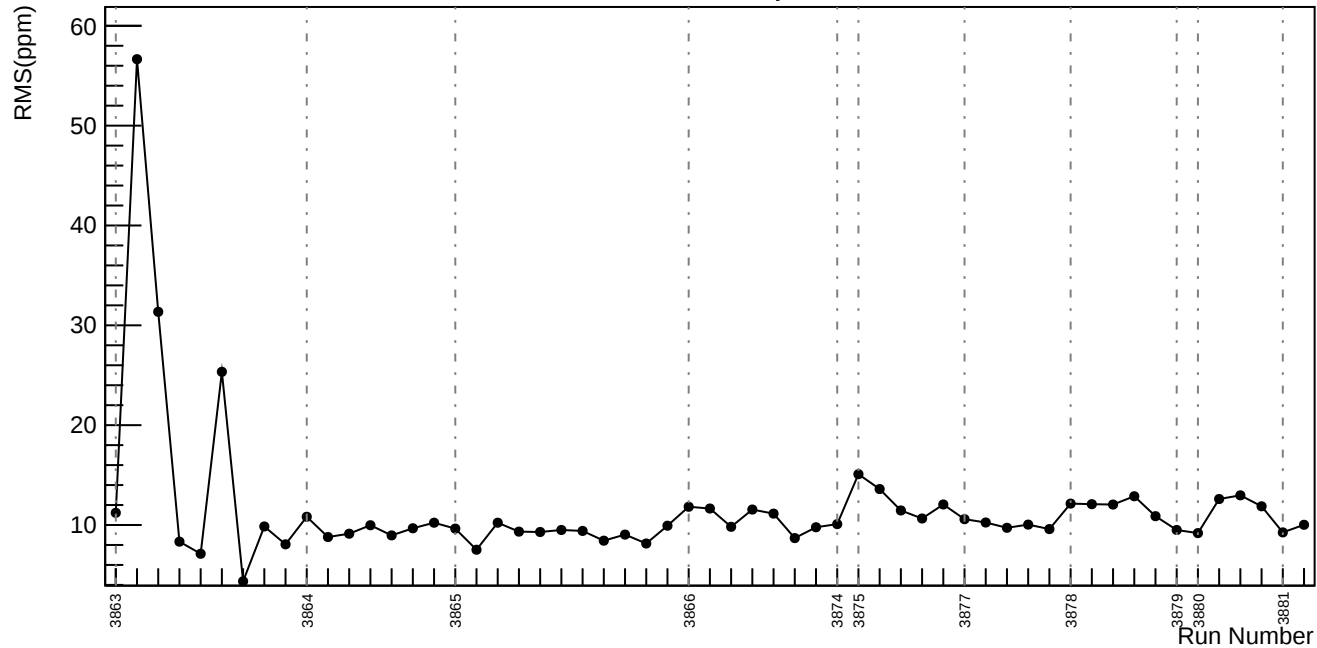
Slug30: asym_us_dd: \sqrt{\sigma_{\text{dit}}^2 - \sigma_{\text{reg}}^2} (ppm)
