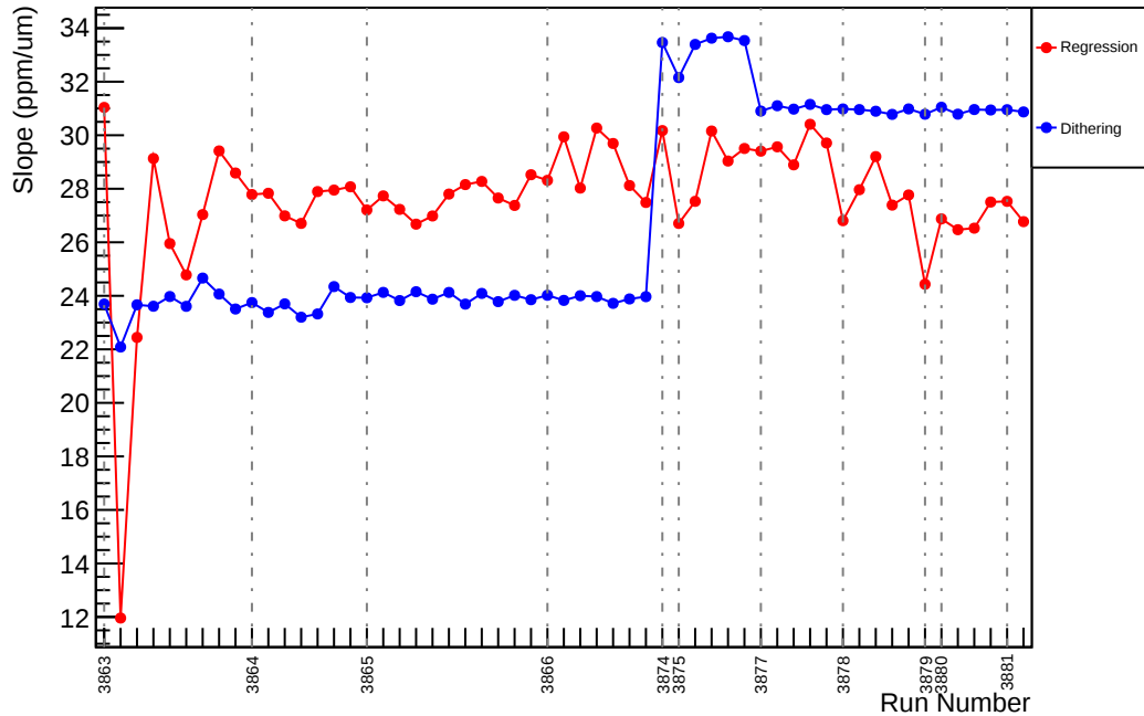
Slug30: Slope : us_dd_vs_evMon3 (ppm/um)
