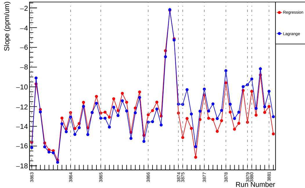
Slug30: Slope : us_dd_vs_evMon7 (ppm/um)
