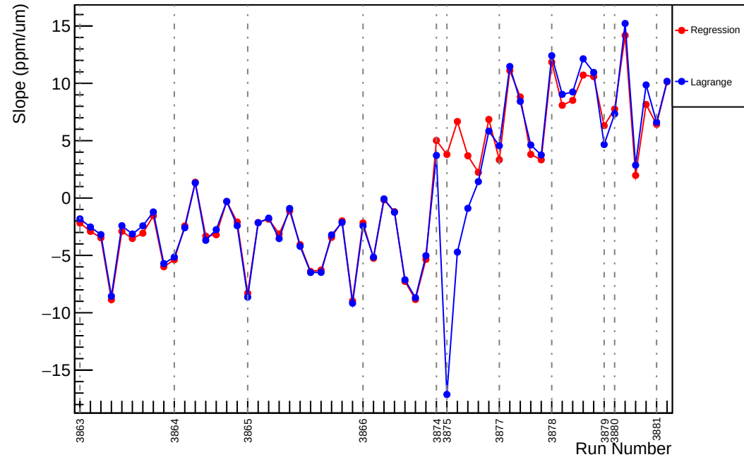
Slug30: Slope : us_dd_vs_evMon11 (ppm/um)
