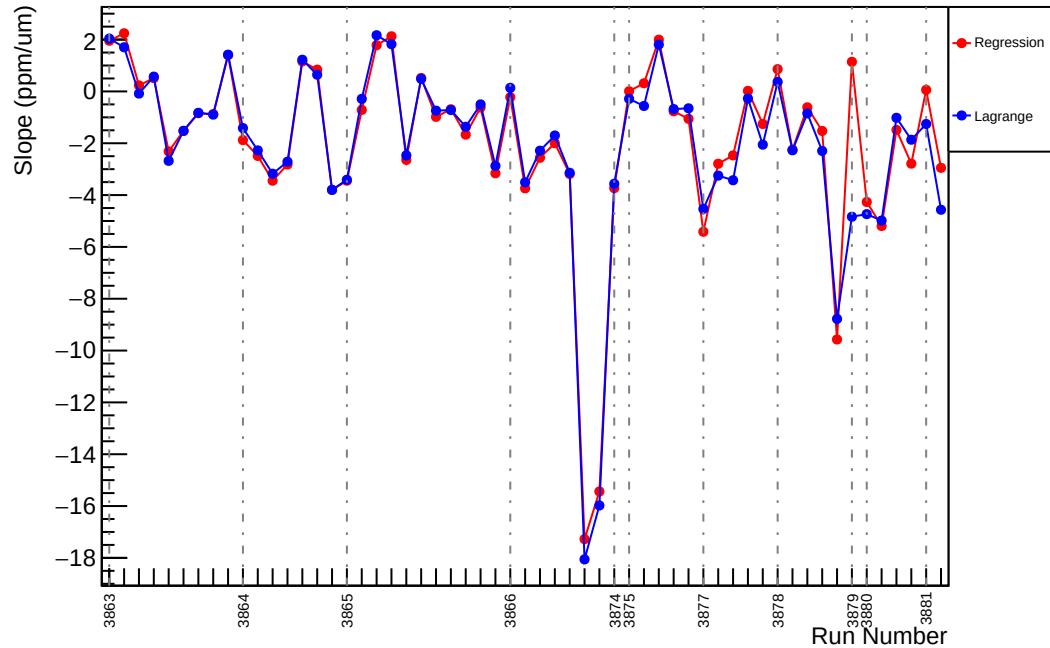
Slug30: Slope : us_dd_vs_evMon8 (ppm/um)
