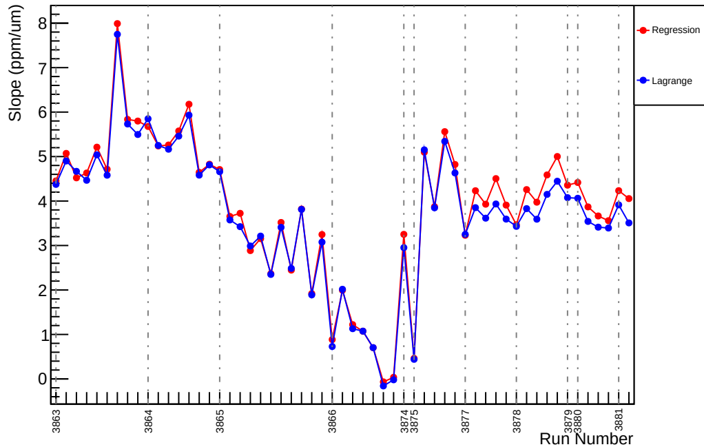
Slug30: Slope : us_dd_vs_evMon2 (ppm/um)
