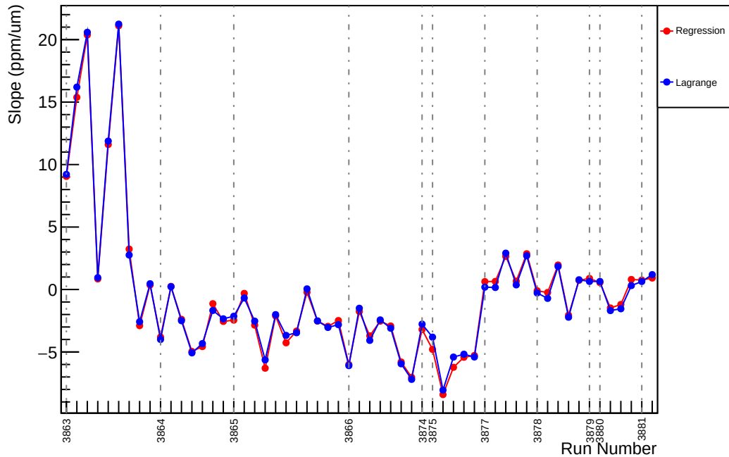
Slug30: Slope : us_dd_vs_evMon6 (ppm/um)
