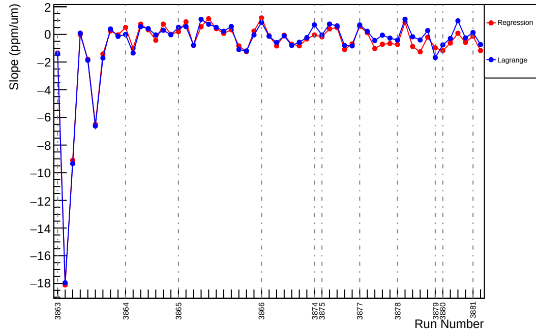
Slug30: Slope : us_dd_vs_evMon5 (ppm/um)
