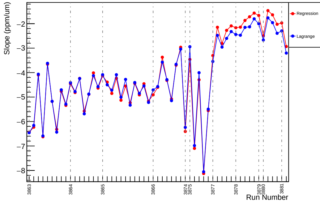
Slug30: Slope : us_dd_vs_evMon1 (ppm/um)
