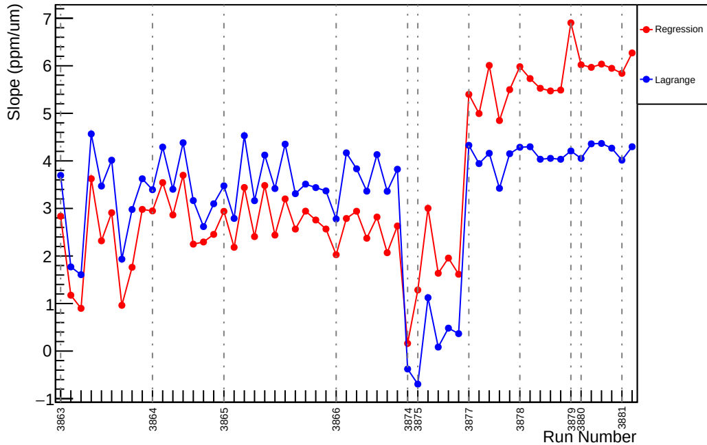
Slug30: Slope : us_dd_vs_evMon4 (ppm/um)
