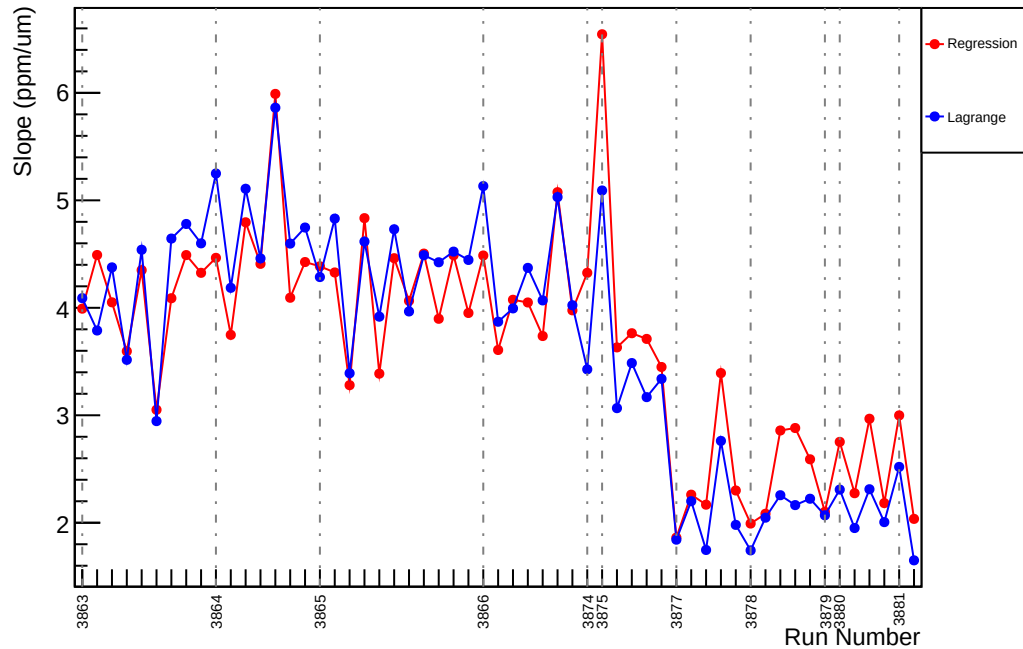
Slug30: Slope : us_dd_vs_evMon3 (ppm/um)
