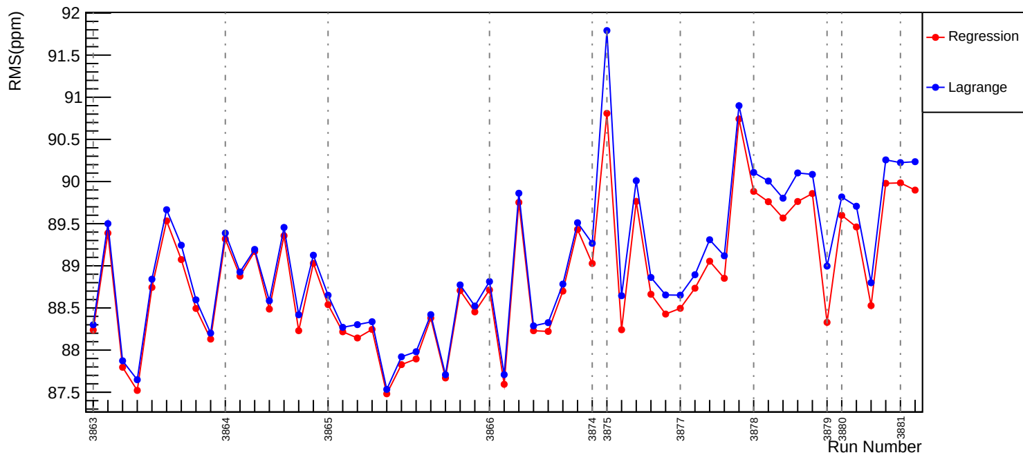
Slug30: Corrected RMS (ppm): asym_us_dd
