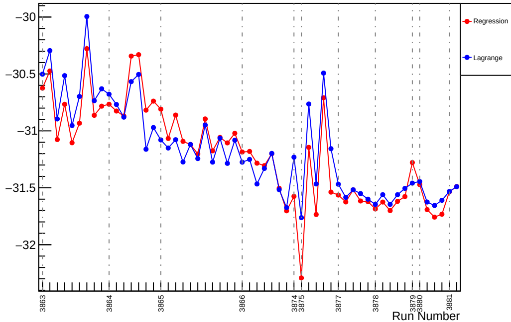
Slug30: Slope : us_dd_vs_evMon0 (ppm/um)
