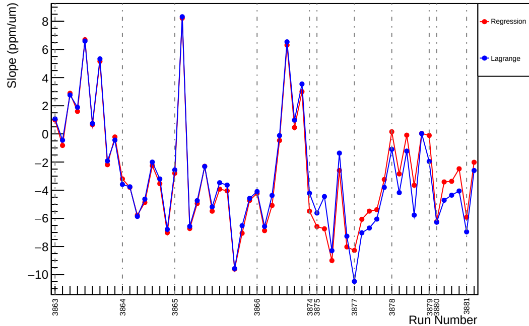
Slug30: Slope : us_dd_vs_evMon10 (ppm/um)
