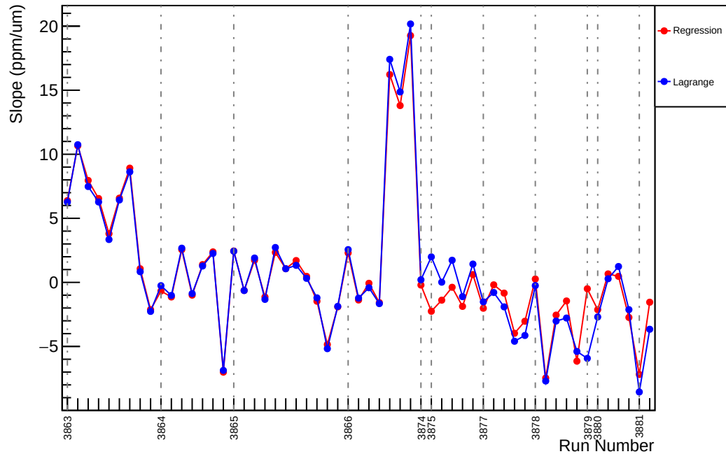
Slug30: Slope : us_dd_vs_evMon9 (ppm/um)
