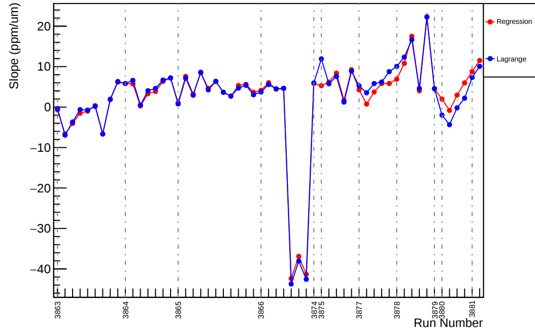
Slug30: Slope : usr_vs_evMon9 (ppm/um)
