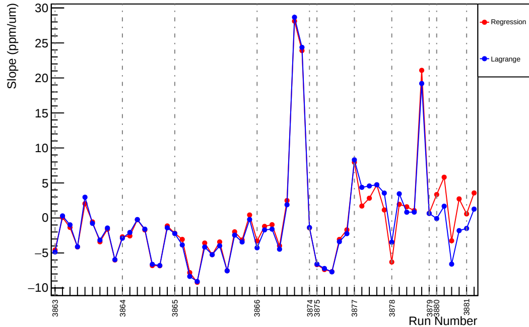
Slug30: Slope : usr_vs_evMon8 (ppm/um)
