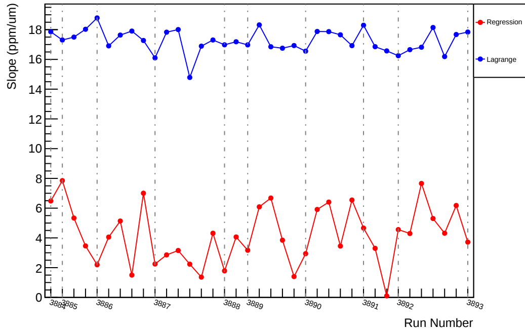
Slug31: Slope : usl_vs_evMon4 (ppm/um)
