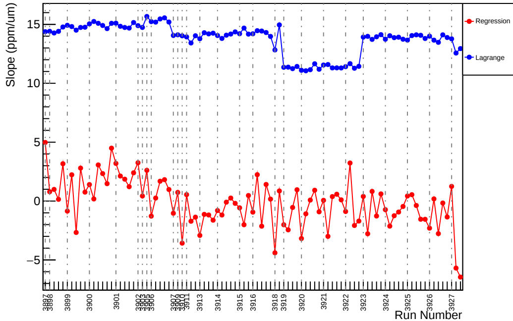
Slug32: Slope : us_avg_vs_evMon4 (ppm/um)
