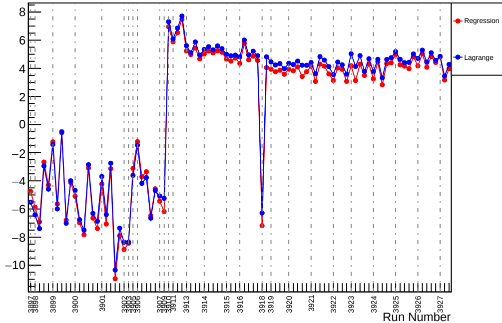
Slug32: Slope : us_avg_vs_evMon1 (ppm/um)
