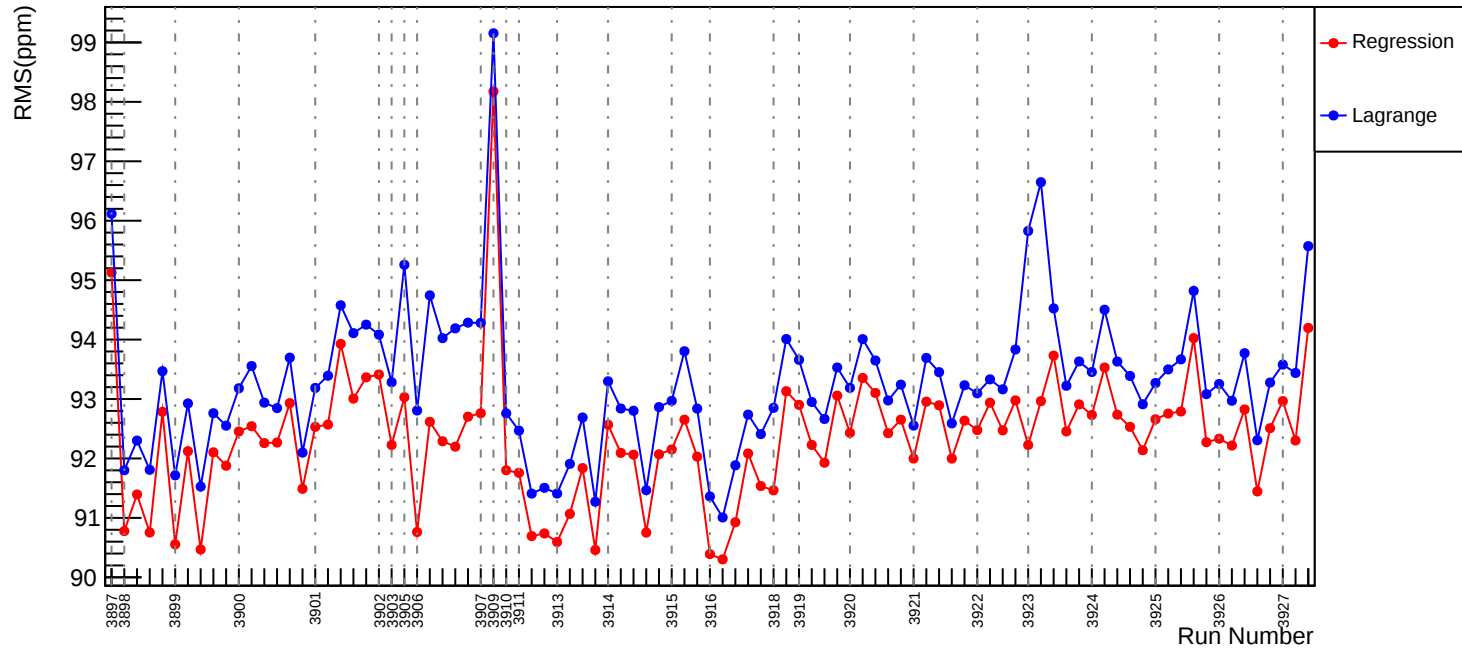
Slug32: Corrected RMS (ppm): asym_us_avg
