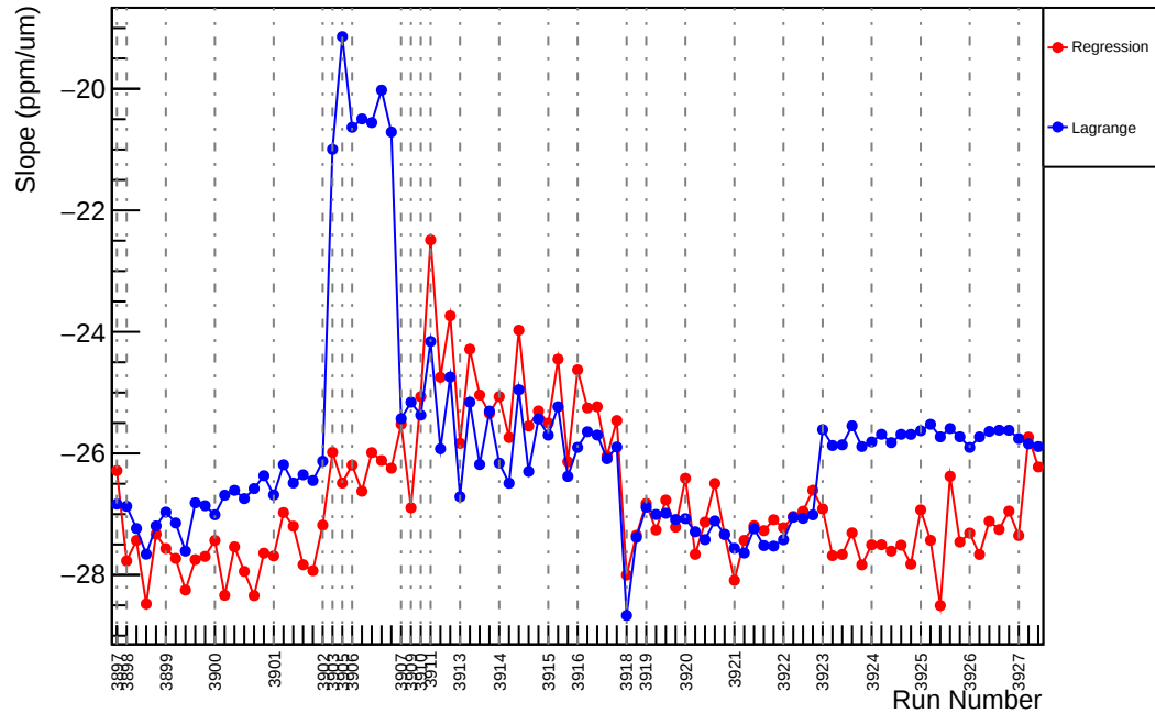
Slug32: Slope : us_avg_vs_evMon3 (ppm/um)
