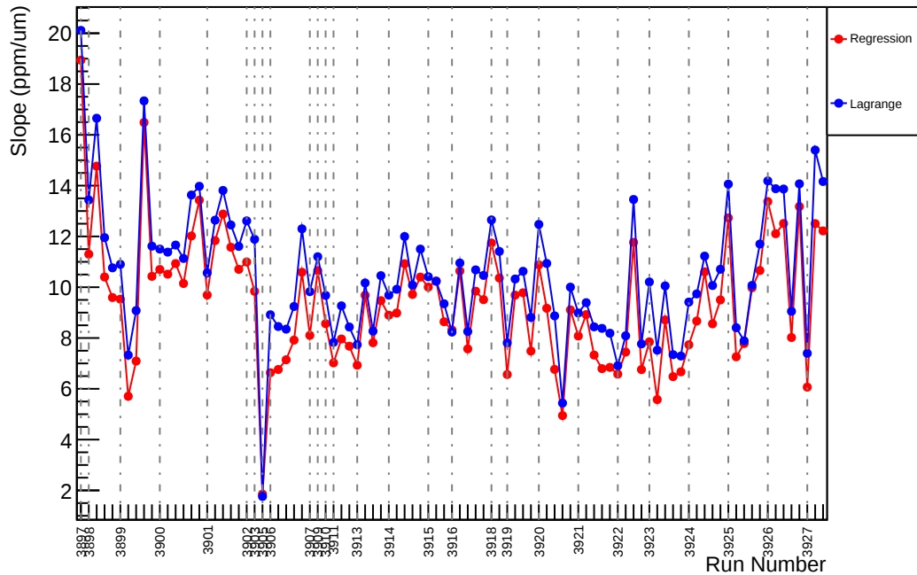
Slug32: Slope : us_avg_vs_evMon5 (ppm/um)
