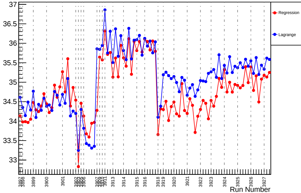
Slug32: Slope : us_avg_vs_evMon2 (ppm/um)
