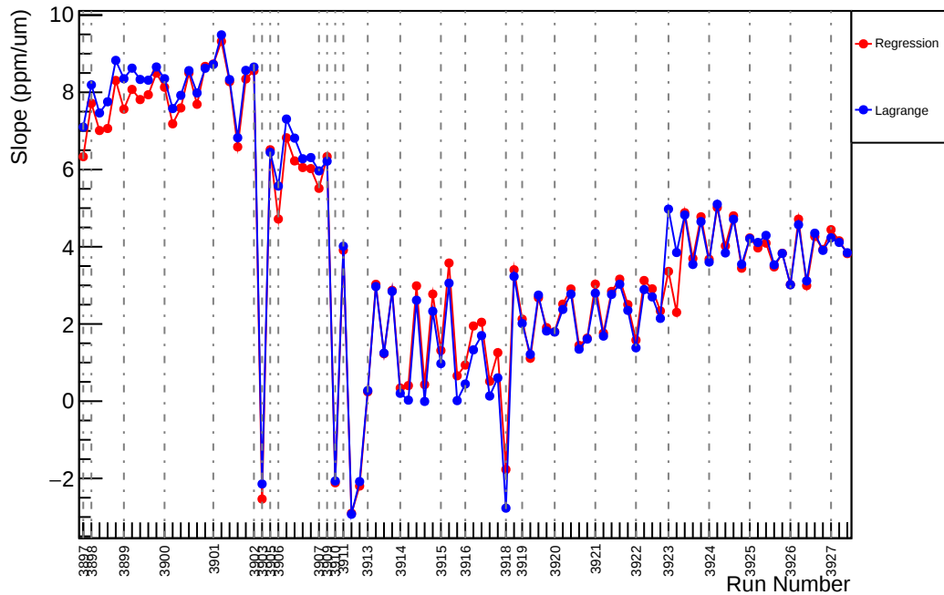
Slug32: Slope : us_avg_vs_evMon0 (ppm/um)
