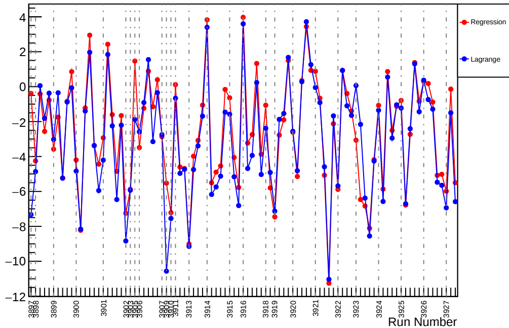
Slug32: Slope : us_avg_vs_evMon11 (ppm/um)
