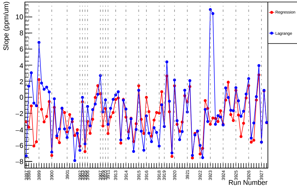
Slug32: Slope : us_avg_vs_evMon9 (ppm/um)
