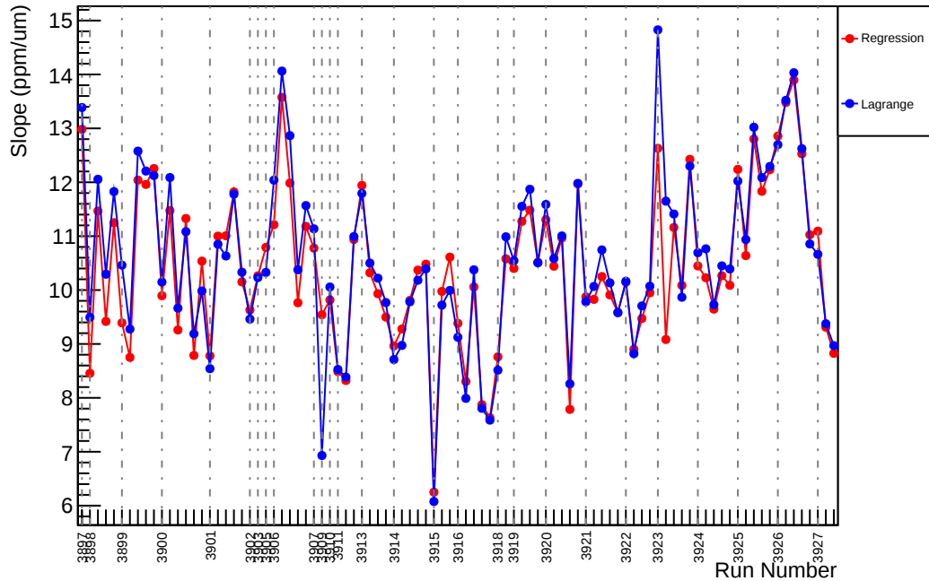
Slug32: Slope : us_avg_vs_evMon6 (ppm/um)
