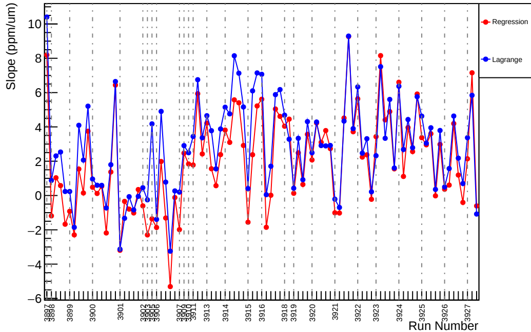
Slug32: Slope : us_avg_vs_evMon10 (ppm/um)
