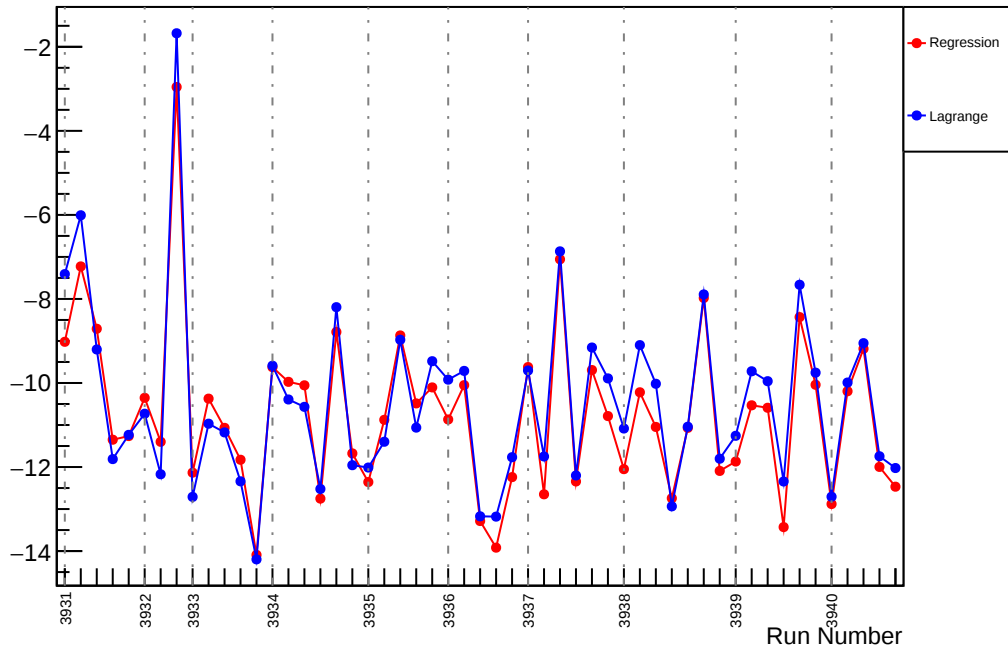
Slug33: Slope : us_dd_vs_evMon7 (ppm/um)
