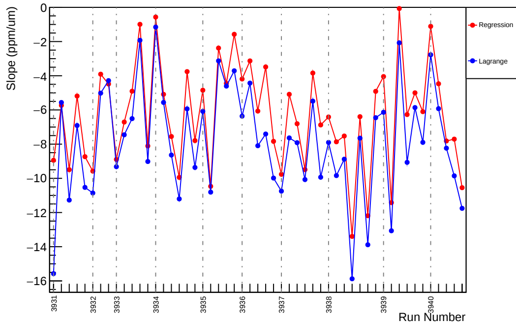
Slug33: Slope : us_dd_vs_evMon10 (ppm/um)
