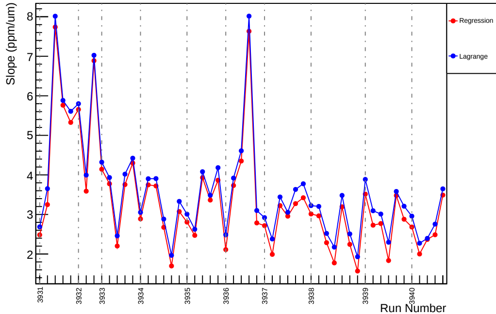
Slug33: Slope : us_dd_vs_evMon1 (ppm/um)
