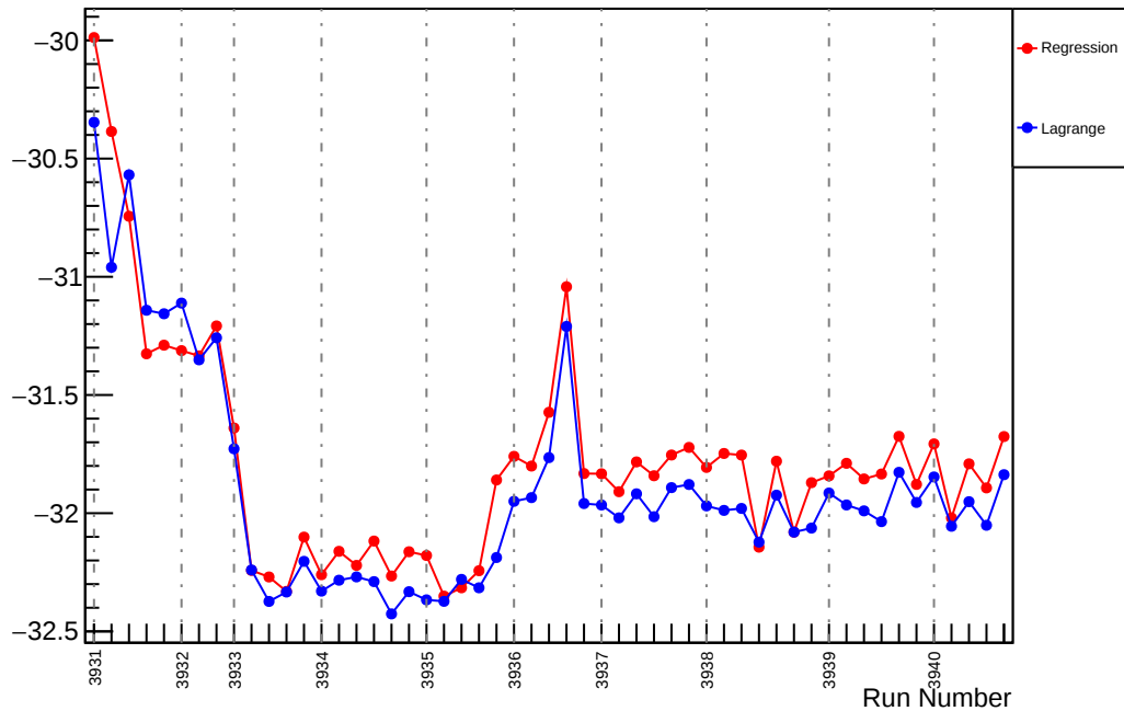
Slug33: Slope : us_dd_vs_evMon0 (ppm/um)
