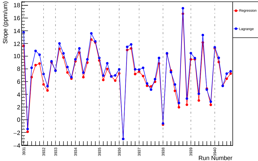
Slug33: Slope : us_dd_vs_evMon11 (ppm/um)
