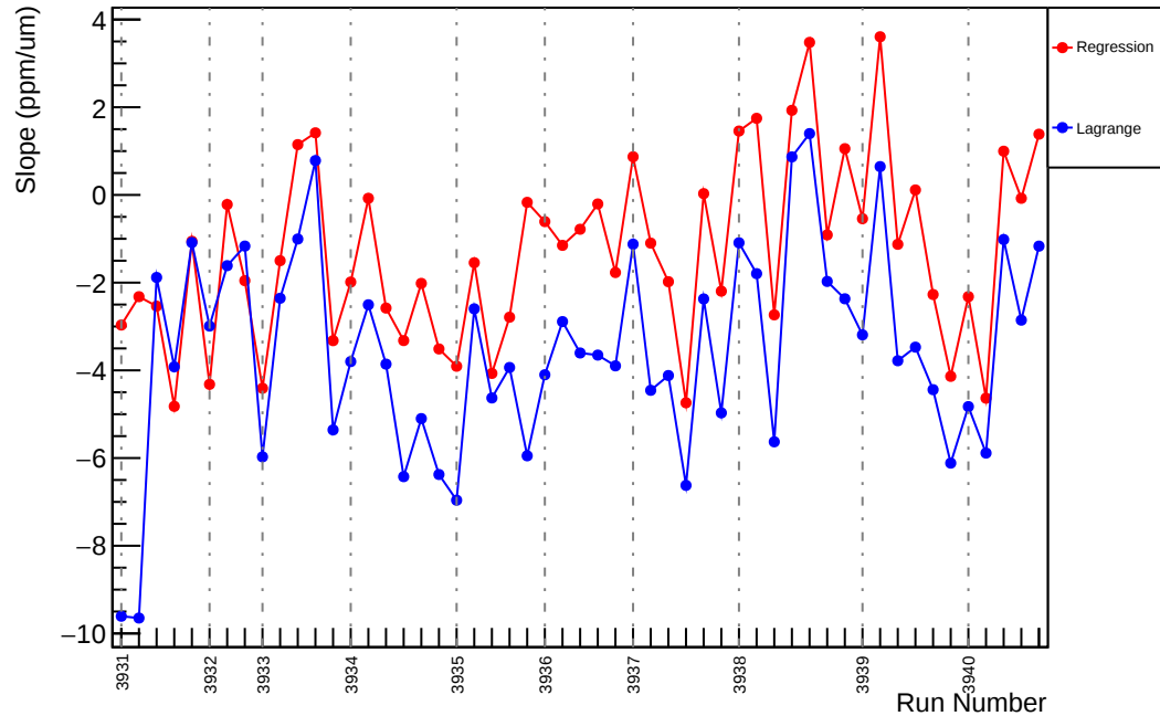
Slug33: Slope : us_dd_vs_evMon8 (ppm/um)
