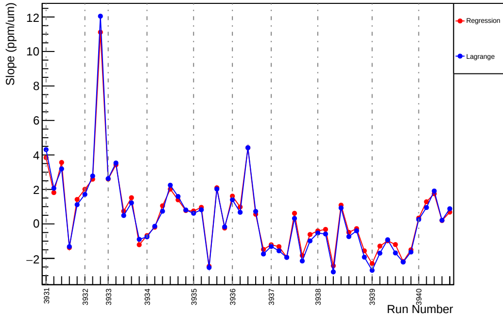
Slug33: Slope : us_dd_vs_evMon6 (ppm/um)
