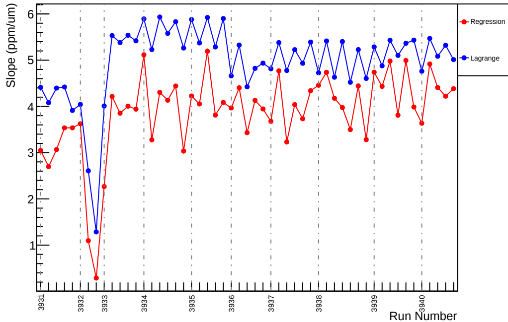
Slug33: Slope : us_dd_vs_evMon4 (ppm/um)
