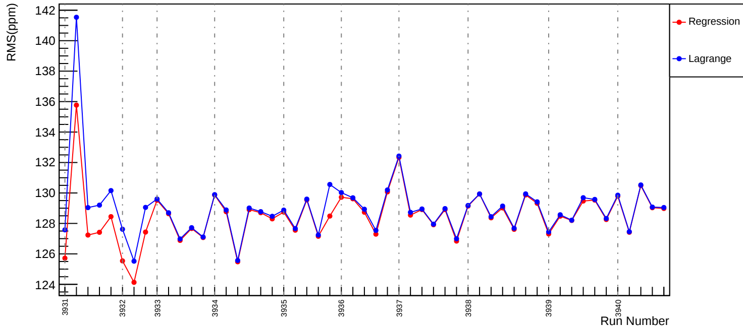
Slug33: Corrected RMS (ppm): asym_usr
