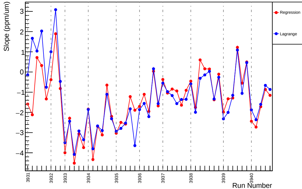
Slug33: Slope : usr_vs_evMon5 (ppm/um)
