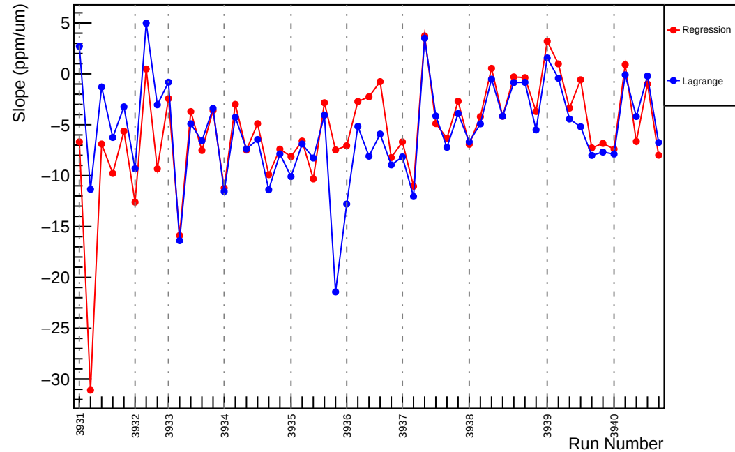
Slug33: Slope : usr_vs_evMon9 (ppm/um)
