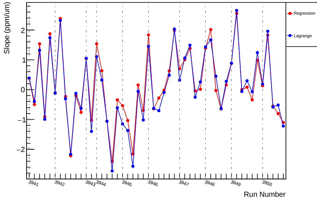
Slug34: Slope : us_dd_vs_evMon6 (ppm/um)
