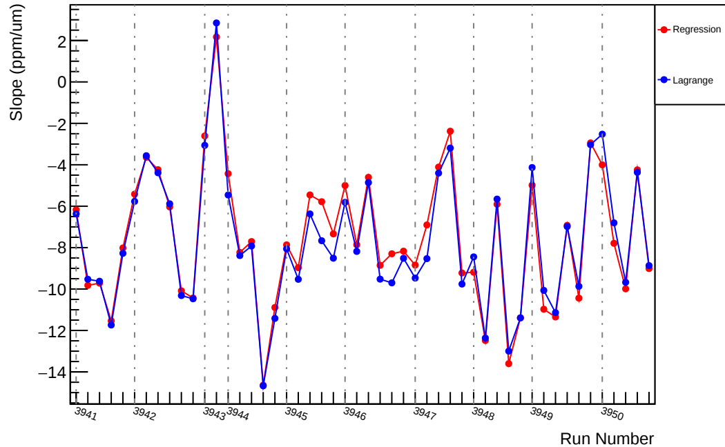
Slug34: Slope : us_dd_vs_evMon11 (ppm/um)
