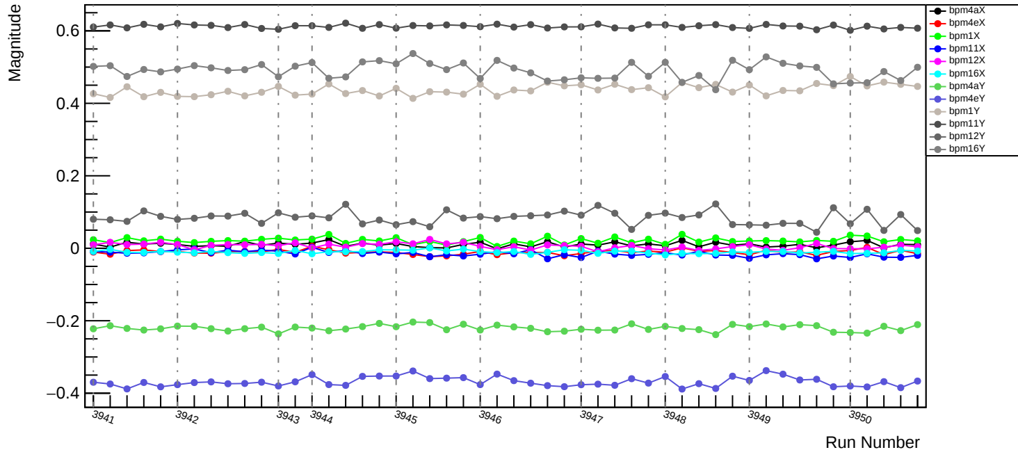
Slug34: EigenVector #5
