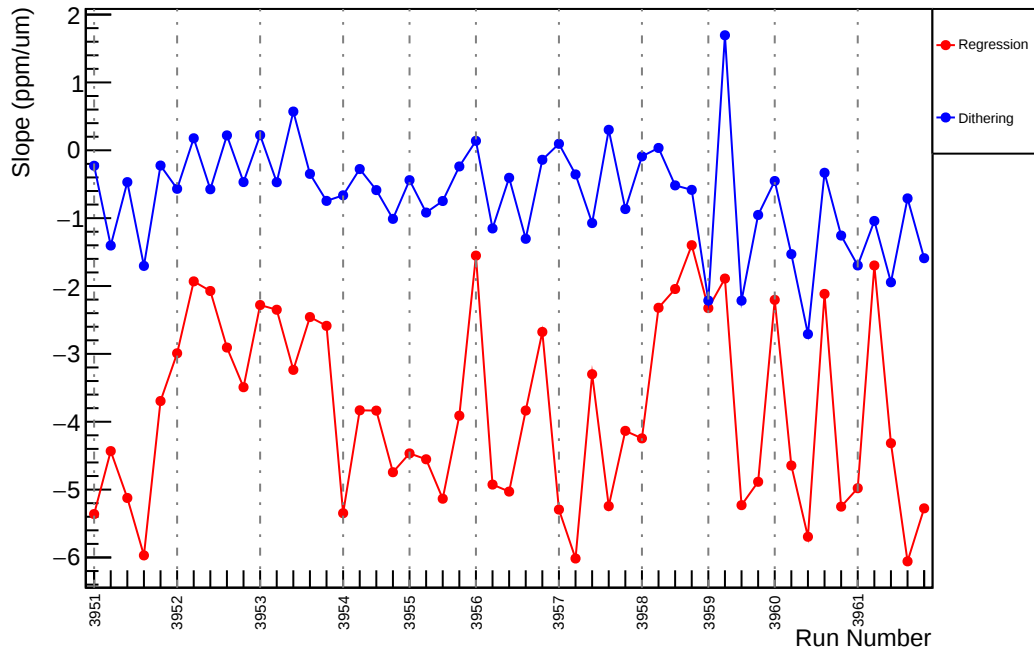
Slug35: Slope : us_dd_vs_evMon4 (ppm/um)
