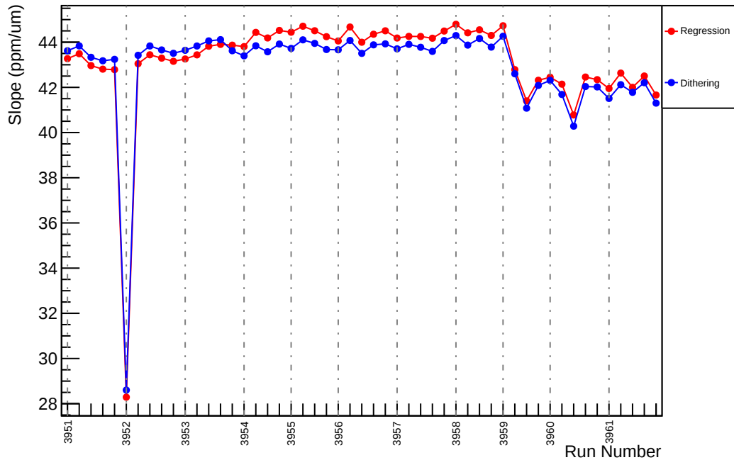
Slug35: Slope : us_dd_vs_evMon0 (ppm/um)
