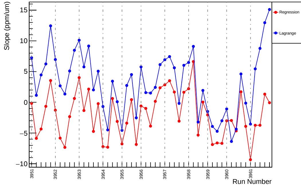
Slug35: Slope : usl_vs_evMon9 (ppm/um)
