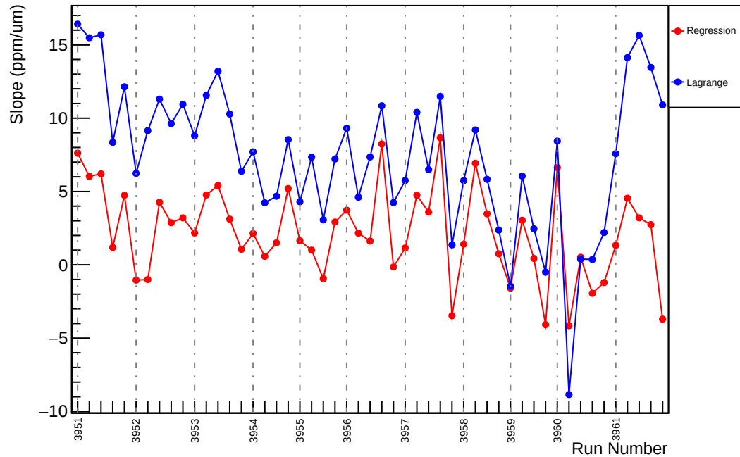
Slug35: Slope : usl_vs_evMon8 (ppm/um)
