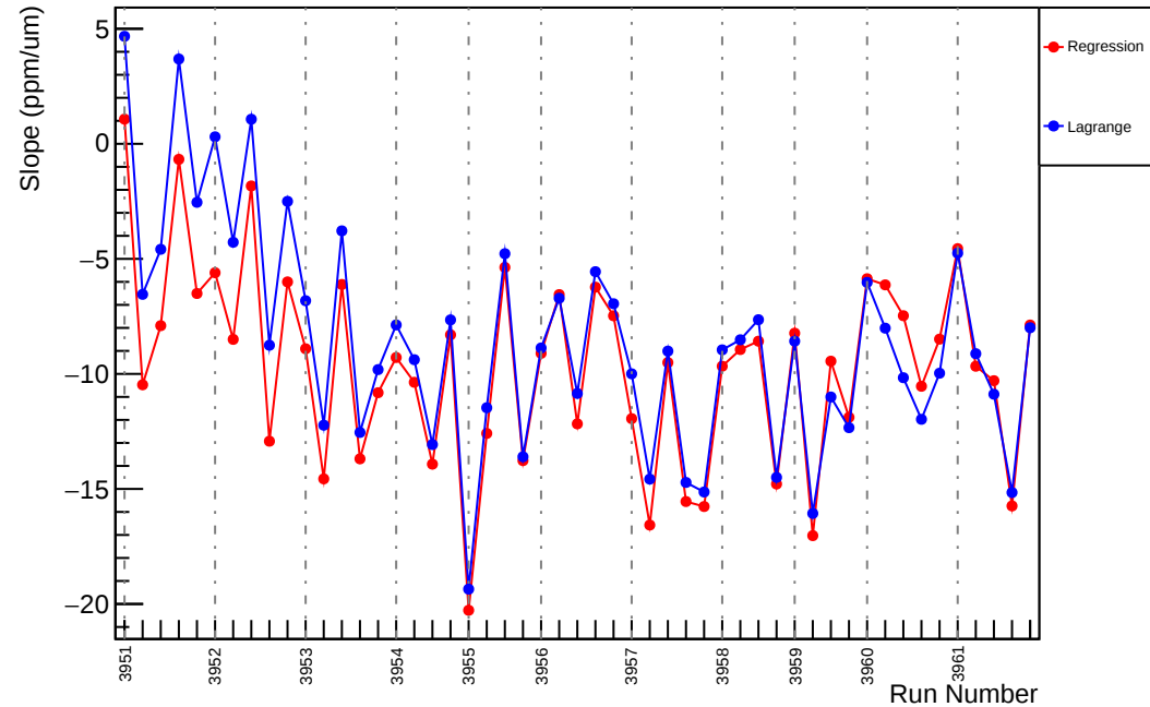
Slug35: Slope : usl_vs_evMon11 (ppm/um)
