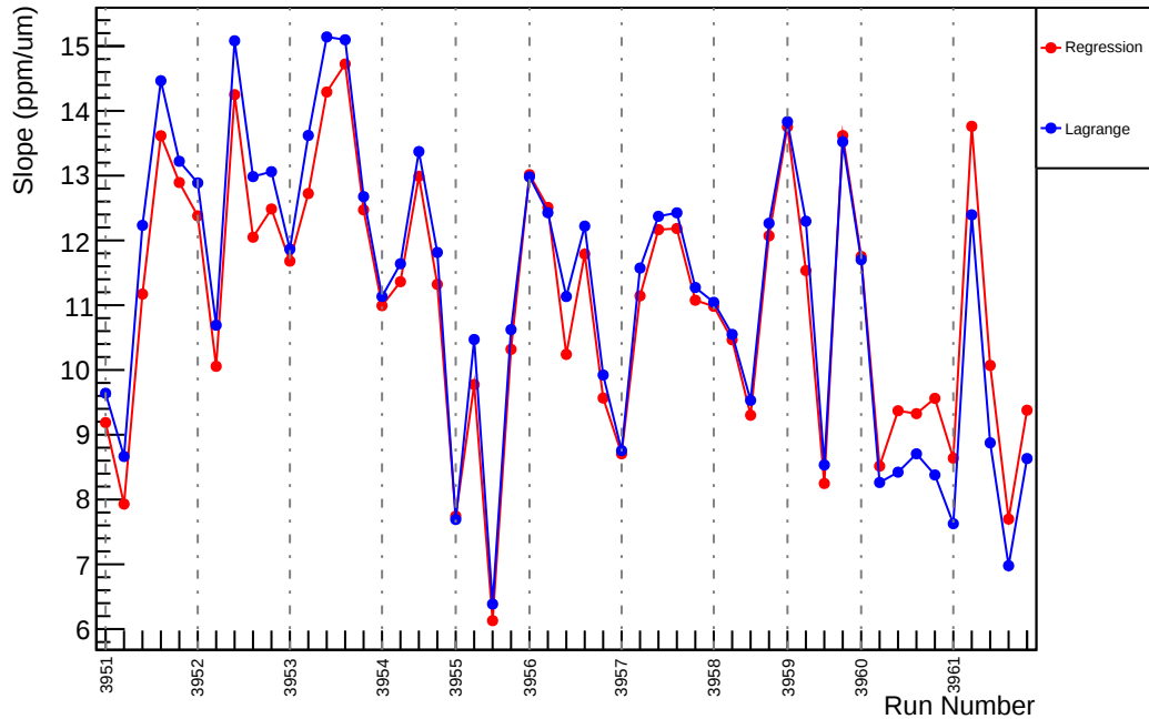
Slug35: Slope : usl_vs_evMon6 (ppm/um)
