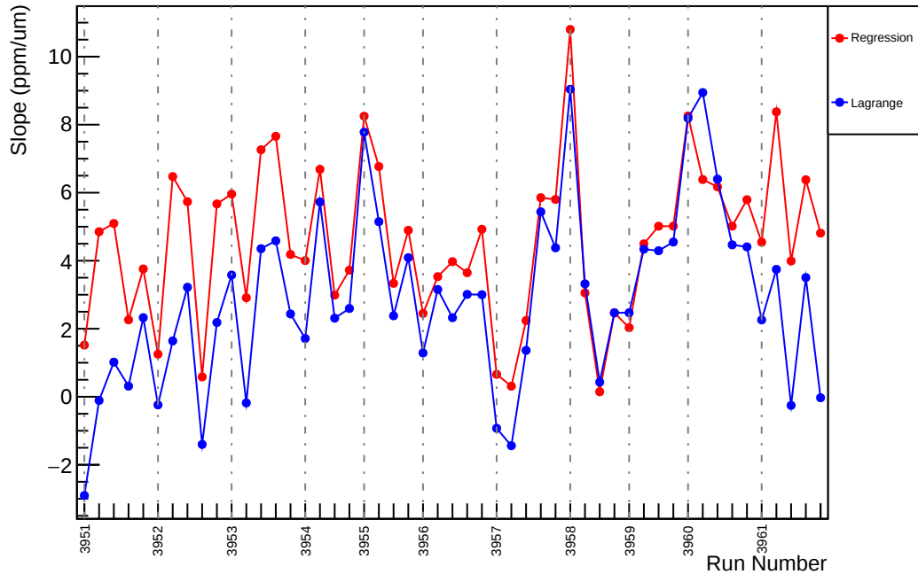
Slug35: Slope : usl_vs_evMon7 (ppm/um)
