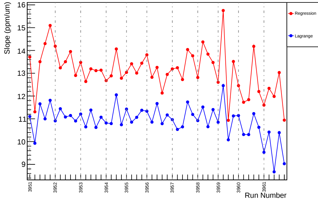
Slug35: Slope : usl_vs_evMon4 (ppm/um)
