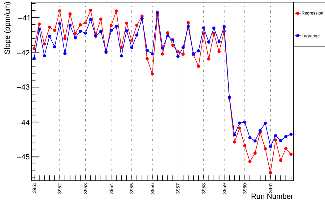
Slug35: Slope : usl_vs_evMon2 (ppm/um)
