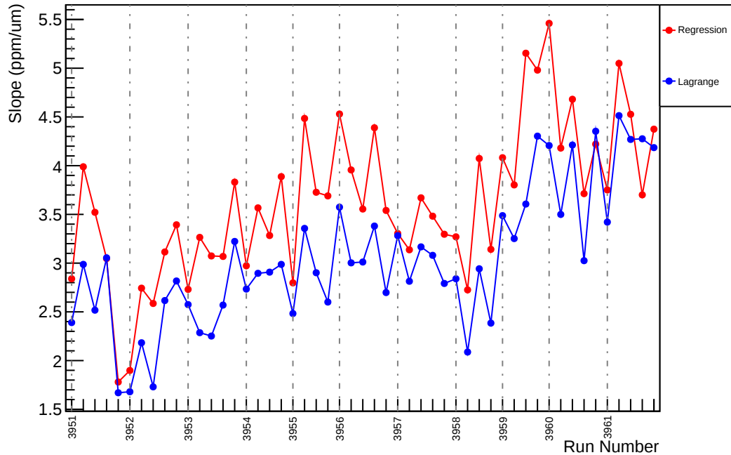
Slug35: Slope : usl_vs_evMon3 (ppm/um)
