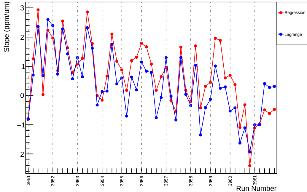
Slug35: Slope : usl_vs_evMon5 (ppm/um)
