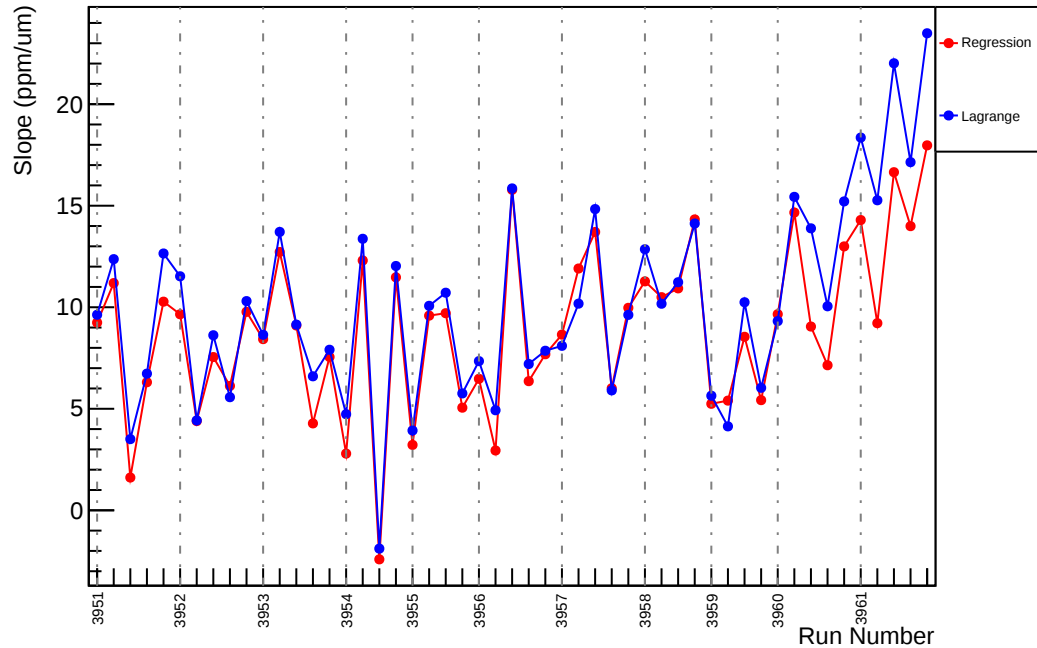
Slug35: Slope : usl_vs_evMon10 (ppm/um)
