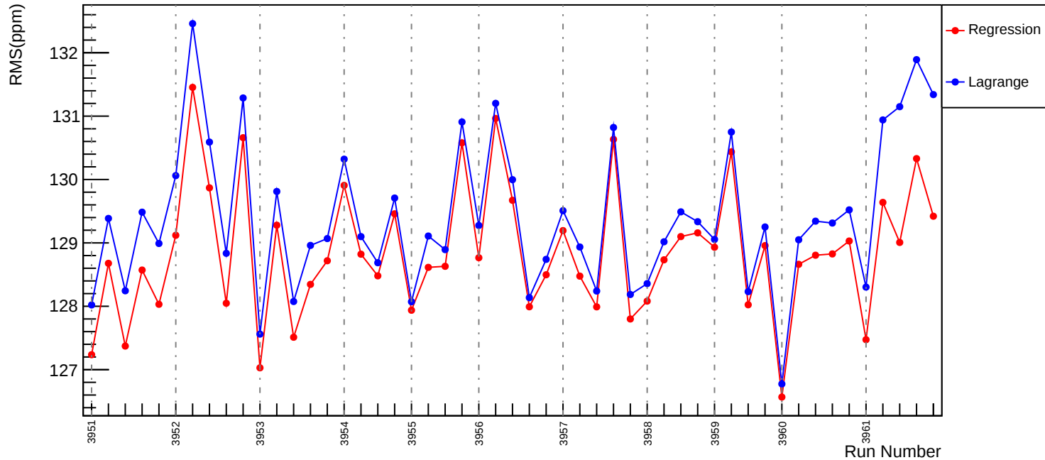
Slug35: Corrected RMS (ppm): asym_usl
