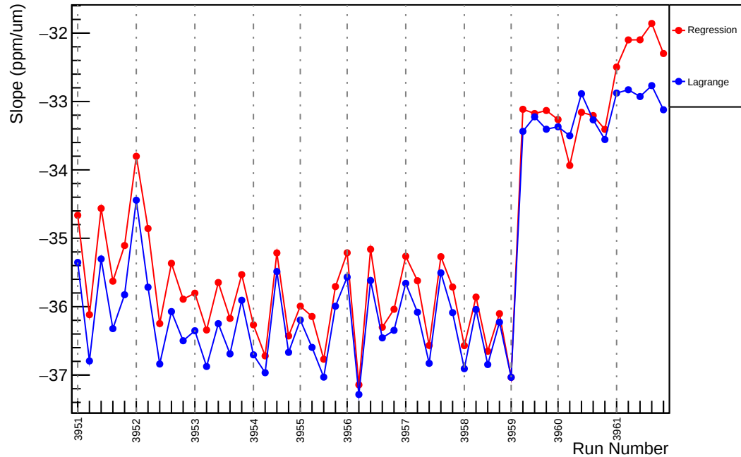
Slug35: Slope : usl_vs_evMon0 (ppm/um)
