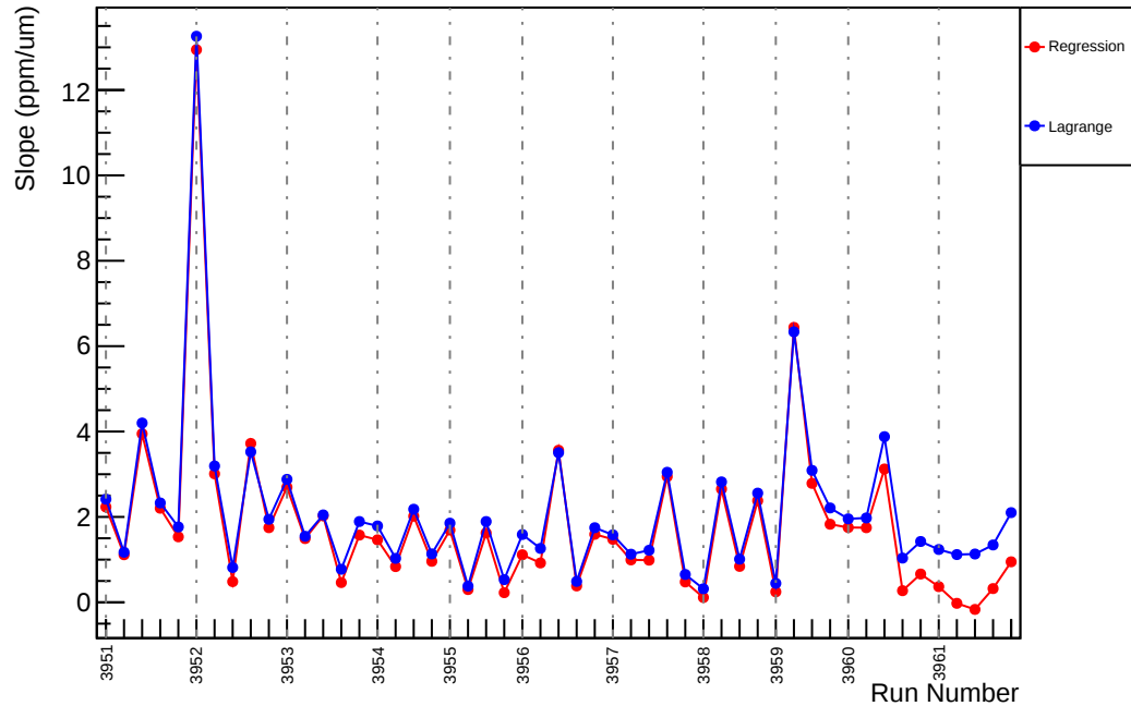
Slug35: Slope : usl_vs_evMon1 (ppm/um)
